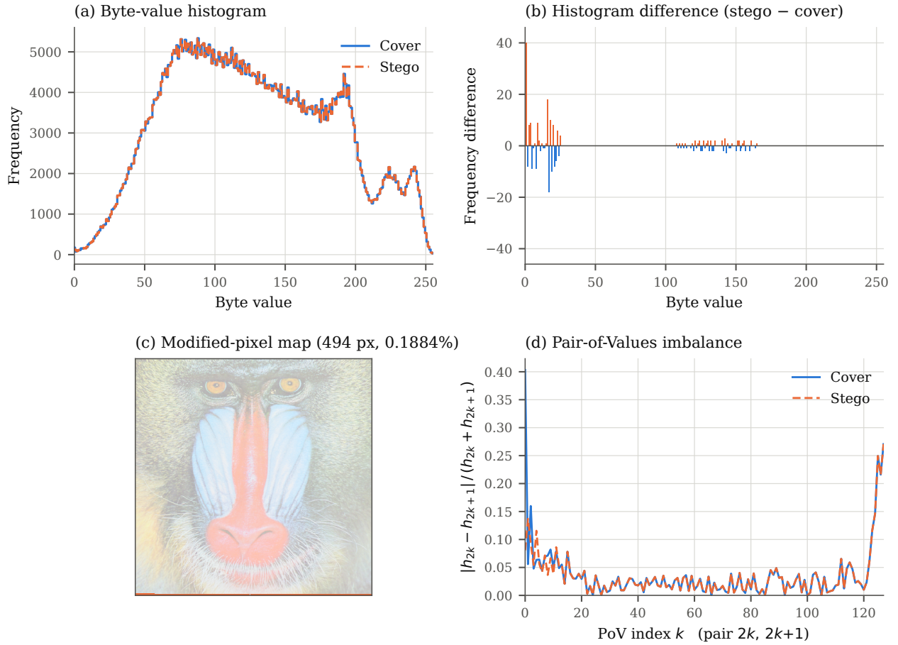
Figure 1. Imperceptibility analysis on the Baboon image (USC-SIPI 4.2.03). (a) Byte-value histograms of cover and stego overlap throughout the range. (b) The signed histogram difference shows that embedding redistributes counts only between adjacent byte values. (c) Spatial distribution of the 494 modified pixels (0.1884% of the image). (d) Pair-of-values imbalance, which the chi-square attack exploits, is essentially unchanged (0.03676 to 0.03437).
