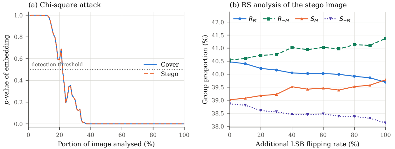
Figure 2. Steganalysis of the proposed scheme on the Baboon image. (a) Chi-square attack: the p -value of the stego image remains indistinguishable from that of the cover across the entire image, indicating that the embedding does not produce the pair-of-values equalisation the attack detects. (b) RS analysis: the R_M and R_{-M} curves differ by 0.071 percentage points at zero additional flipping, consistent with a low embedding rate.
