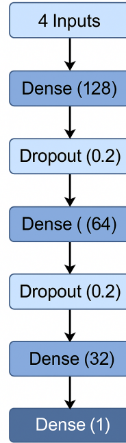
Figure 1. Keras sequential network model.
