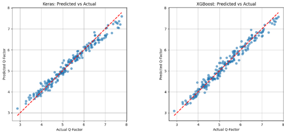
Figure 2. Q-factor scores on test data compared with estimates from both algorithms. The red diagonal ( y = x ) indicates an ideal prediction.
