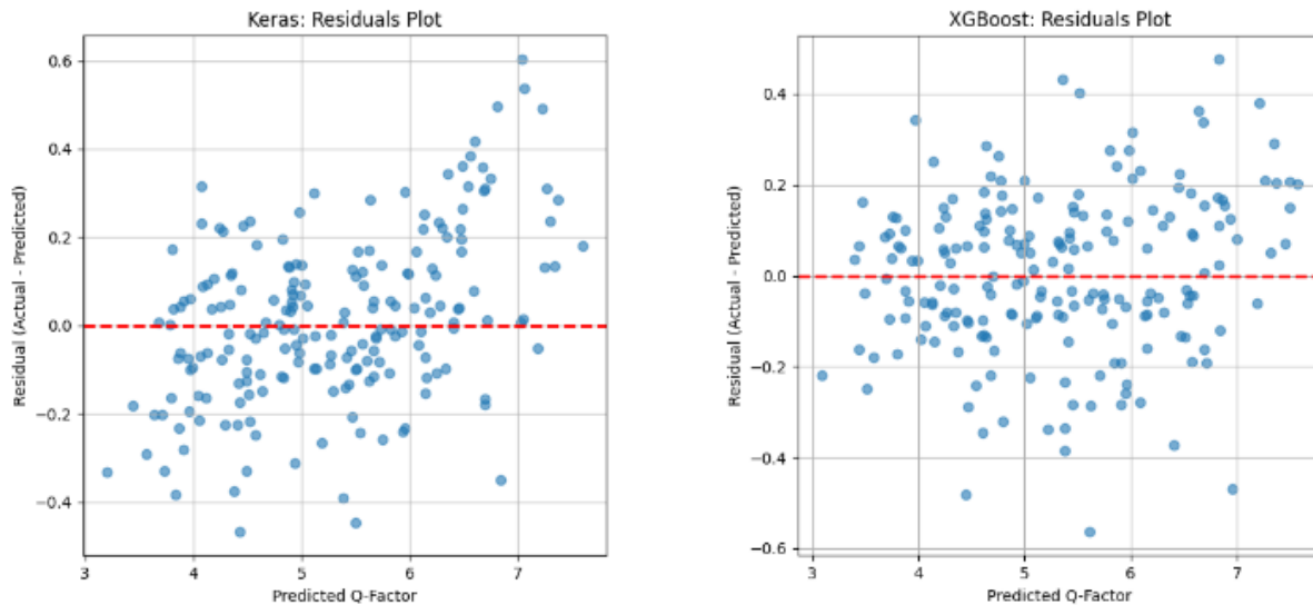
Figure 5. Actual and predicted residual distributions for XGBoost and Keras NN on the test data.
