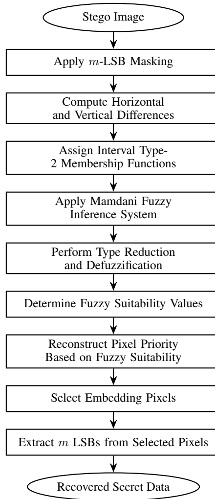
Figure 4. Extraction procedure of the proposed mshEdgeGrayFT2 algorithm.
