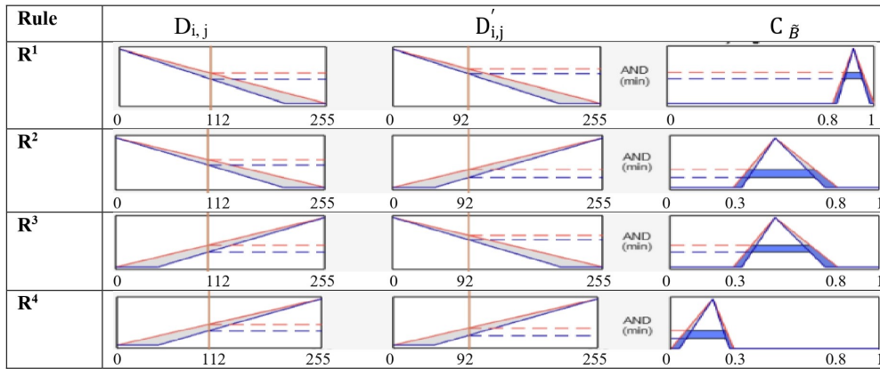
Figure 3. Implication of fuzzy rules
