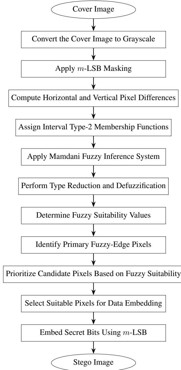
Figure 2. Embedding procedure of the proposed mshEdgeGrayFT2 algorithm.
