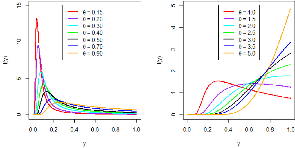
Figure 1. PDFs of the NUH distribution for selected values of the shape parameter \theta .
