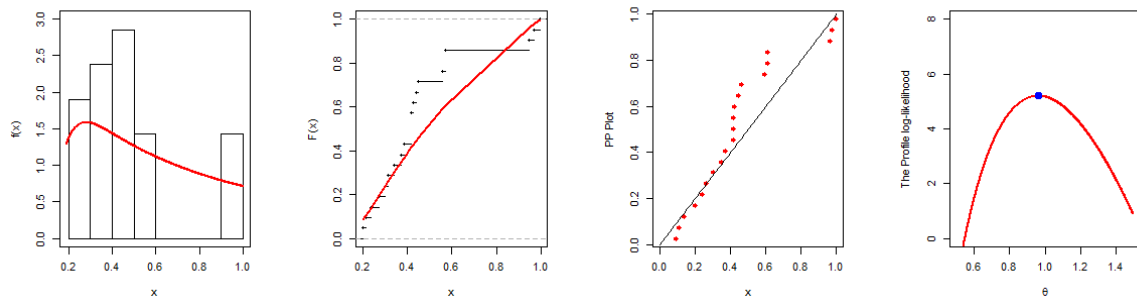
Figure 9. The fitted PDF, CDF, PP, and profile log-likelihood plot for the entomology data.
