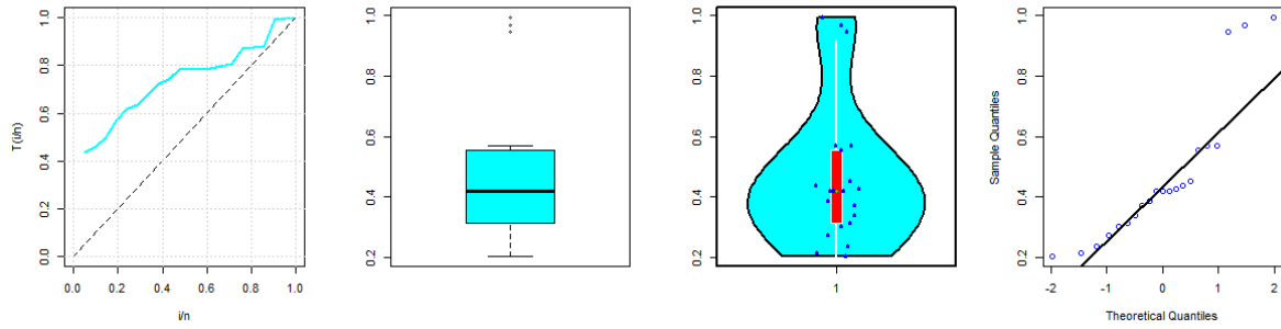
Figure 8. The non-parametric plots based on the entomology data.
