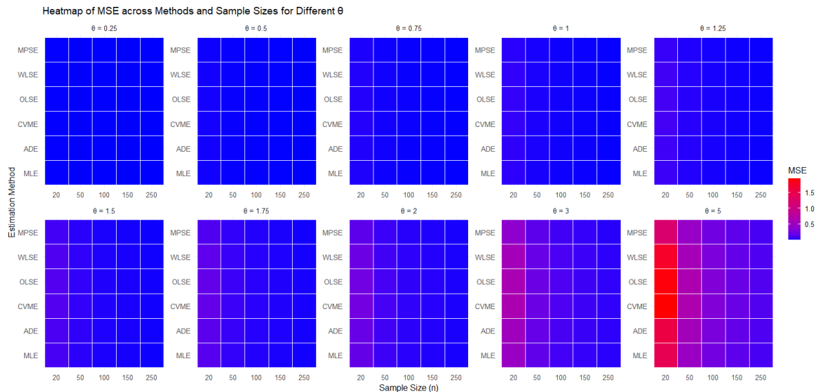
Figure 3. MSE heatmap plots for each choice of parameter \theta .
