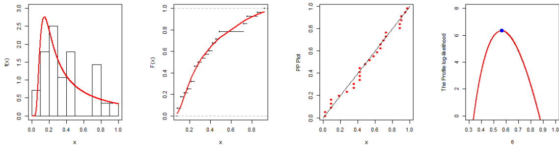
Figure 7. The fitted PDF, CDF, PP, and profile log-likelihood plot for the kidney dialysis data.
