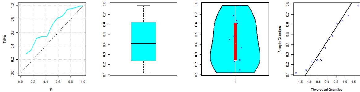
Figure 4. The non-parametric plots based on the COVID-19 data.
