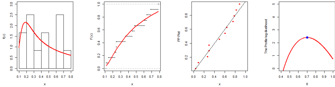
Figure 5. The fitted PDF, CDF, PP, and profile log-likelihood plot for the COVID-19 data.
