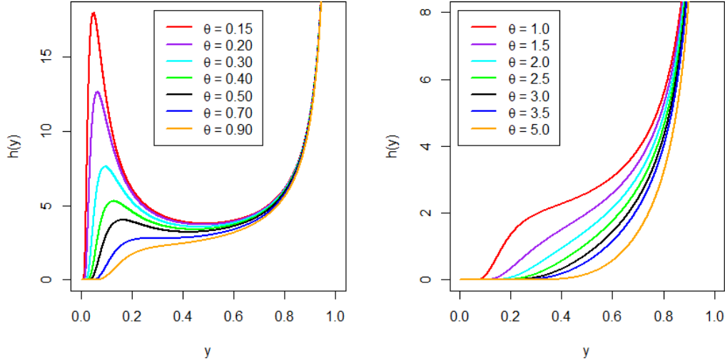
Figure 2. Hazard functions of the NUH distribution for selected values of the shape parameter \theta .
