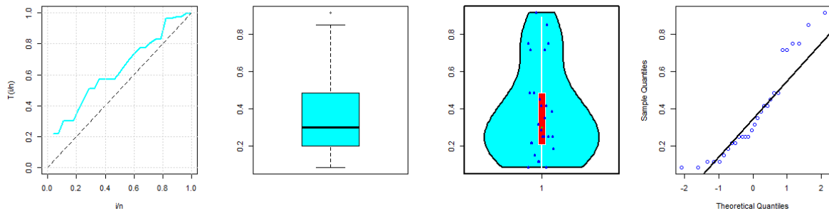
Figure 6. The non-parametric plots based on the kidney dialysis data.
