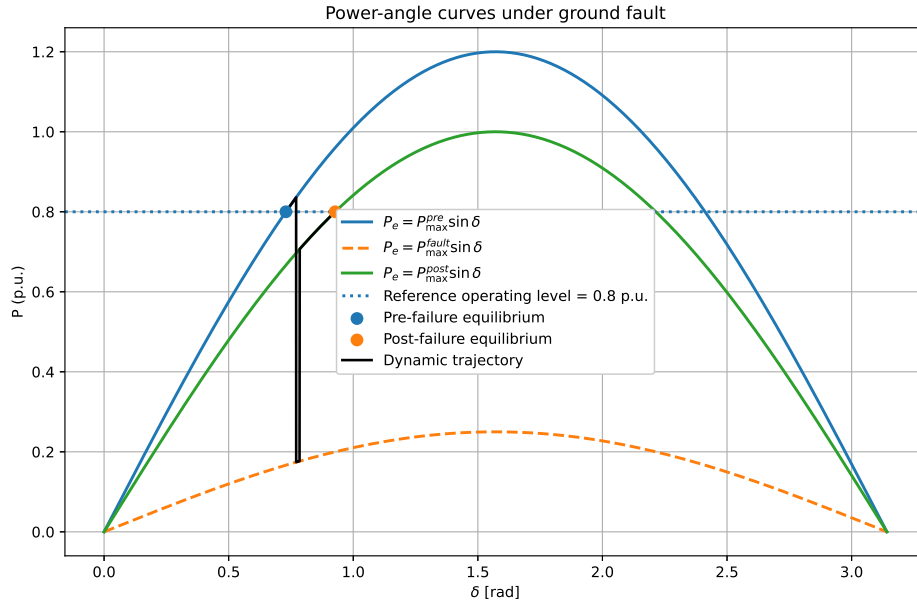
Figure 1. Power vs angle curves before, during, and after the ground fault.
