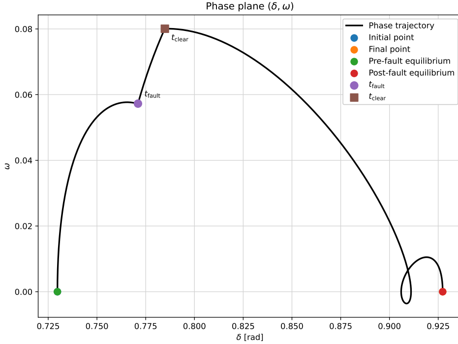
Figure 4. Phase plane (\delta, \omega) showing the system trajectory.
