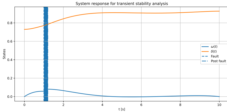
Figure 3. Time response of the state variables for transient-stability analysis.
