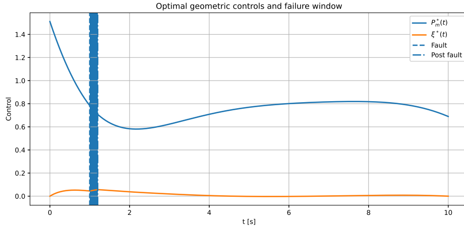
Figure 2. Optimal geometric controls P_m^*(t) and \xi^*(t) , showing the fault inception and clearing times.
