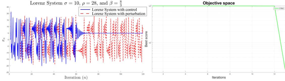
Figure 7. Application of MODPC to system (3) at \sigma = 10 , \rho = 28 , and \beta = \frac{8}{3} : (a) simulation results and (b) MAPE in each iteration.
