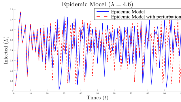
Figure 8. Simulation of system (4) at \lambda = 4.6 .
