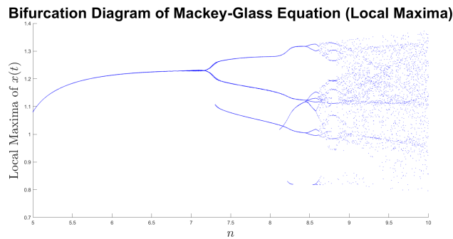
Figure 15. Bifurcation diagram of equation (5).
