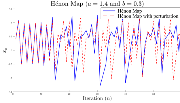
Figure 4. Simulation of system (2) at a = 1.4 and b = 0.3 .
