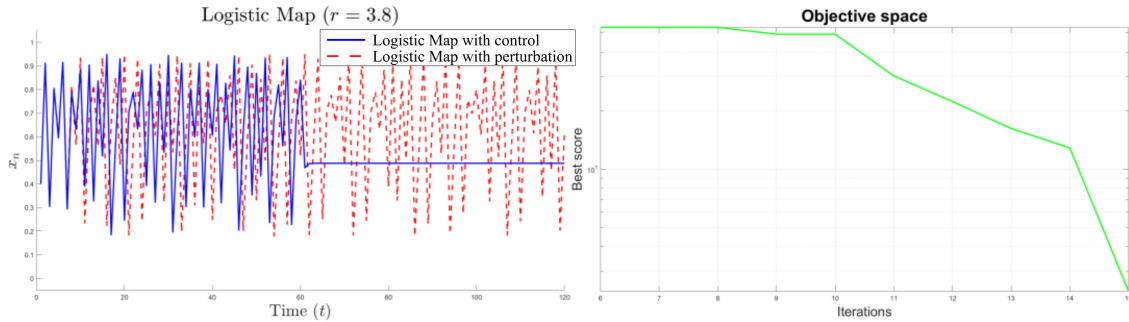
Figure 2. Application of MODPC to system (1) at r = 3.8 : (a) simulation results and (b) MAPE in each iteration.
