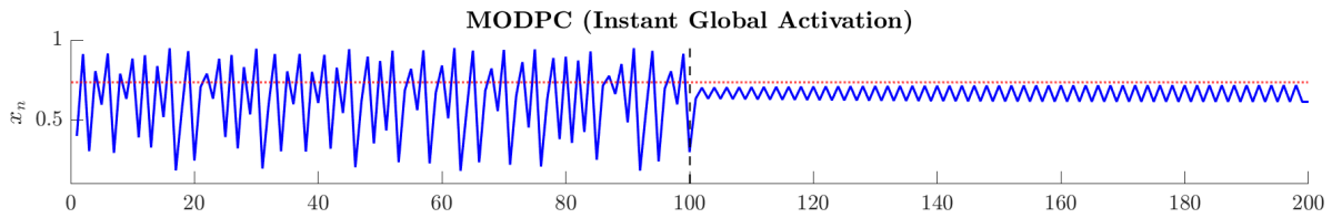
Figure 11. MODPC response when the unstable period-1 orbit of the Logistic map at r = 3.8 is directly specified as the target trajectory.
