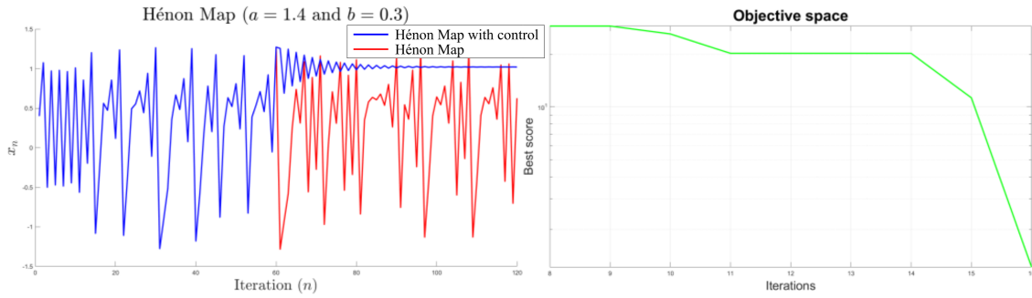
Figure 5. Application of MODPC to system (2) at a = 1.4 and b = 0.3 : (a) simulation results and (b) MAPE in each iteration.
