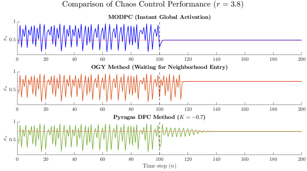
Figure 10. Numerical comparison of OGY, Pyragas DFC, and MODPC for controlling the chaotic Logistic map at r = 3.8 .
