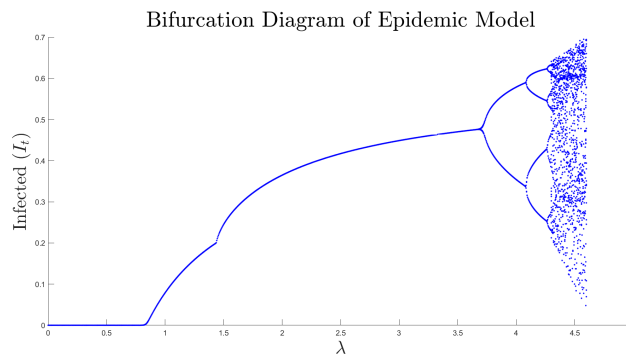
Figure 13. Bifurcation diagram of the discrete epidemic model (i.e., system (4)).
