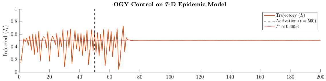
Figure 12. Control of the seventh-order epidemic model using the OGY method from the chaotic condition \lambda = 4.6 .
