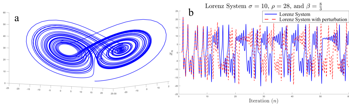
Figure 6. System (3): (a) phase portrait and (b) simulation at \sigma = 10 , \rho = 28 , and \beta = \frac{8}{3} .
