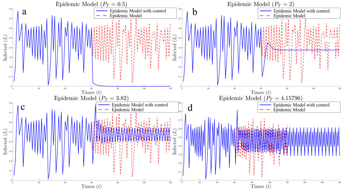
Figure 14. Simulation results from applying MODPC to system (4) with different target behaviors: (a) P_T = 0.5 , (b) P_T = 2 , (c) P_T = 3.82 , and (d) P_T = 4.15796 .
