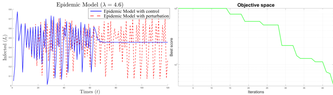
Figure 9. Application of MODPC to system (4) at \lambda = 4.6 : (a) simulation results and (b) MAPE in each iteration.
