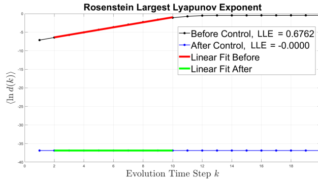
Figure 3. Data-driven estimation of the LLE using the Rosenstein algorithm for system (1) before and after the application of MODPC.
