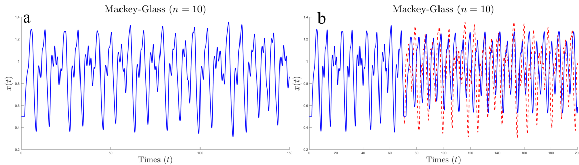
Figure 16. Simulation of equation (5) at n = 10 : (a) before and (b) after application of MODPC to achieve n = 7.5 .
