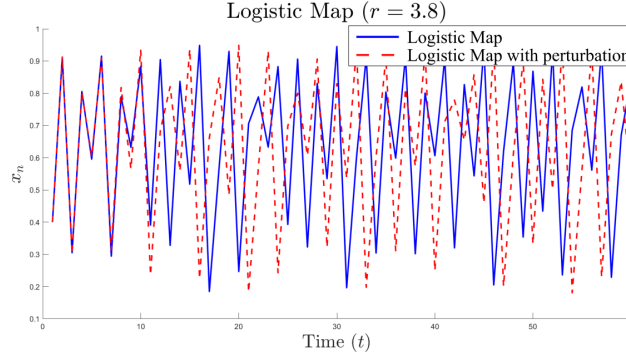
Figure 1. Simulation of system (1) at r = 3.8 .
