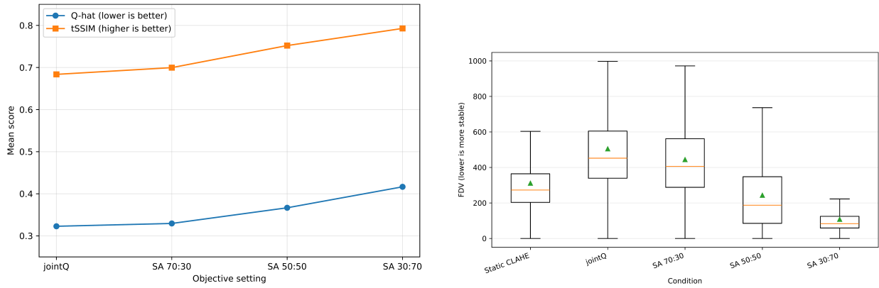
Figure 5. Quality-stability sensitivity. Left: mean \hat{Q} and tSSIM across objective settings. Right: FDV distributions for Static CLAHE and the four adaptive final objectives.
