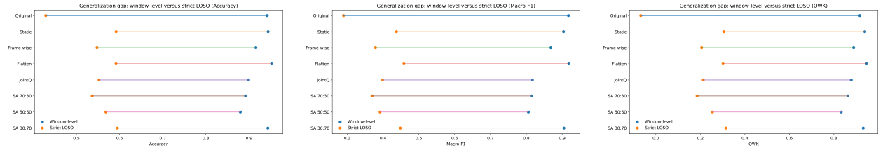
Figure 9. Descriptive generalization gap between the earlier window-level protocol and strict LOSO for Accuracy, Macro-F1, and QWK.
