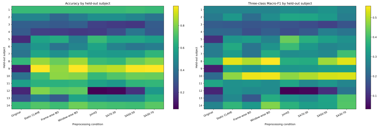
Figure 7. Strict-LOSO participant-level heterogeneity. Left: Accuracy by held-out participant and preprocessing condition. Right: fixed-three-class Macro-F1 by held-out participant and condition.
