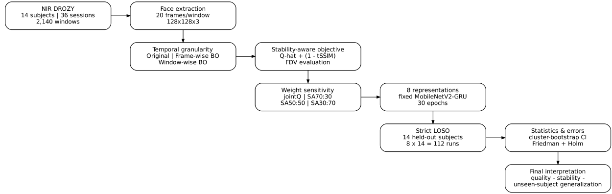
Figure 1. Overall experimental workflow from DROZY NIR videos to subject-independent LOSO interpretation. The pipeline separates the precursor temporal-granularity experiment, the final stability-aware objective study, and the downstream generalization analysis.
