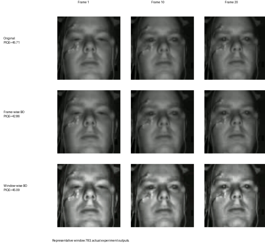
Figure 3. Actual experiment frames illustrating Original, Frame-wise BO, and legacy Window-wise BO on the same representative window.
