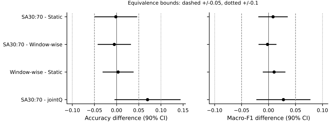
Figure 10. Paired subject-level differences with 90% confidence intervals. Dashed lines mark the primary equivalence margin ( \pm 0.05 ), dotted lines the secondary margin ( \pm 0.10 ).
