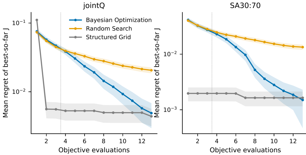
Figure 12. Mean regret of the best-so-far objective versus number of evaluations (shaded: 95% interval of the mean). The dotted line marks the end of the three initial BO evaluations.
