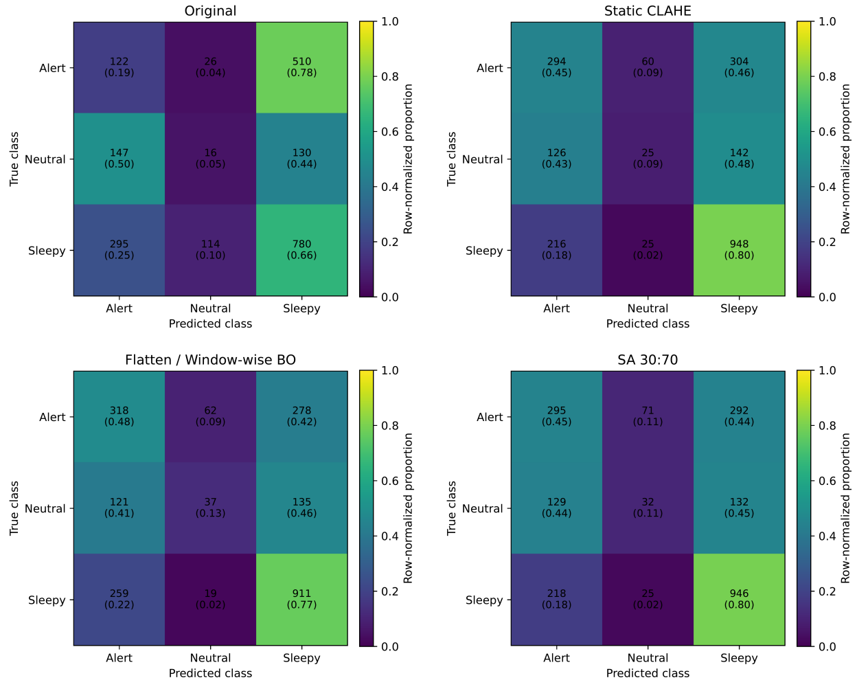
Figure 8. Pooled strict-LOSO confusion matrices for Original, Static CLAHE, Flatten/legacy Window-wise BO, and SA 30:70. Each cell shows the count and row-normalized proportion.
