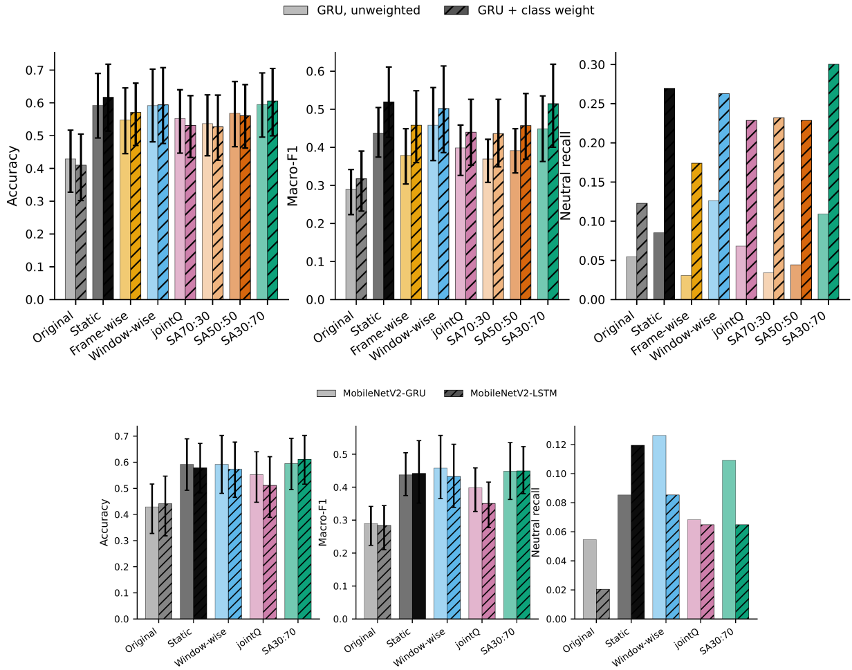
Figure 11. Sensitivity of strict-LOSO Accuracy, Macro-F1, and Neutral recall. Top: unweighted GRU (light) versus GRU with training-fold class weights (hatched). Bottom: GRU (light) versus LSTM (hatched). Error bars are 95% subject-cluster bootstrap intervals.
