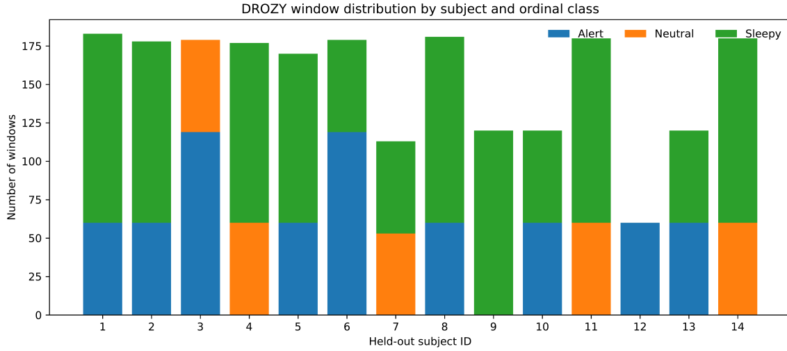
Figure 2. Distribution of the 2,140 windows across the 14 DROZY participants and three ordinal classes. The heterogeneous class composition motivates fixed-three-class Macro-F1 and explains why subject-level QWK is not used for paired inference.
