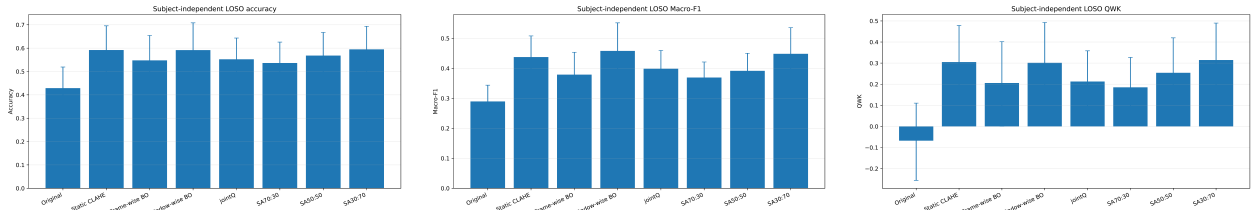
Figure 6. Pooled strict-LOSO Accuracy, Macro-F1, and QWK across eight preprocessing conditions.
