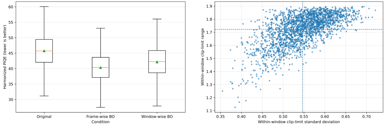
Figure 4. Temporal-granularity evidence. Left: harmonized PIQE distributions across 2,140 paired windows. Right: within-window Frame-wise clip-limit drift.
