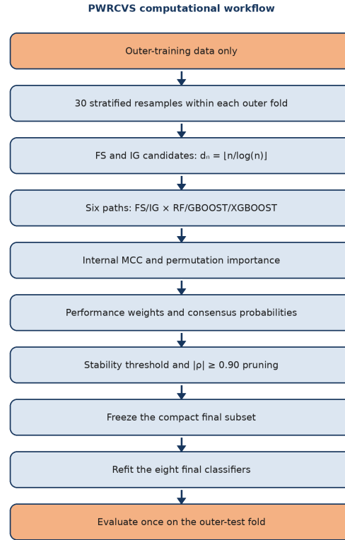
Figure 1. Leakage-controlled PWRCVS workflow. Every data-dependent operation, including filtering, path weighting, threshold selection, correlation pruning, and refitting, is completed within the outer-training sample before one evaluation on the reserved outer-test fold.
