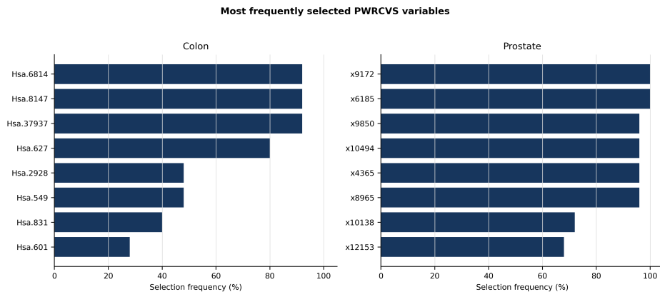
Figure 4. Selection frequency of the most recurrent PWRCVS variables across 25 outer-training selections. Frequency denotes conditional algorithmic recurrence and must not be interpreted as biological validation.
