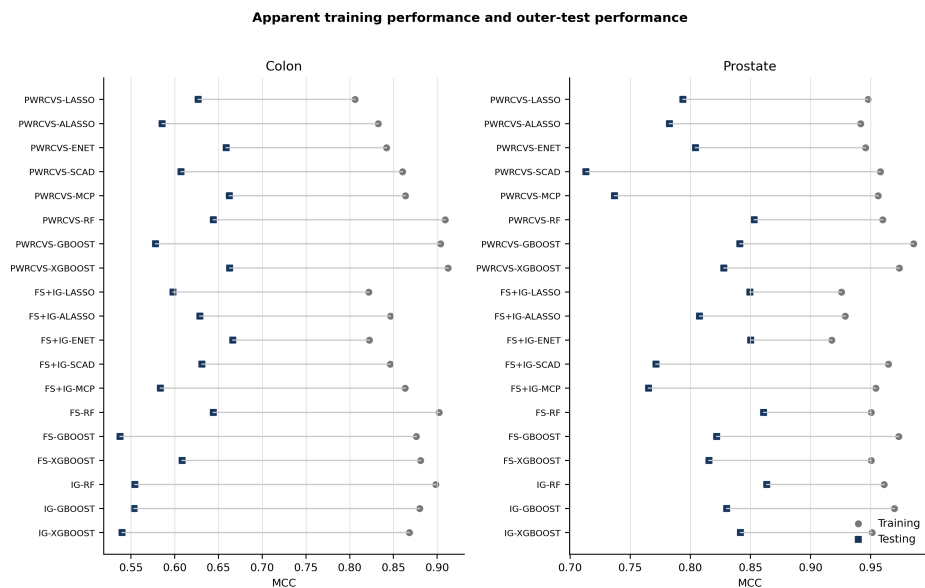
Figure 2. Apparent training MCC and mean outer-test MCC for the 19 evaluated paths. The connecting segments show the direction and magnitude of optimism, not confidence intervals; fold-to-fold standard deviations are reported in Tables 5–8.
