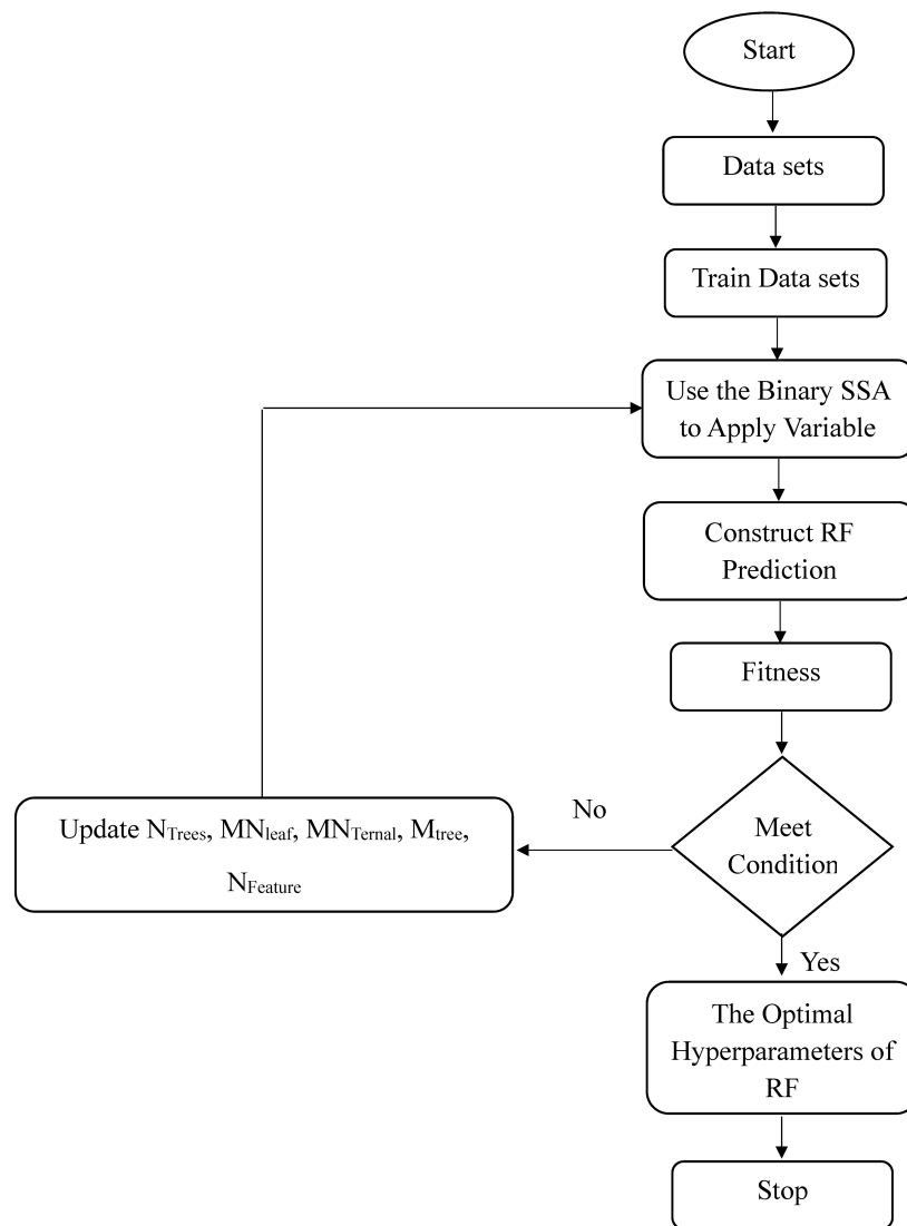
Figure 3. The architecture of the proposed ISSA-RF algorithm.
