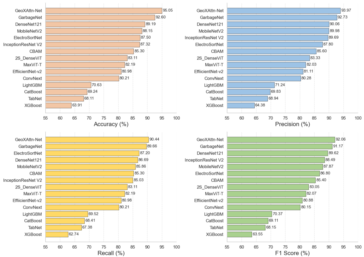
Figure 7. Comparison of the outcome of the GeoXAttn-Net method with metrics
