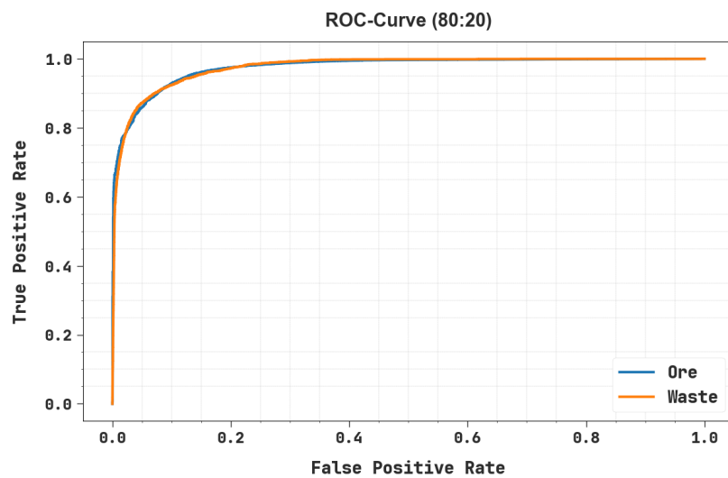
Figure 4. ROC- curve of the GeoXAttn-Net system with 80:20
