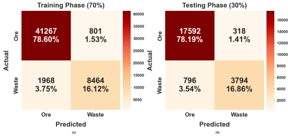
Figure 5. Confusion matrices of the GeoXAttn-Net method with 70:30 split
