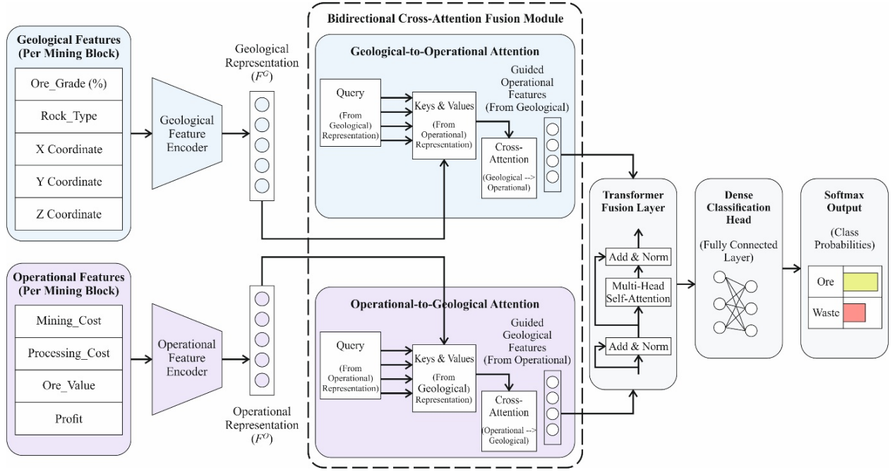
Figure 2. Internal architecture of the proposed approach demonstrating geological encoder, operational encoder, and bidirectional cross-attention fusion.
