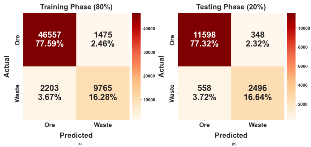
Figure 3. Confusion matrices of the GeoXAttn-Net method with 80:20 split
