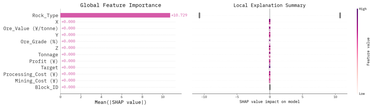
Figure 8. SHAP value for the global and local explanation
