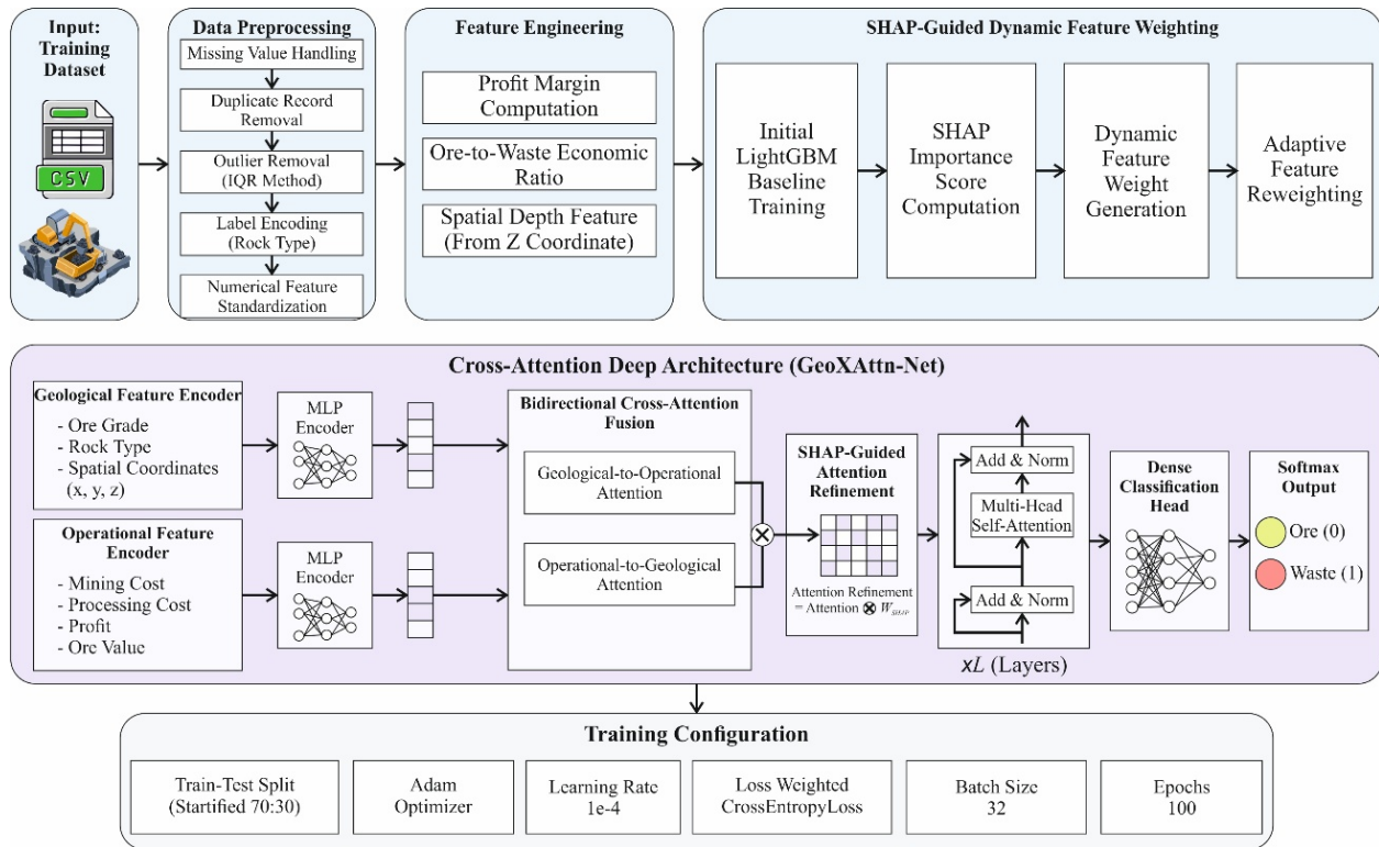
Figure 1. Overall architecture of the proposed GeoXAttn-Net approach
