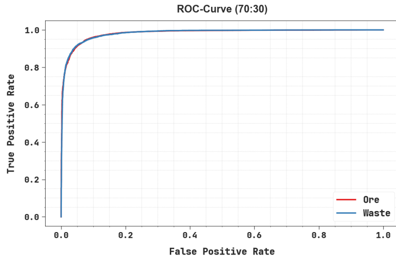
Figure 6. ROC-curve of the GeoXAttn-Net approach with 70:30
