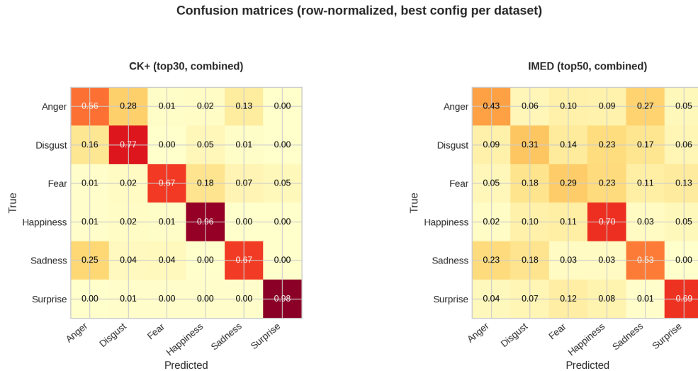
Figure 8. Row-normalized confusion matrix for the best configuration, both datasets.
