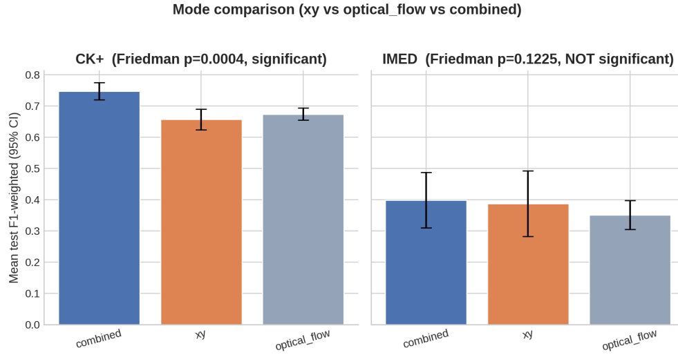
Figure 4. Input modality comparison, both datasets.
