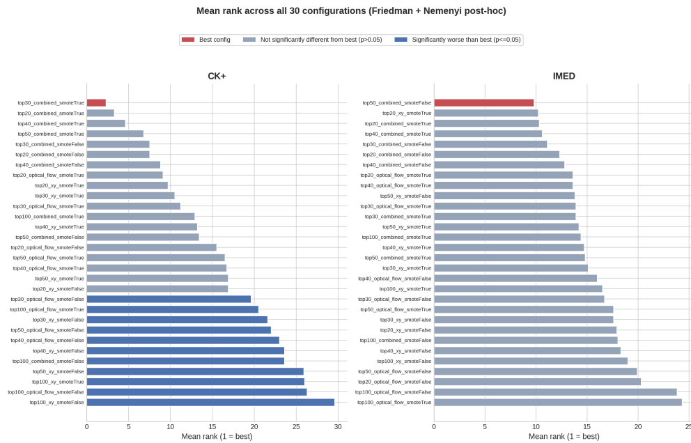
Figure 2. Mean rank across all 30 configurations, both datasets.
