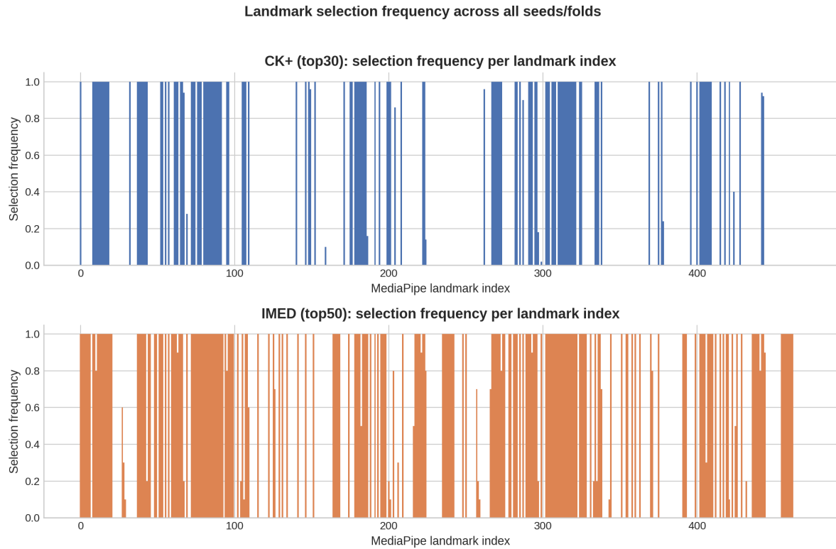
Figure 6. Landmark selection frequency across seeds and folds, both datasets.
