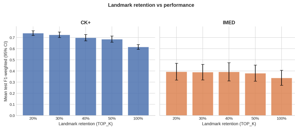
Figure 3. Landmark retention (Top-K) versus performance, both datasets.
