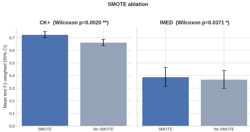
Figure 5. BorderlineSMOTE ablation, both datasets.
