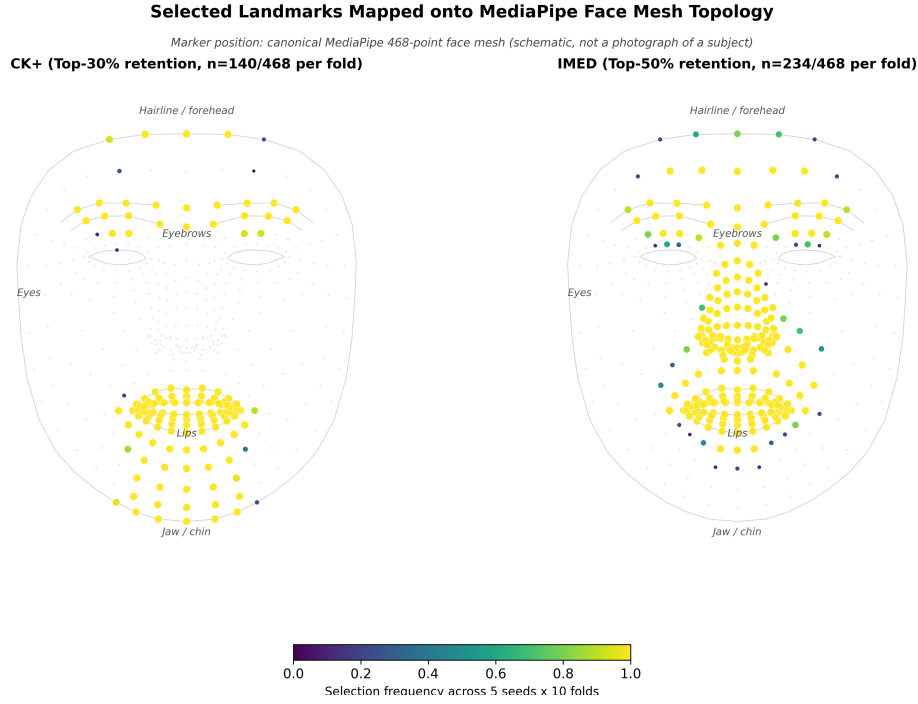
Figure 7. Selected landmarks mapped onto the MediaPipe canonical face-mesh template. Selection frequency per index is the fraction of the 50 fold-seed runs (headline configuration) in which that index appears in the selected set, plotted at that index's canonical (x, y) position (geometric template only, no photograph or identity).
