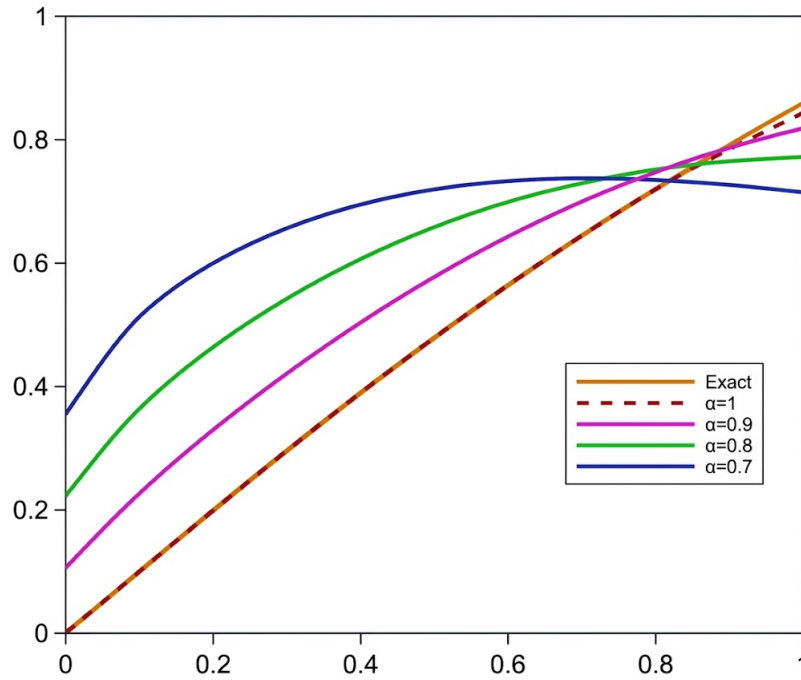
Figure 1. Different values for \alpha of approximate solution and comparison between \alpha = 1 and the exact solution.
