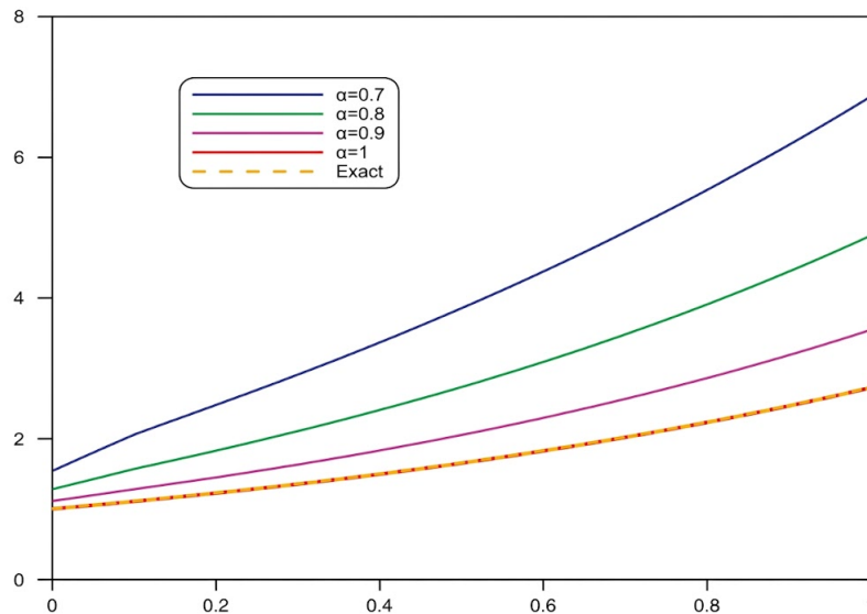
Figure 3. Different values for \alpha of approximate solution and comparison between \alpha = 1 and the exact solution.
