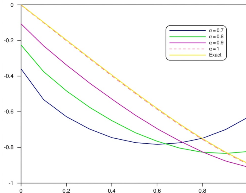
Figure 2. Different values for \alpha of approximate solution and comparison between \alpha = 1 and the exact solution.
