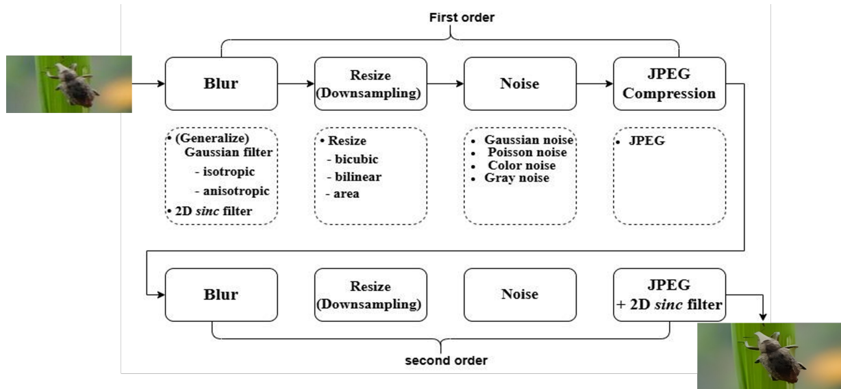
Figure 6. Generated Synthetic Data in Real-ESRGAN.
