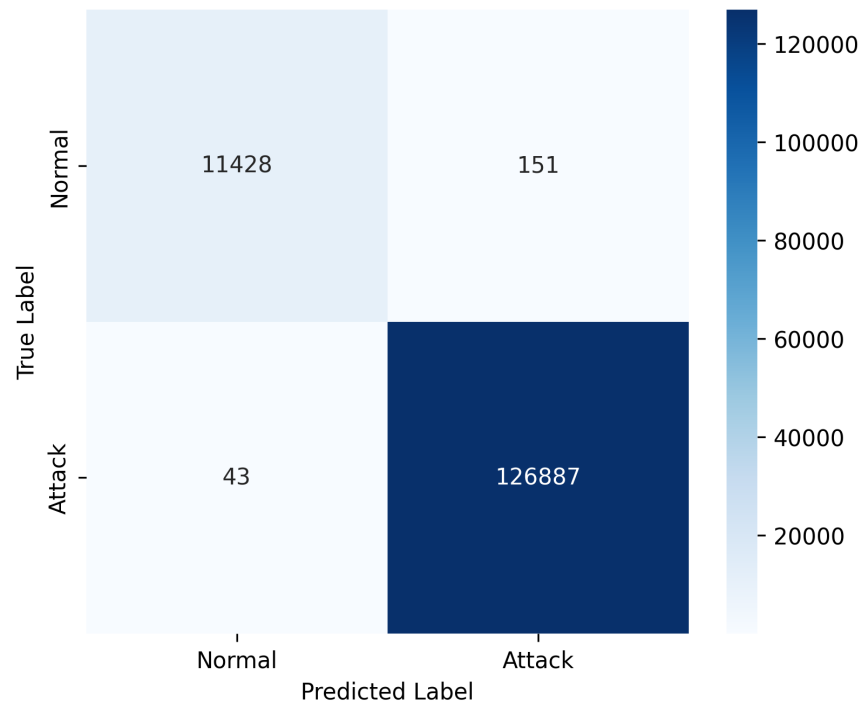
Figure 9. ASAE Confusion Matrix on IOTID20 Dataset.
