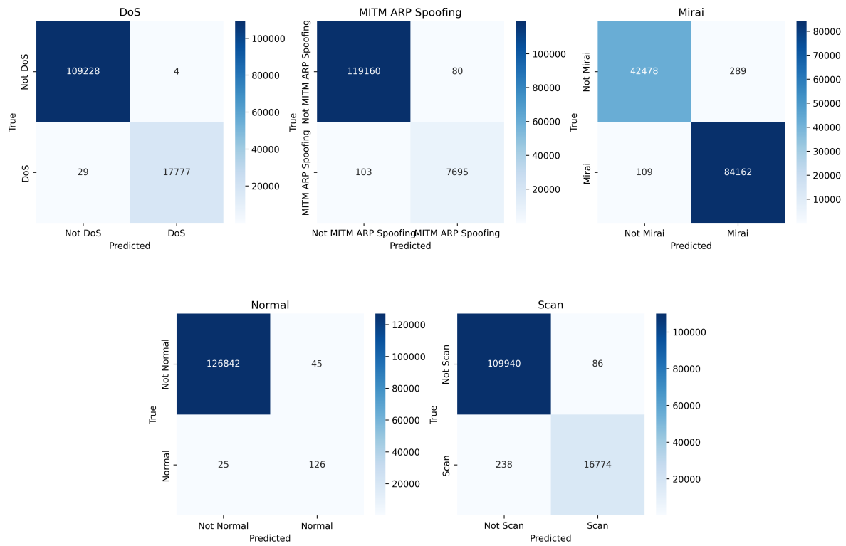
Figure 13. One-vs-Rest Confusion Matrices on IOTID20 Dataset.
