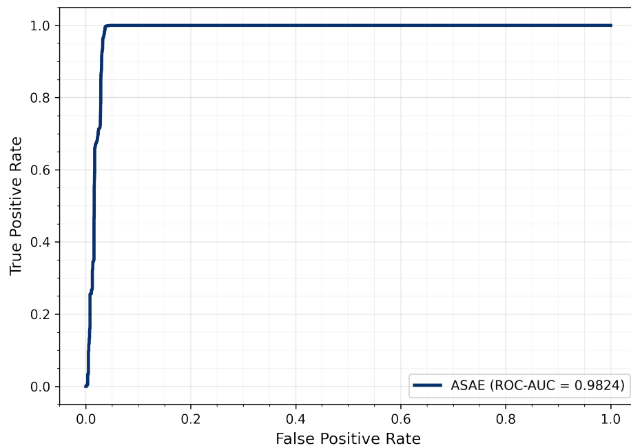
Figure 3. ASAE ROC curve on TON_IoT Network Dataset.
