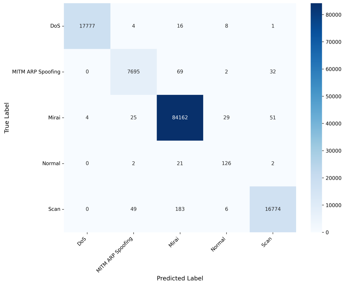
Figure 12. Multi-class Confusion Matrix on IOTID20 Dataset.
