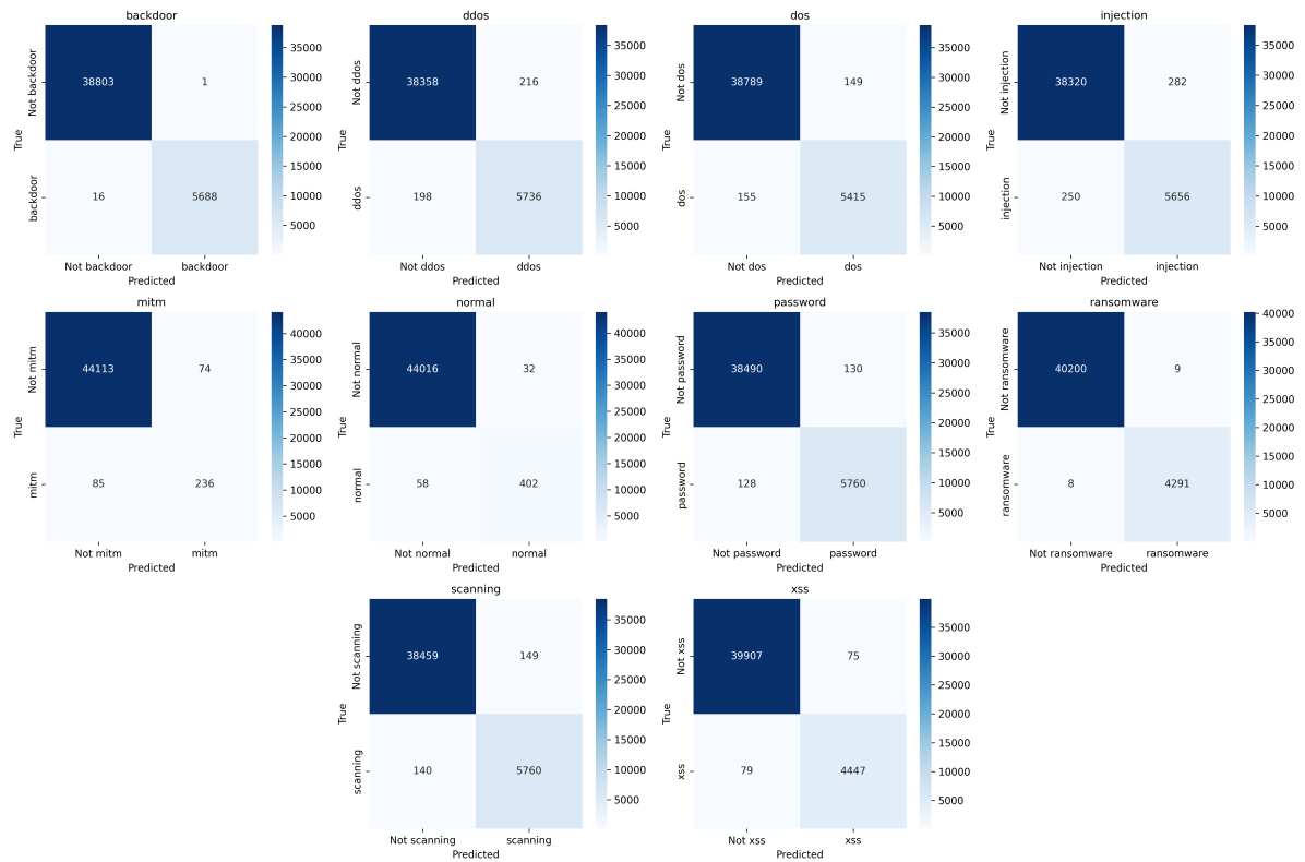
Figure 6. One-vs-Rest Confusion Matrices on TON_IoT Network Dataset.
