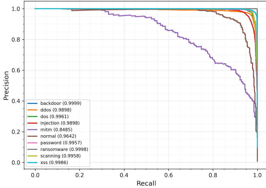
Figure 8. One-vs-Rest PR Curves on TON_IoT Network Dataset.
