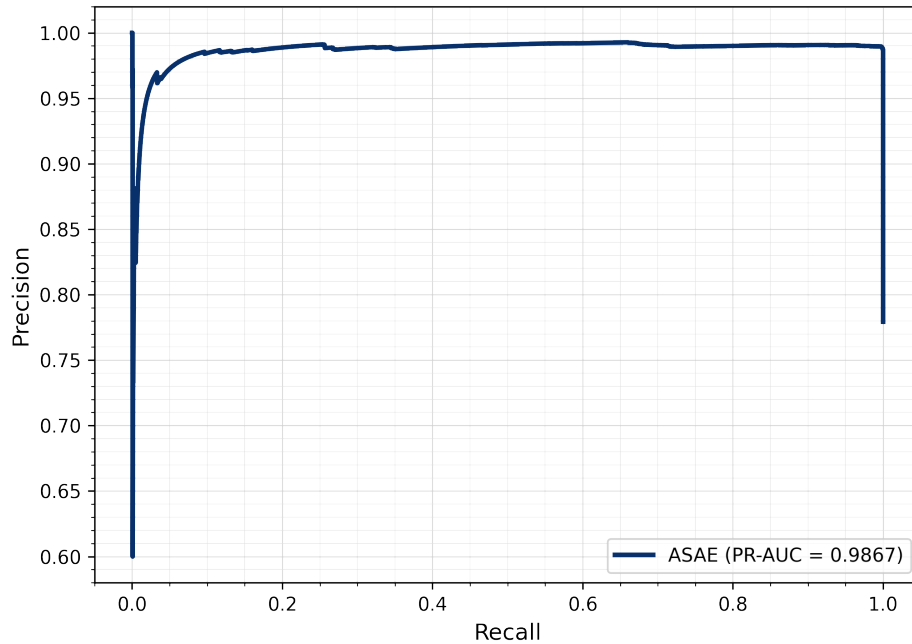
Figure 4. ASAE PR curve on TON.IoT Network Dataset.
