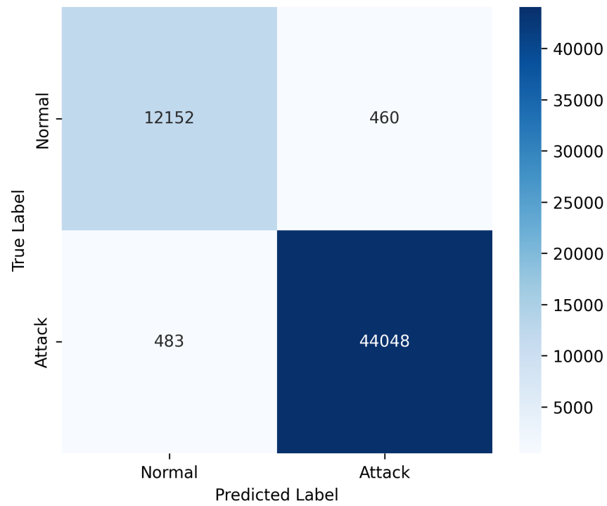
Figure 2. ASAE Confusion Matrix on TON_IoT Network Dataset.
