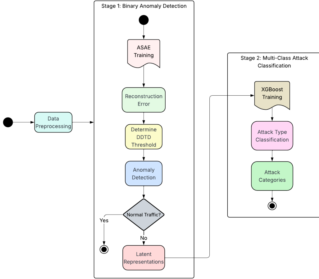
Figure 1. Architecture of the proposed framework.
