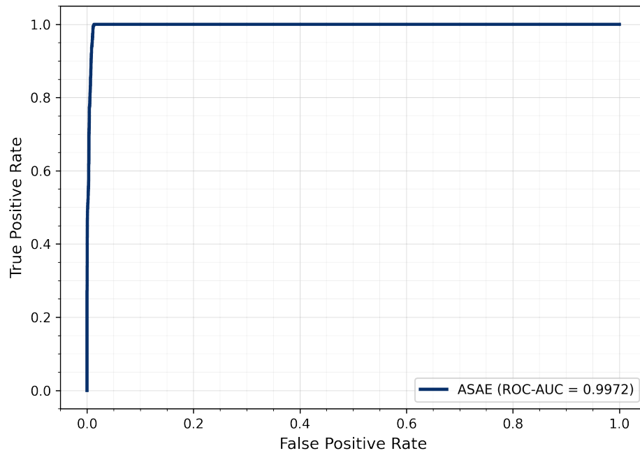
Figure 10. ASAE ROC curve on IOTID20 Dataset.
