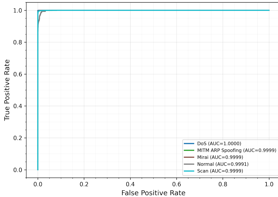
Figure 14. One-vs-Rest ROC Curves on IOTID20 Dataset.
