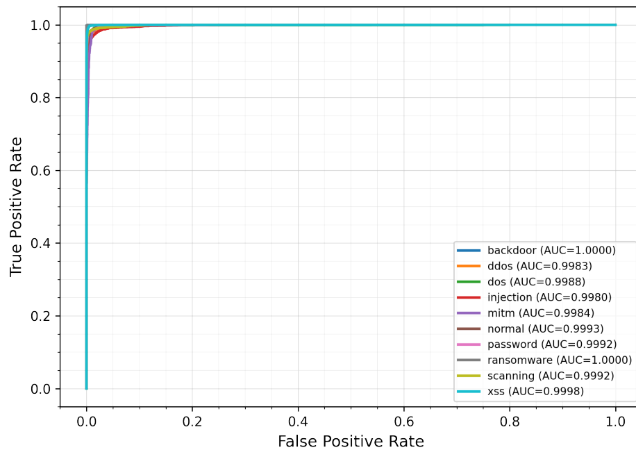
Figure 7. One-vs-Rest ROC Curves on TON_IoT Network Dataset.
