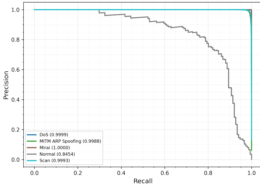
Figure 15. One-vs-Rest PR Curves on IOTID20 Dataset.
