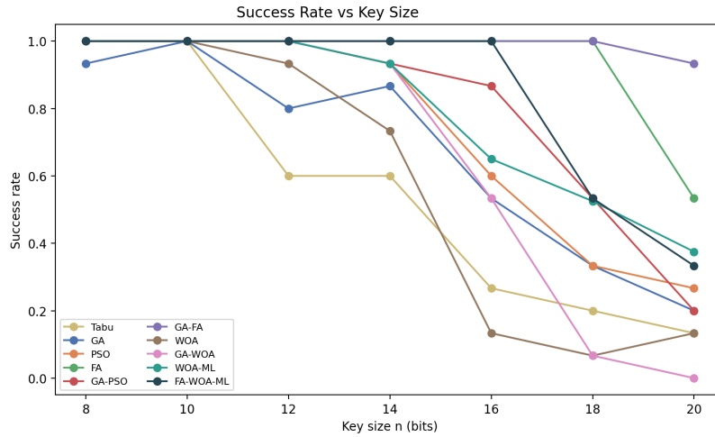
Figure 3. Success rate versus key size n .
