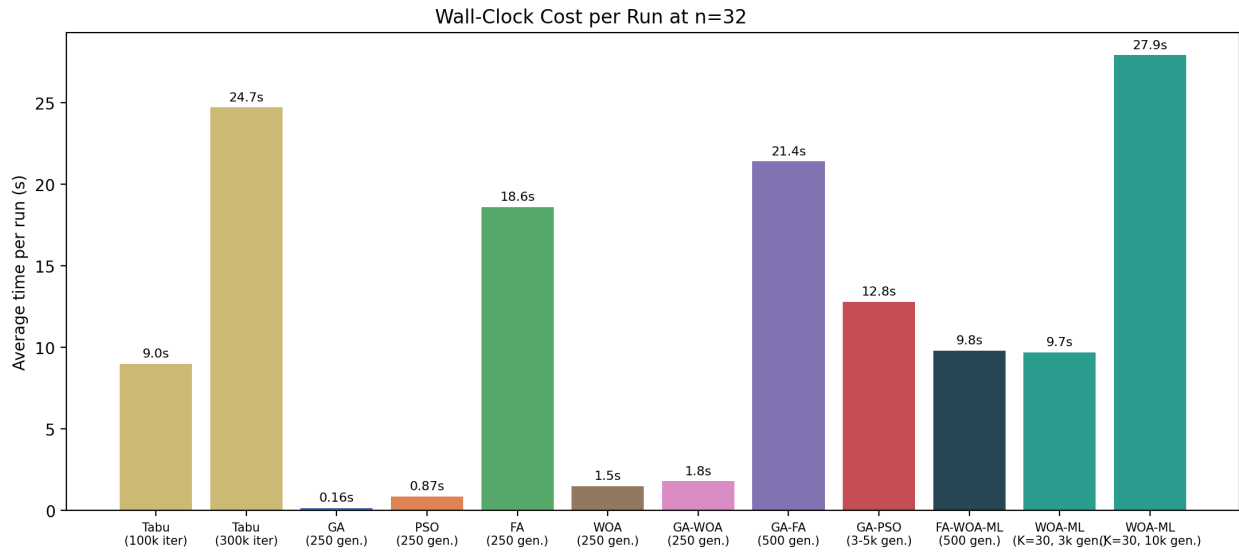
Figure 8. Average wall-clock time per run at n = 32 .
