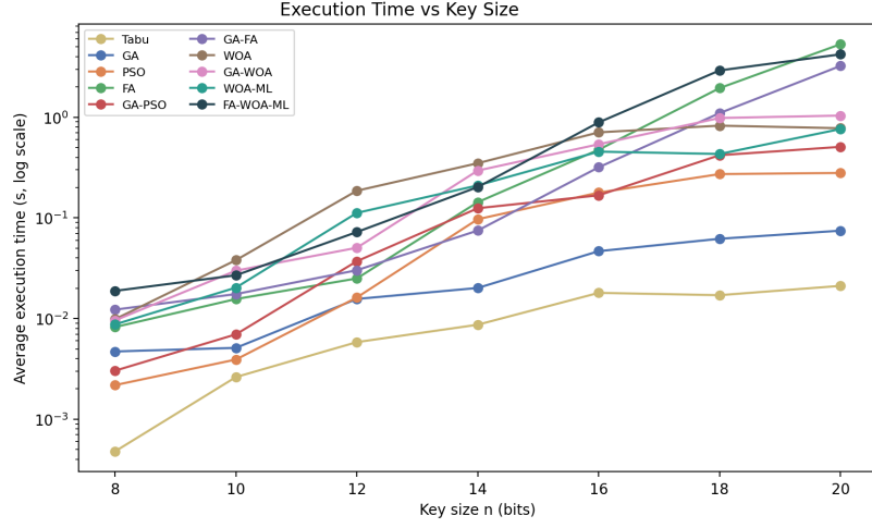
Figure 4. Average execution time versus key size n (log scale).
