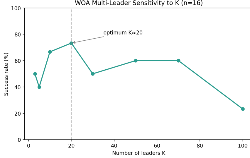
Figure 7. WOA-ML success rate versus number of leaders K , at n = 16 ( P = 100 , 30 runs per value).
