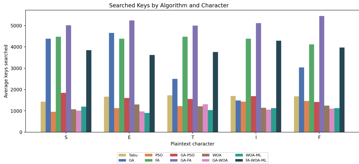
Figure 12. Average number of keys searched by algorithm and plaintext character, at n = 10 (baseline experiment of §3).
