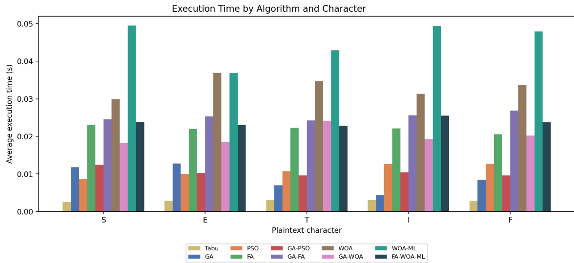
Figure 11. Average execution time by algorithm and plaintext character, at n = 10 (baseline experiment of §3).
