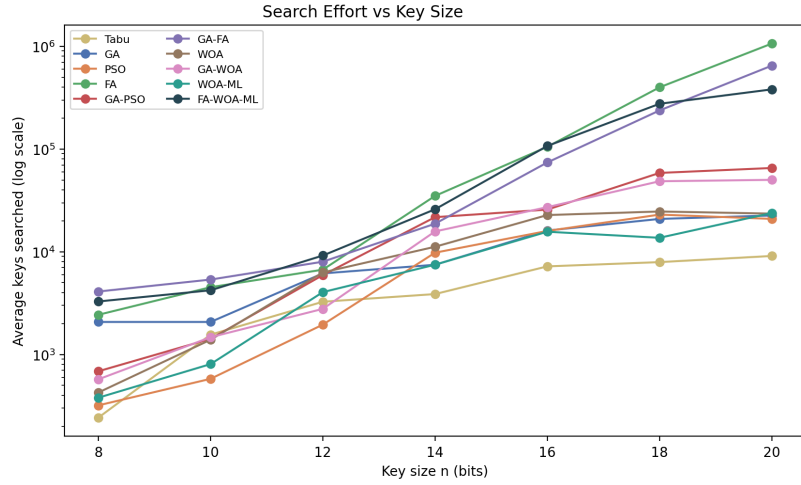
Figure 5. Average keys searched versus key size n (log scale).
