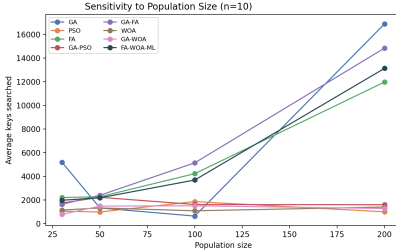
Figure 9. Average keys searched as a function of population size, for all eight methods with a population-size parameter.
