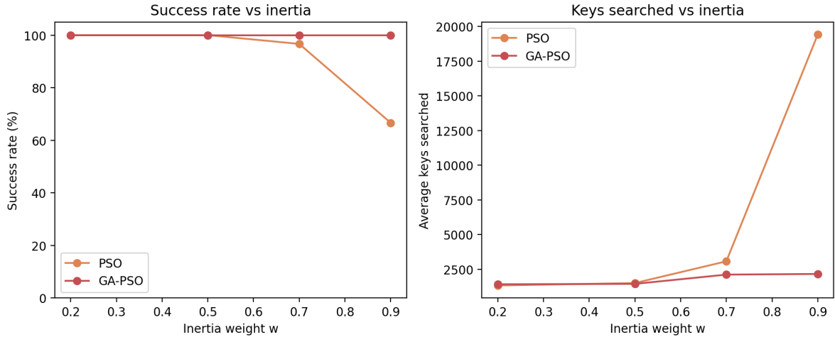
Figure 10. Success rate and keys searched versus inertia weight w , for PSO and GA-PSO.
