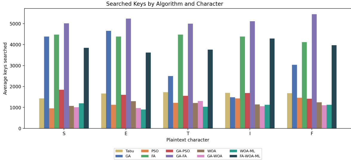
Figure 2. Average keys searched by algorithm and character.
