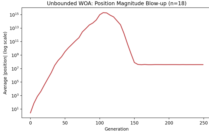
Figure 6. Average |\text{position}| across the population over 250 generations of unbounded WOA at n = 18 (log scale).
