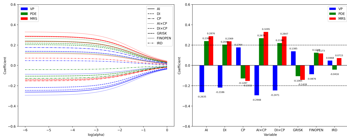
Figure 4. LASSO Coefficient Paths and Selected Coefficients for FX Market Outcomes
