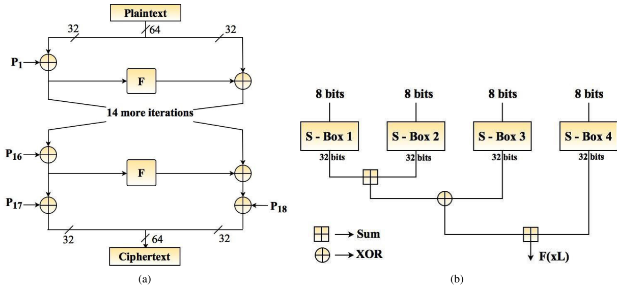
Figure 4. Graphical representation of (a) Blowfish algorithm (b) Function module (F) [18, 19].
