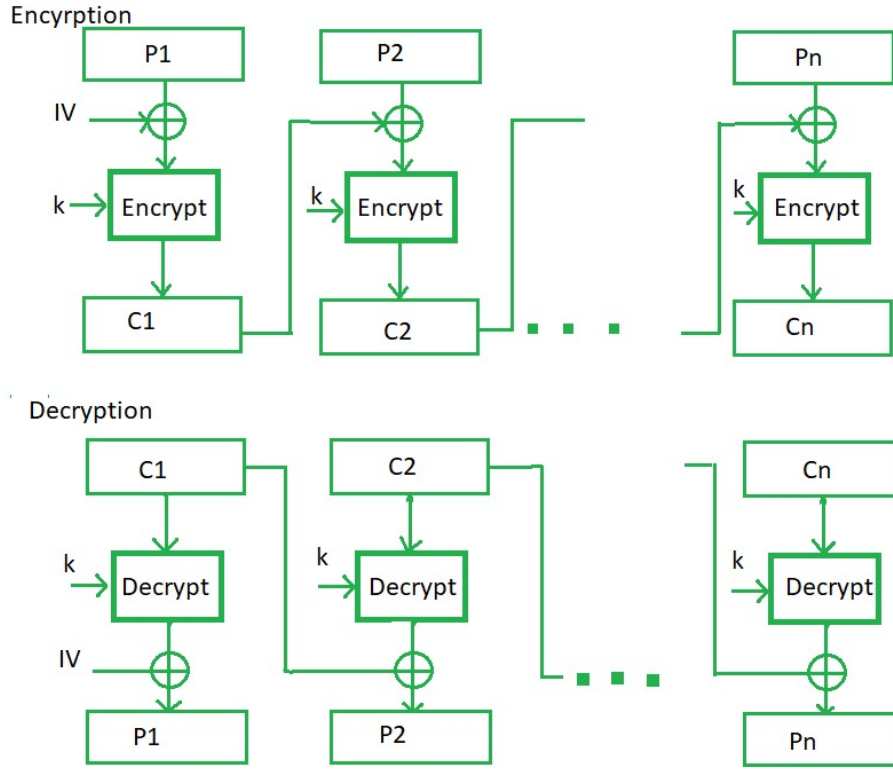
Figure 5. shows the steps of CBC mode for blowfish algorithm.
