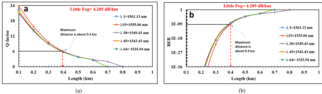
Figure 8. (a) Q-Factor as a goal of a link path and (b) BER as a goal of a link length for multi-wavelengths without an amplifier. The obtained link the distance approximates 0.4 km under attenuation equal (4.285 dB/km) with dim weather fog condition.
