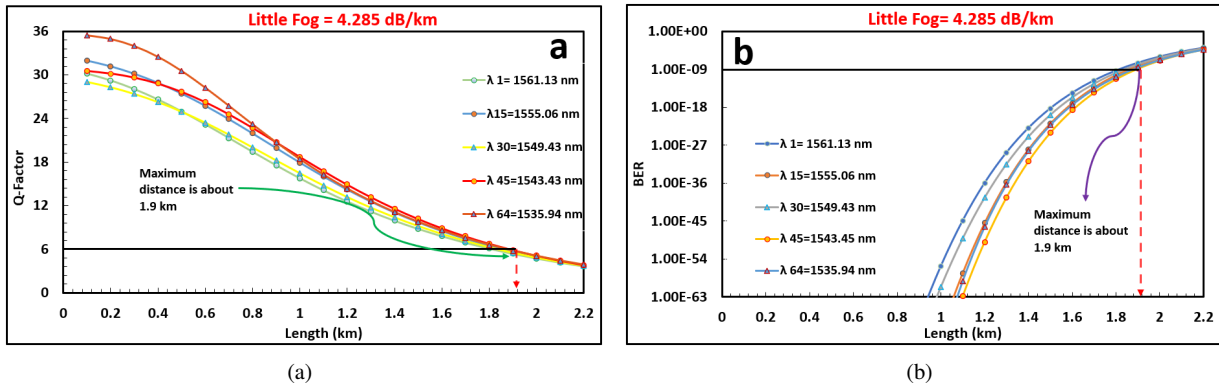
Figure 9. (a) Q-Factor as a goal of a link path and (b) BER as a goal of a link length for multi-wavelengths. The obtained link the distance approximates 1.9 km under attenuation equal (4.285 dB/km) with dim weather fog condition.
