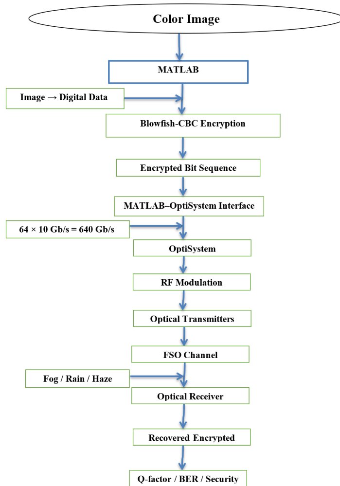
Figure 6. Block Diagram of the integration process OptiSystem with Matlab.
