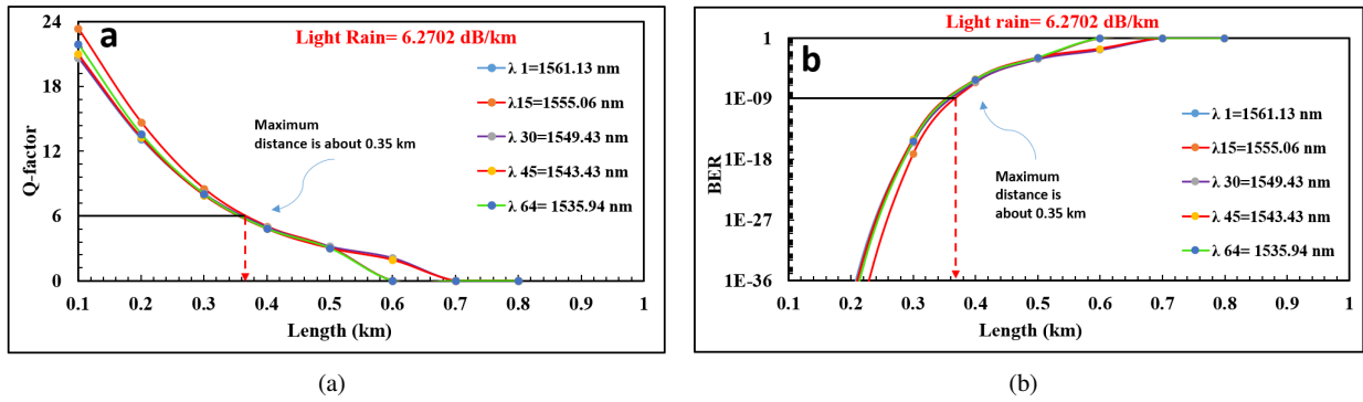
Figure 10. (a) an illustration of the Q-Factor as a goal of link path, (b) BER as a goal of link range at a little rainfall weather condition under attenuation equal 6.2702 (dB/km) for many wavelengths without an amplifier, and approximately 0.35 km as the achieved link range.
