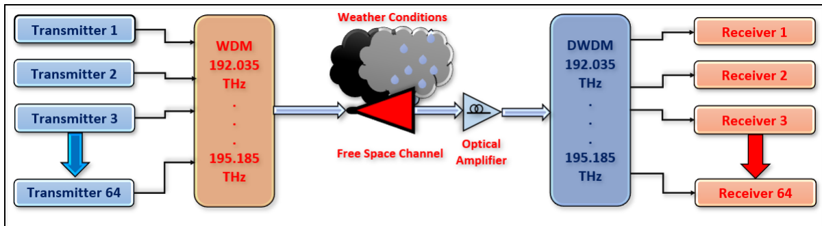
Figure 1. Ro-FSO system schematic diagram.
