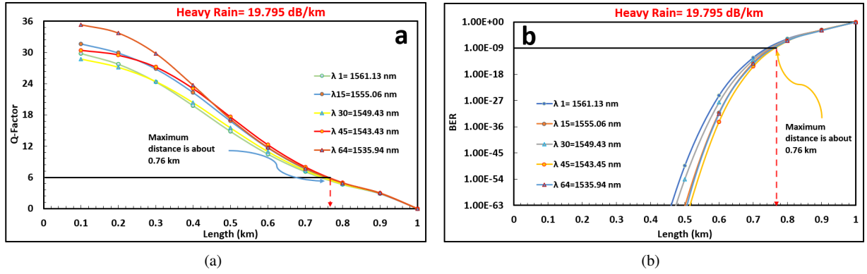
Figure 15. (a) Q-Factor as a goal of a link and (b) BER as a goal of a link length investigated at intense rain equal attenuation at 19.795 (dB/km) for many wavelengths and about 0.76 km is the achieved link range.
