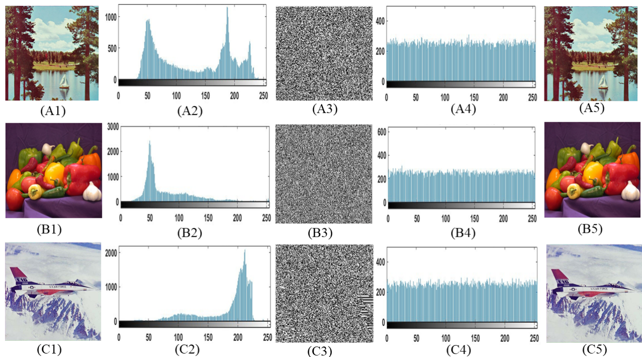
Figure 18. The simulation result: plain images (A1–C1), histogram of the plain images (A2–C2), encrypted image (A3–C3) histogram of the encrypted image (A4–C4) and the retrieved images (A5–C5).
