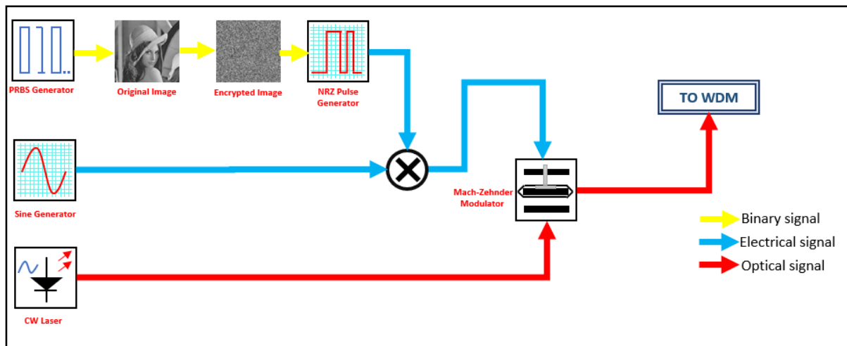
Figure 2. The components of the transmitter subsystem.
