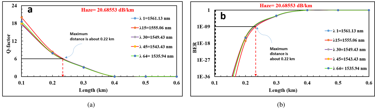
Figure 16. (a) Q-Factor as a goal of the link and (b) BER as a goal a link length at a hazy weather under attenuation equal 20.68553 (dB/km) for many wavelengths without an amplifier and about 0.22 km is the achieved link range.
