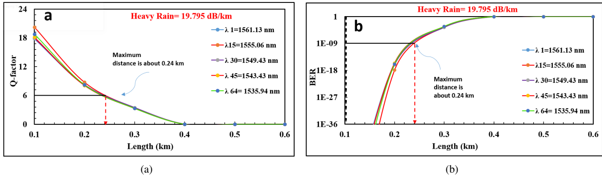
Figure 14. (a) Q-Factor as a goal of a length and (b) BER as a goal of a link length investigated at intense rain equal attenuation at 19.795 dB/km for a number of wavelengths with no amplifier and about 0.24 km is the achieved link range.
