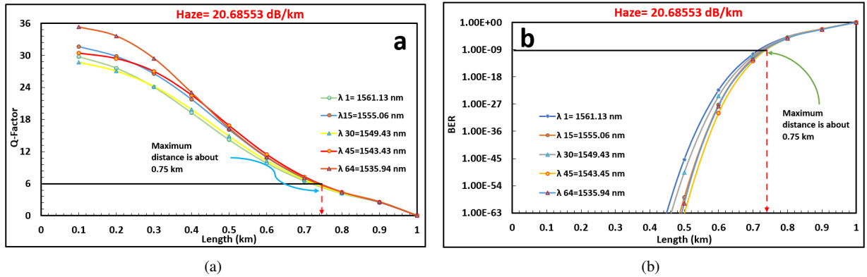
Figure 17. (a) Q-Factor as a goal of the length and (b) BER as a goal a link length at a hazy weather under attenuation equal 20.68553 dB/km for several wavelengths and about 0.75 km is the achieved link range.
