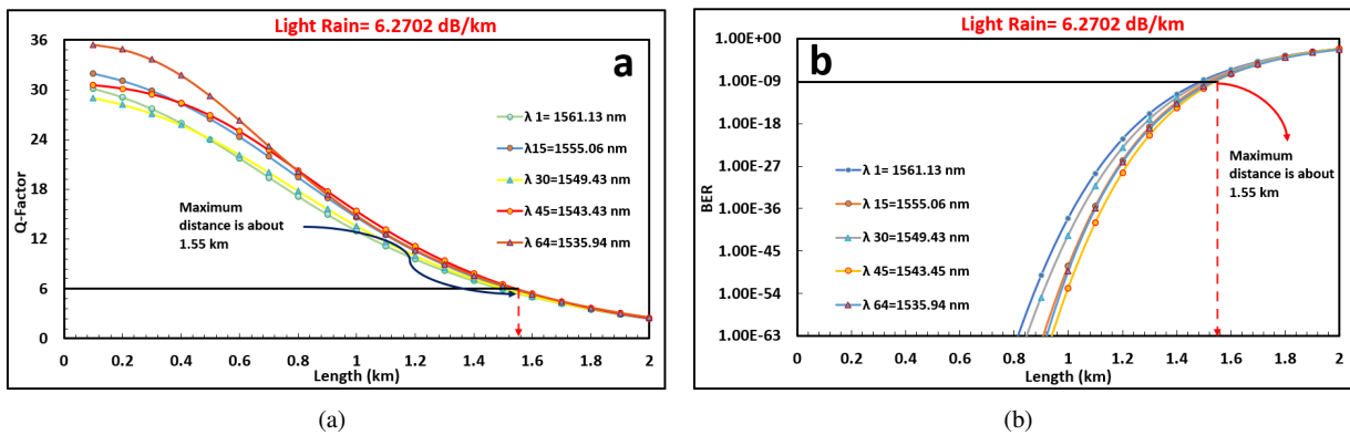
Figure 11. (a) an illustration of the Q-Factor as a goal of link path, (b) BER as a goal of link range at a little rainfall weather condition with an attenuation of 6.2702 (dB/km) for many wavelengths, and approximately 1.55 km as the connection length attained.
