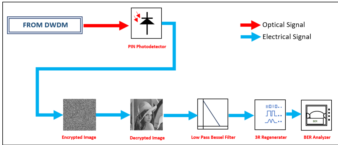
Figure 3. The components of the subsystem of the receiver.
