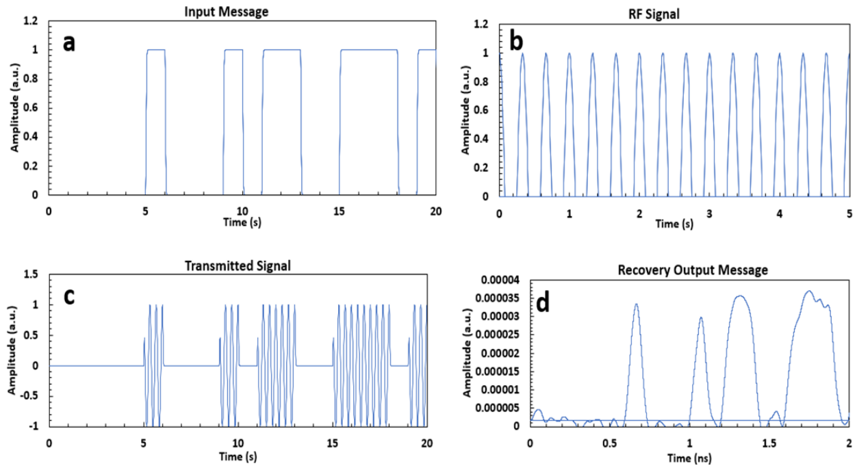
Figure 7. Time domain of signal spectrum's (a) the signal of input electrical message, (b) the signal of RF, (c) the transmitted signal in the optical form, (d) the recovered electrical signal at a maximum transmitted distance of 1.9 km under a light fog.
