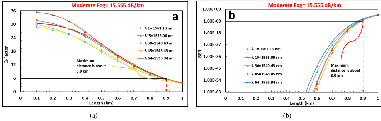
Figure 13. (a) Q-Factor as a goal of length and (b) BER as a goal of link length range at Medium fog equal attenuation at 15.555 (dB/km) for many wavelengths and 0.9 km as the achieved link range.
