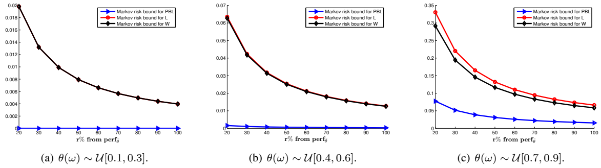
Figure 6. Markov risk bounds for the main performance measures of M/E 2 /1/10 queue with dependent breakdowns.
