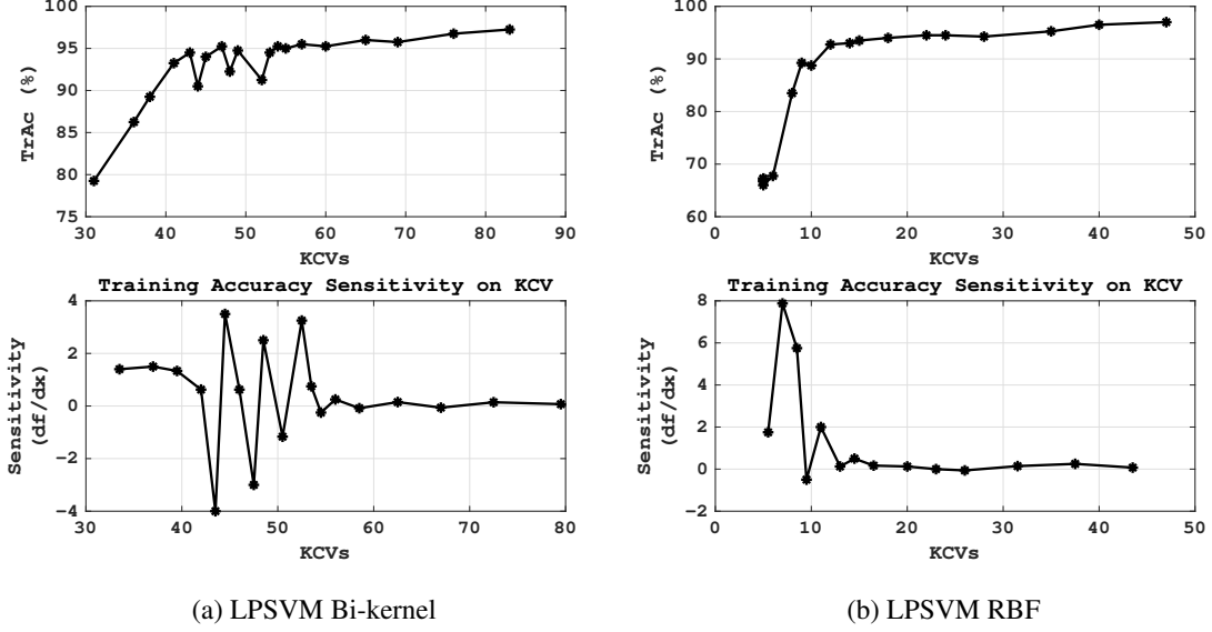
Figure 3. Training Accuracy & Accuracy-Sensitivity on KCV. Very low and nearly flat sensitivity in the top accuracy region is interesting.
