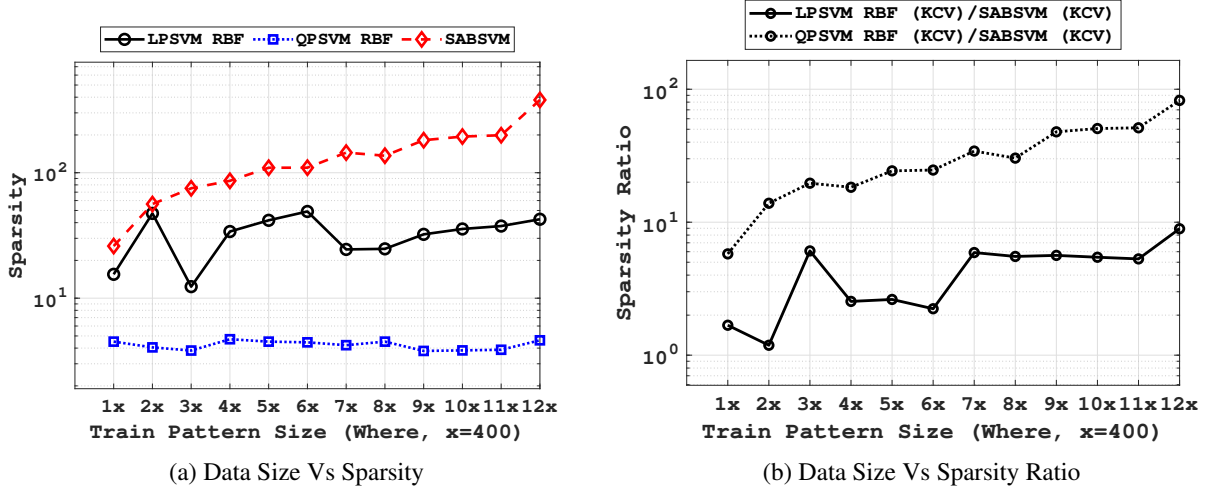
Figure 6. Sparsity with variational training pattern size
