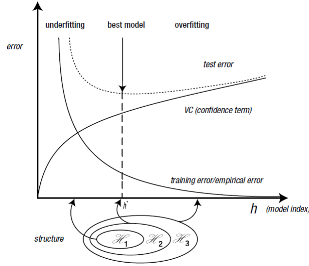
Figure 4. Error Trends On Model Complexity [64].
