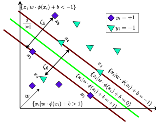
Figure 5. A visual representation of the standard SVM[21]
