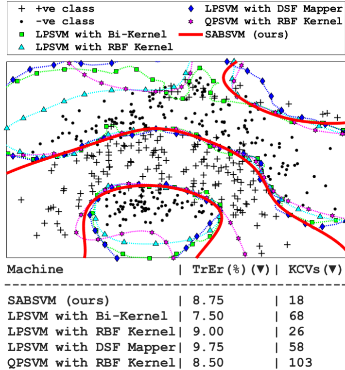
Figure 1. Decision boundaries on Banana data ( 400 \times 2 ) from proposed SABSVM & some other SOTA machines. From the small metric values above, it can be traced that using the least number of ( = 18 ) Kernel computing Vectors (KCVs) among all, the proposed SABSVM produces Training error (TrEr) of 8.75% very near to the other high accuracy machine, leading to the lowest (157.5) Machine's Error-Cost Loss (MECL, defined later) compared to others (234, 510, 565.5 and 875.5 respectively) as desired. Its decision boundary (red solid line) also looks quite smooth yet powerful.
