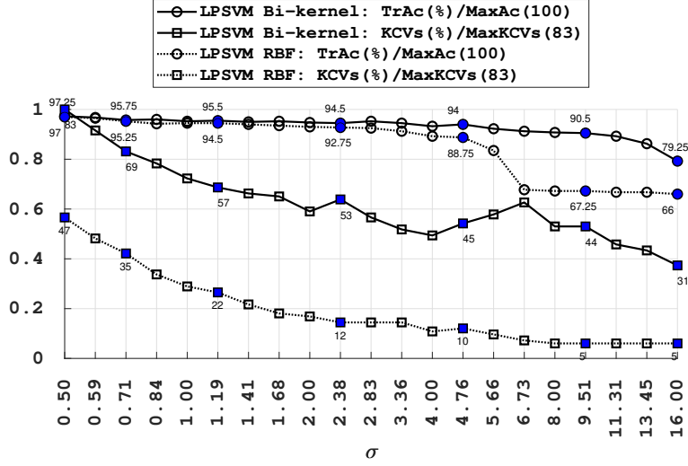
Figure 2. Training Accuracy & #KCV on Kernel Parameter, \sigma from LPSVM
