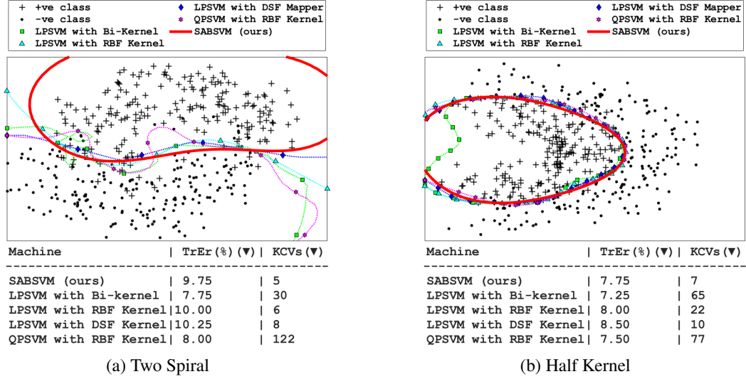
Figure 7. Decision boundaries on Synthetic data ( 400 \times 2 ) from proposed SABSVM & some other SOTA machines
