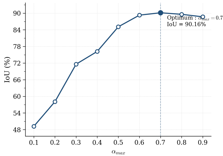
Figure 3. Influence of the adaptive loss parameter \alpha_{max} on IoU for BRATS dataset.
