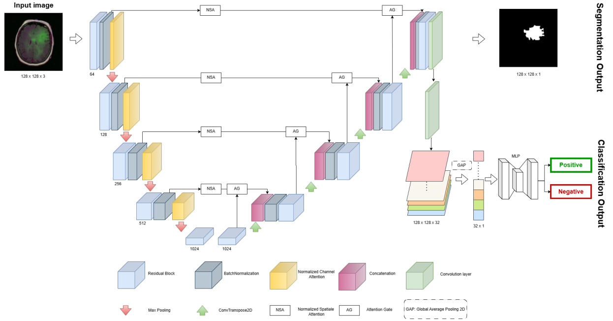
Figure 1. Diagram of the proposed method showing the encoder-decoder architecture with optimized attention mechanisms and joint classification-segmentation outputs.
