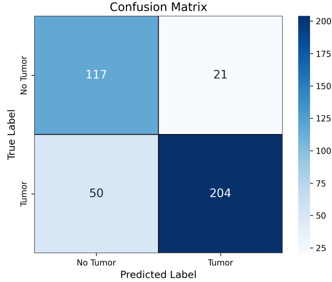
Figure 5. Image-level confusion matrix of the ablation without the classification branch on the LGG test set ( \alpha_{\max} = 1 , i.e. pure Dice loss).
