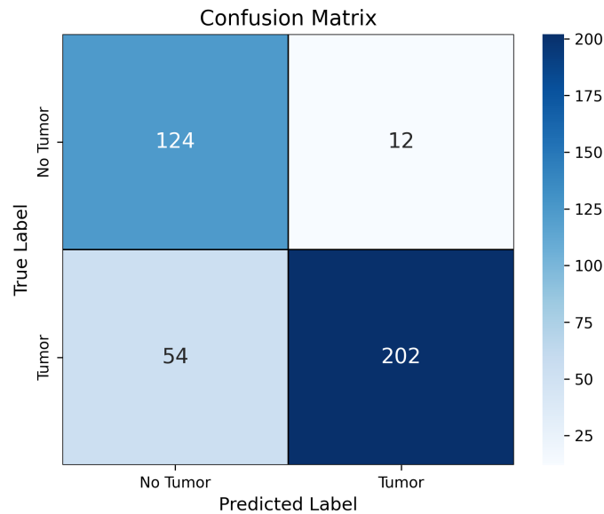
Figure 4. Image-level confusion matrix of the proposed joint model on the LGG test set ( \alpha_{max} = 0.7 ).
