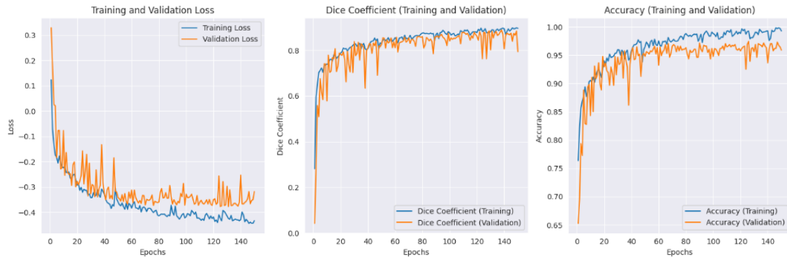
Figure 10. Training and validation learning curves on the LGG dataset.
