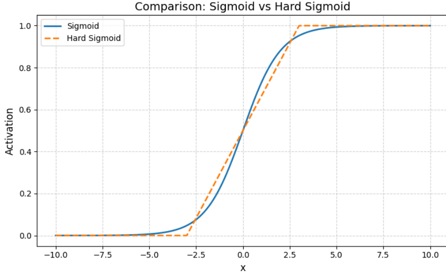
Figure 2. Comparison of sigmoid and hard sigmoid activation functions showing computational efficiency gain while maintaining similar scaling behavior.
