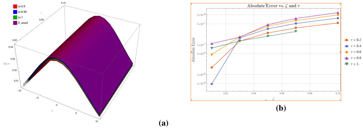
Figure 5. (a) 3D plots of \Omega(x,t) for \alpha = 0.9, 0.95, 1 and \Omega_{\text{exact}} , with -10 \leq x \leq 10 , 0 \leq t \leq 0.10 , showing the convergence to the exact solution and memory induced damping: smaller \alpha values lead to smaller and smoother amplitude. (b) the 2D graph of the Absolute error for any value of \tau and \alpha = 0.90, 0.95, 1 , Exactsolution
