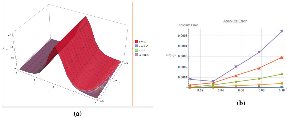
Figure 2. (a) 3D plots of \Omega(x, t) for \alpha = 0.9, 0.95, 1 and \Omega_{\text{exact}} , with -10 \leq x \leq 10 , 0 \leq t \leq 0.10 , showing the convergence to the exact solution and memory induced damping: smaller \alpha values lead to smaller and smoother amplitude. (b) the 2D graph of the Absolute error for any value of \tau and \alpha = 0.90, 0.95, 1 , \Omega_{\text{exact}}
