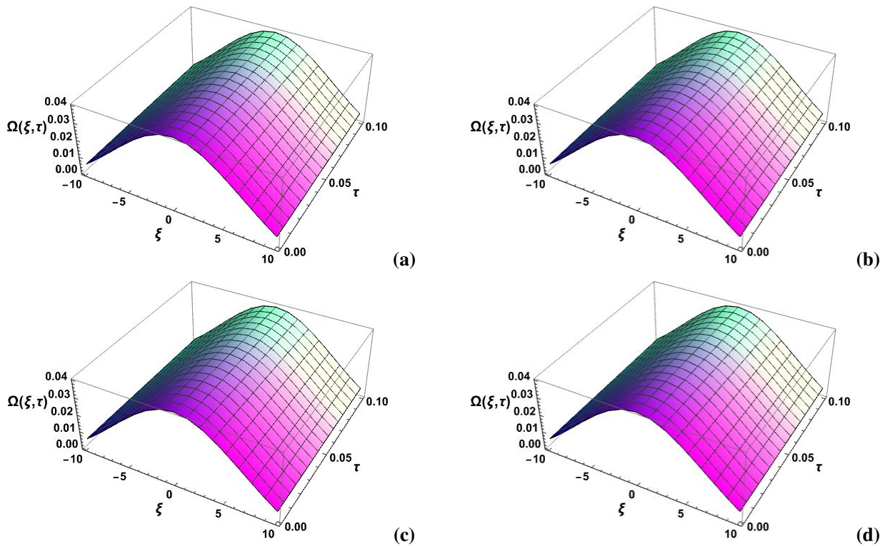
Figure 4. The graphs for Example 2 Three-dimensional representations of the approximate solutions Laplace New Iterative Method (LNIM) for \Omega(\xi, \tau) for Example 2: (a) \alpha = 0.90 , (b) \alpha = 0.95 and (c) \alpha = 1 as against (d) the corresponding exact solution. The axes of the horizontal represent the spatial variable \xi and the time variable \tau , respectively. the vertical axis is the solution \Omega(\xi, \tau) . The near agreement of the approximate and exact solutions indicates the accuracy of the proposed LNIM.
