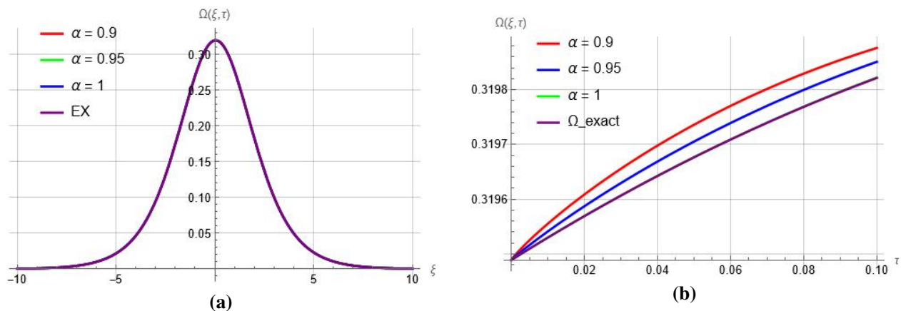
Figure 3. (a) The 2D graph of the \Omega for any value of \xi and \alpha = 0.90, 0.95, 1 , \Omega_{\text{exact}} (b) the 2D graph of the \Omega for any value of \tau and \alpha = 0.90, 0.95, 1 , \Omega_{\text{exact}}
