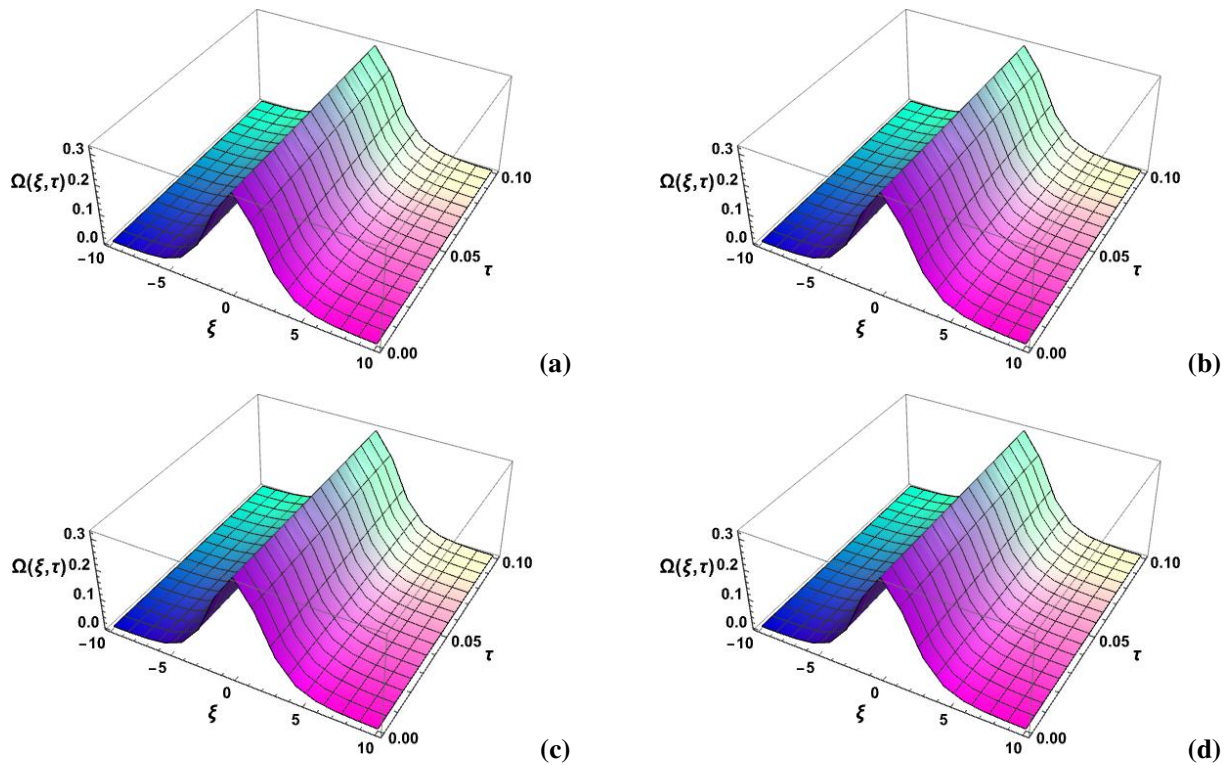
Figure 1. 3D plots of the solution \Omega(\xi, \tau) at Example 1 Generated via Laplace New Iterative Method (LNIM): (a) \alpha = 0.90 , (b) \alpha = 0.95 , (c) \alpha = 1 and with (d) the exact solution corresponding. The horizontal axis is the spatial variable \xi and time variable \tau , and the vertical axis is the solution \Omega(\xi, \tau) . Good agreement between approximate solutions and the exact solution demonstrates the accuracy of the proposed LNIM.
