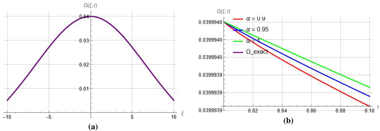
Figure 6. (a) The 2D graph of the \Omega for any value of \xi and \alpha = 0.90, 0.95, 1 , Exactsolution (b) the 2D graph of the \Omega for any value of \tau and \alpha = 0.90, 0.95, 1 , Exactsolution
