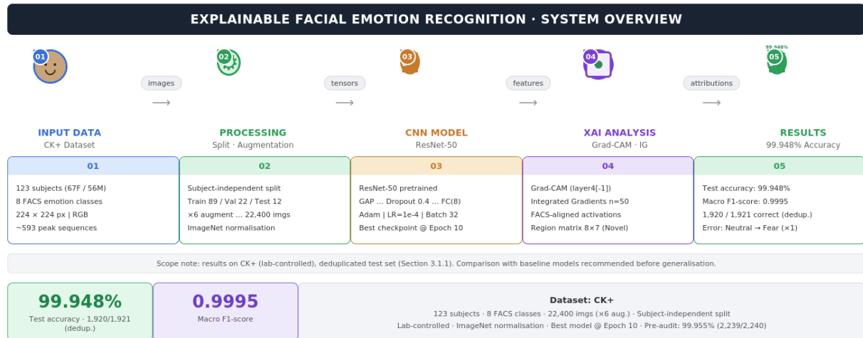
Figure 1. System overview of the proposed explainable FER framework. The pipeline proceeds from CK+ input data through data processing, ResNet-50 fine-tuning, dual XAI analysis
