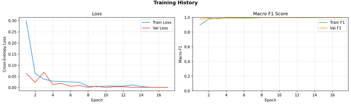
Figure 3. Training history: loss curves (left) and macro F1-score curves (right).
