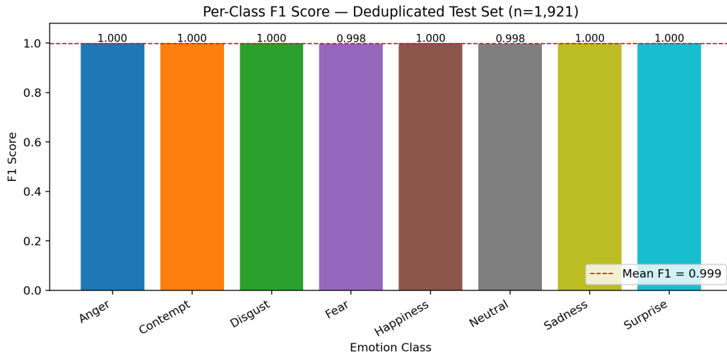
Figure 5. Per-class F1-score on the test set (deduplicated, n = 1,921 ).
