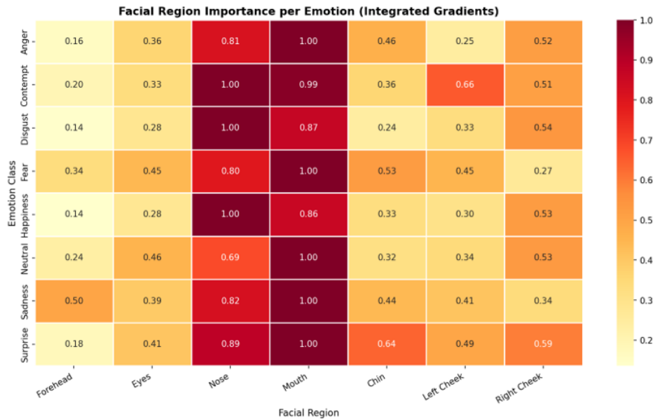
Figure 11. Facial Region Importance Matrix derived from Integrated Gradients
