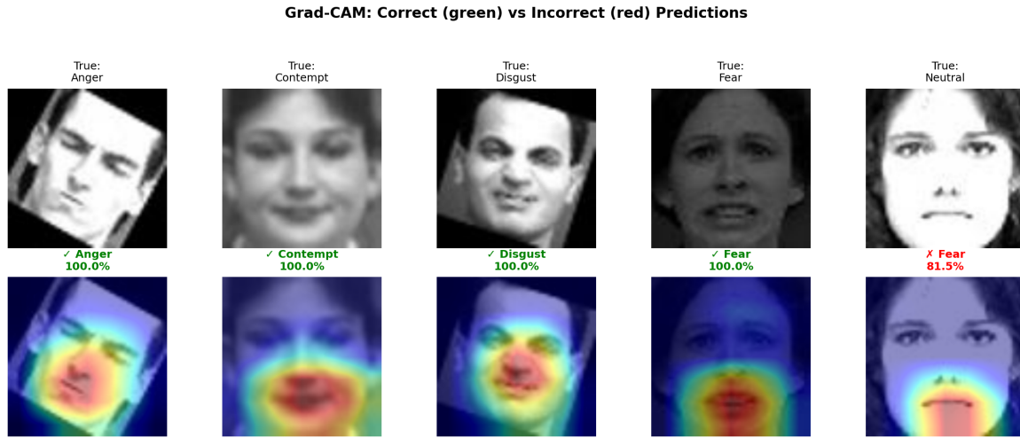
Figure 9. Grad-CAM: four correct predictions (green ✓, columns 1–4, one per class shown) vs. the single incorrect prediction in the entire test set (red ✗, column 5).
