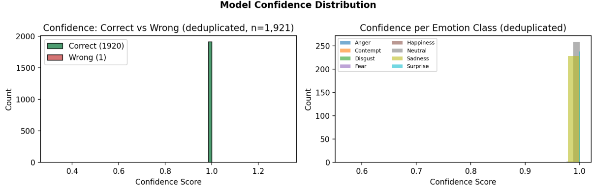
Figure 6. Model confidence distributions. Left: correctly vs. incorrectly classified samples. Right: per-class confidence histograms (deduplicated test set, n = 1,921 ; see Section 3.1.1).
