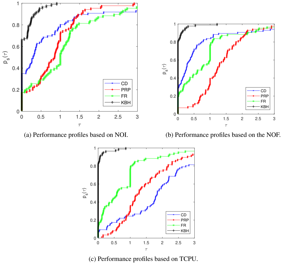
Figure 1. Performance profiles of the KBH method compared to the CD, PRP and FR methods.
