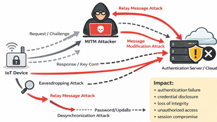
Figure 8. MITM attack schema
