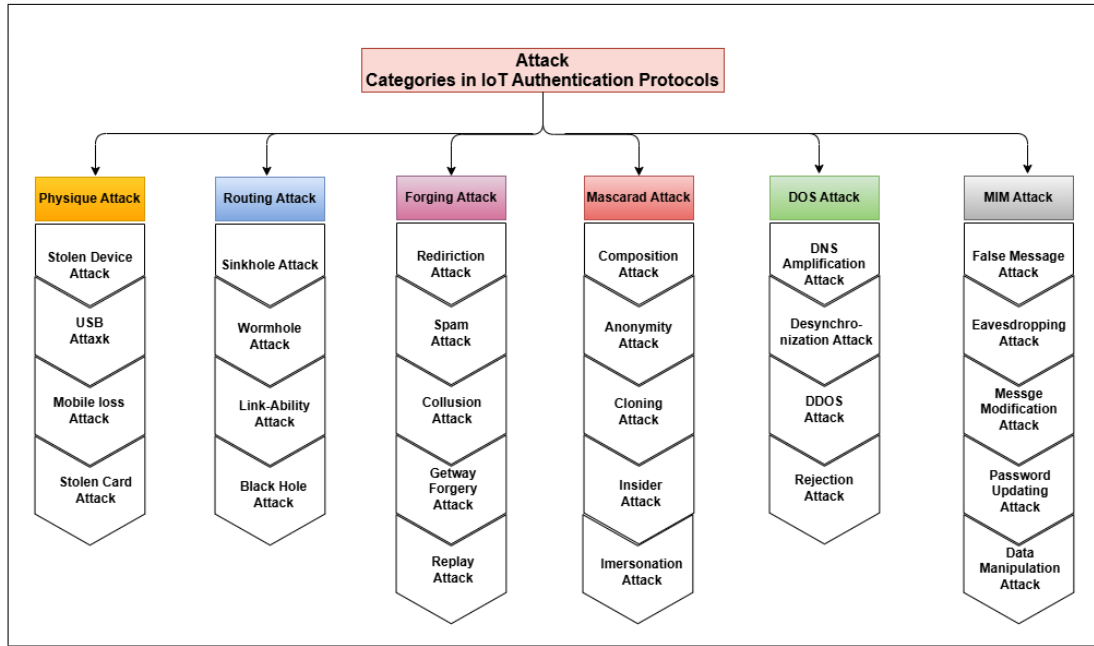
Figure 3. Mechanisms used by authentication protocols
