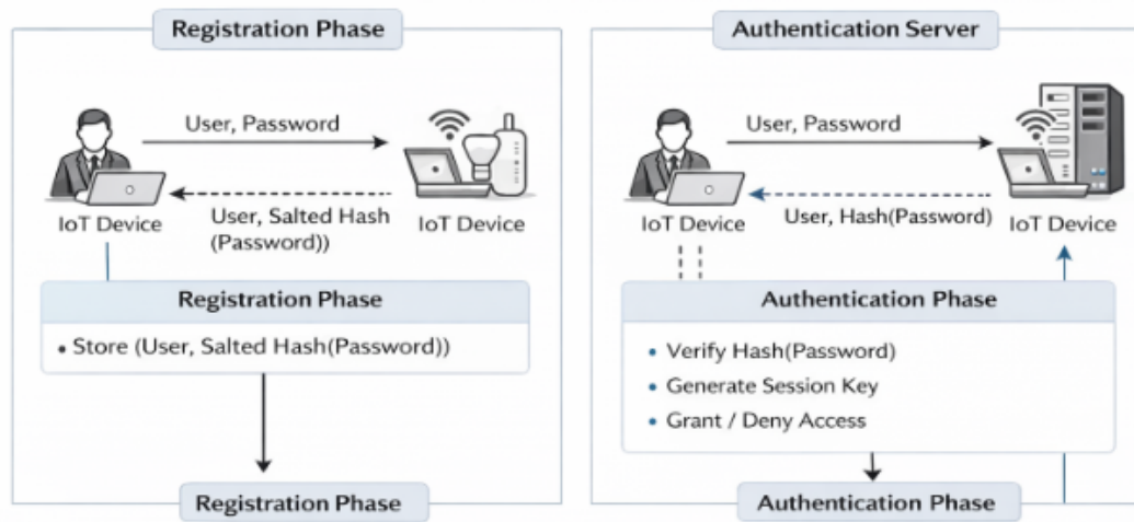
Figure 10. Authentication methods
