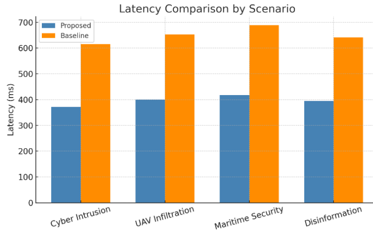
Figure 3. Latency comparison for threat response scenarios
