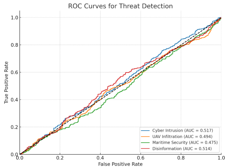
Figure 2. Receiver operating characteristic curves for threat detection
