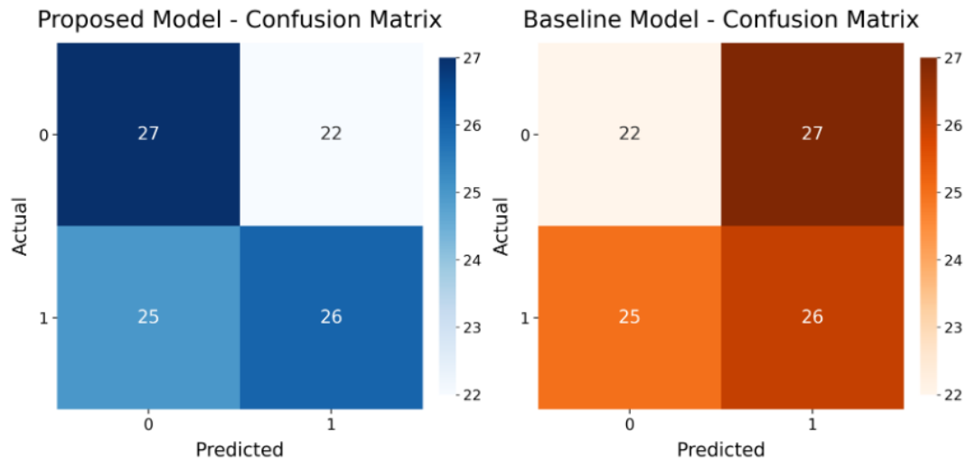
Figure 4. Comparative confusion matrices for threat detection
