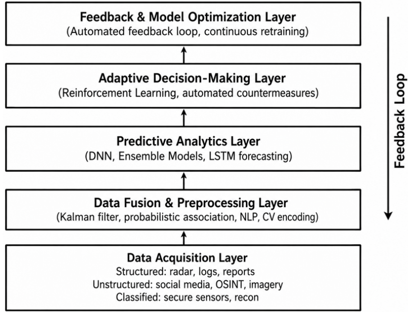
Figure 1. Proposed AI-driven situational intelligence architecture
