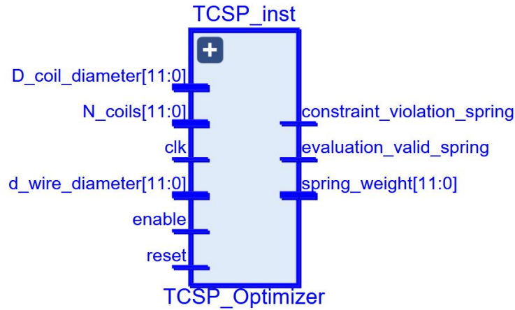
Figure 14. TCSP_Optimizer instance on FPGA.
