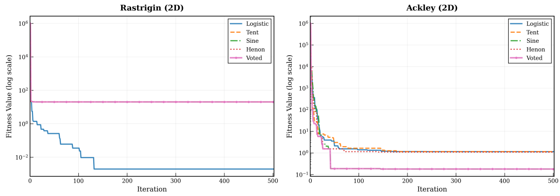
Figure 9. Convergence curves - 2D multimodal functions.
