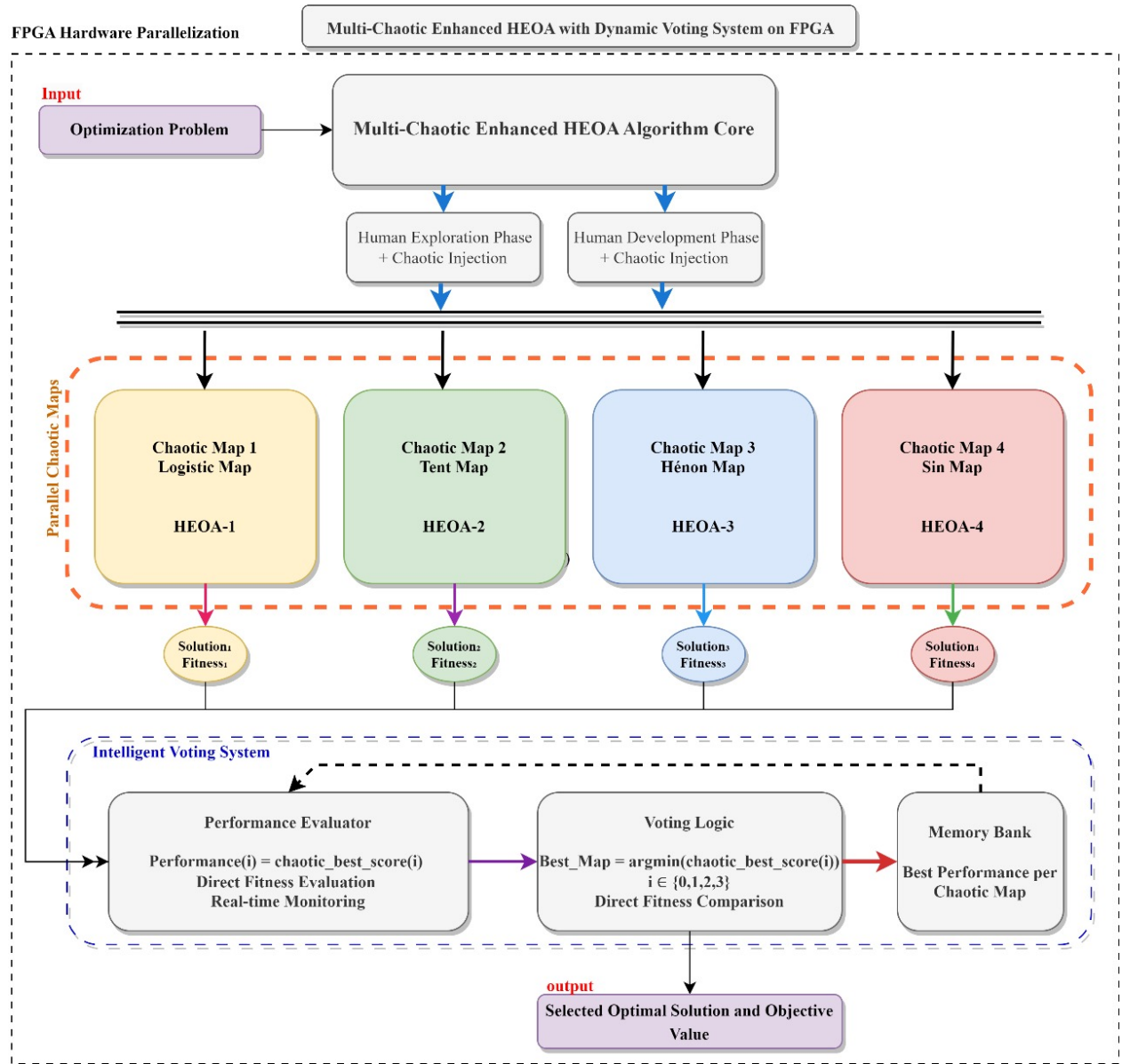
Figure 3. Overall architecture of the MC-HEOA framework with four parallel chaotic maps and dynamic voting system on FPGA.
