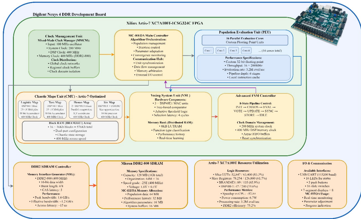
Figure 4. Modular FPGA architecture for MC-HEOA implementation. The architecture integrates four specialized units with a pipeline system for parallel processing and coordinated management of the selection mechanism.
