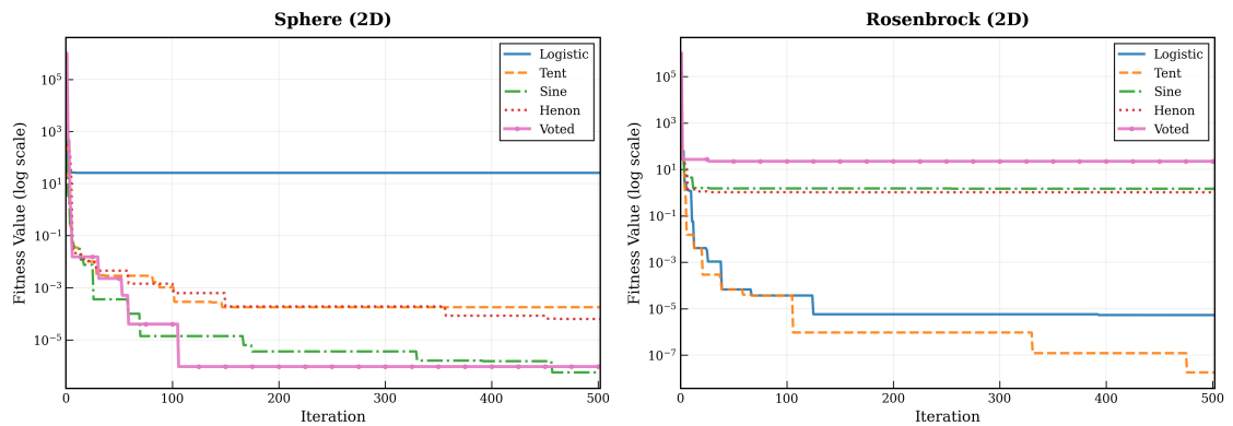
Figure 8. Convergence curves - 2D unimodal functions.
