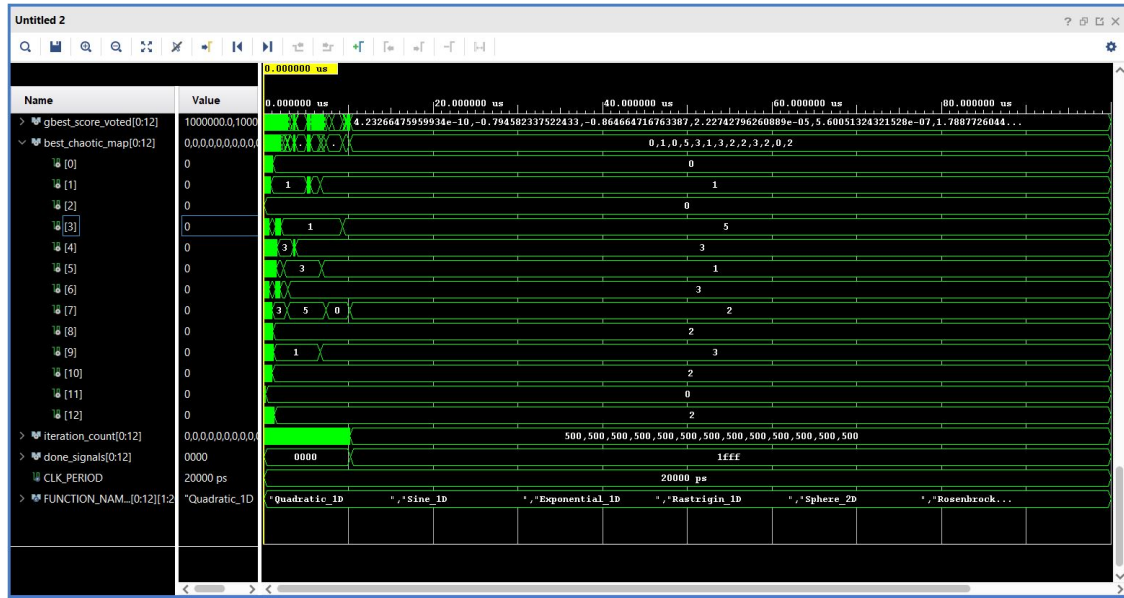
Figure 6. Adaptive selection of chaotic maps.
