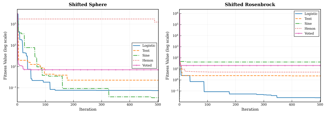
Figure 10. Convergence curves - Shifted unimodal functions.
