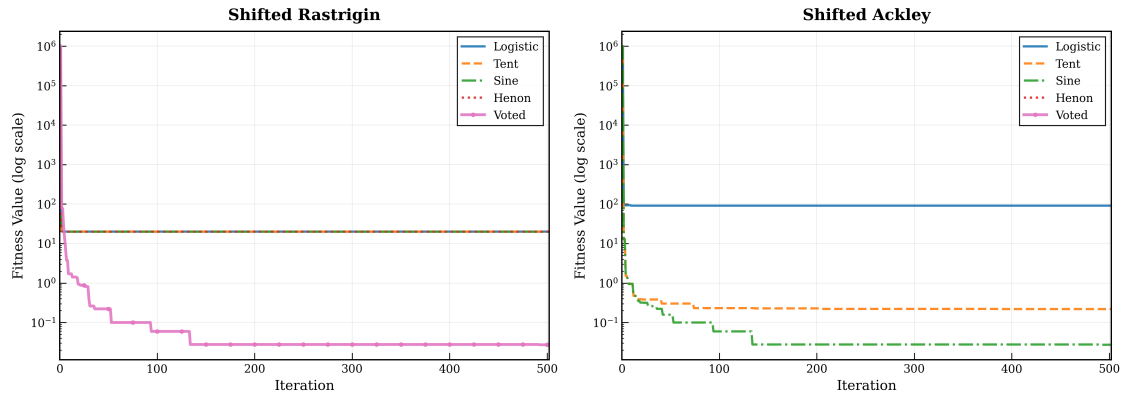
Figure 11. Convergence curves - Shifted multimodal functions.
