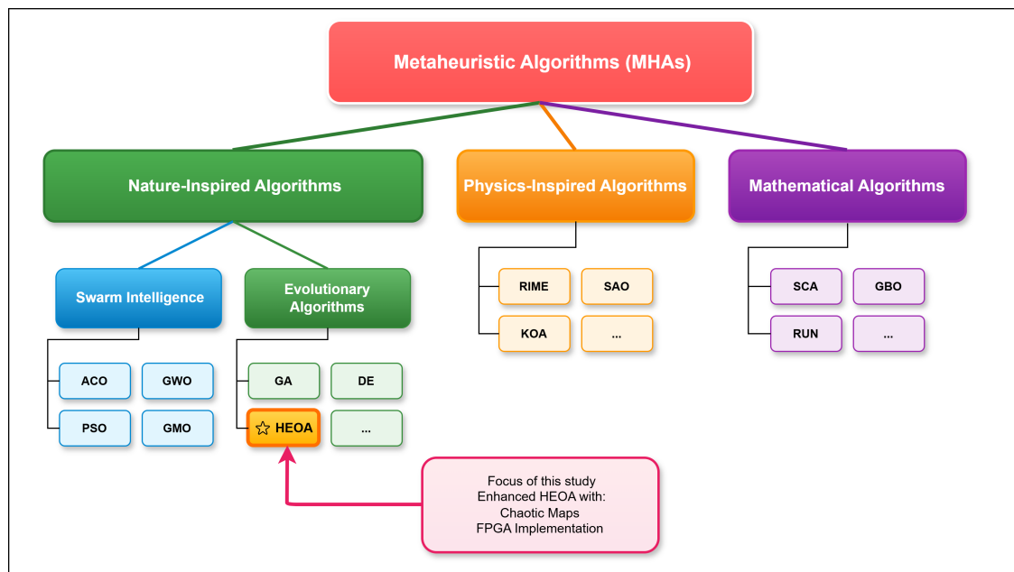
Figure 1. Hierarchical classification of metaheuristic optimization algorithms
