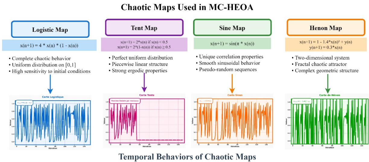
Figure 2. Temporal behaviors of the four chaotic maps over 150 iterations.
