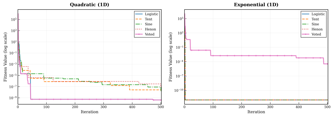
Figure 7. Convergence curves - 1D functions.
