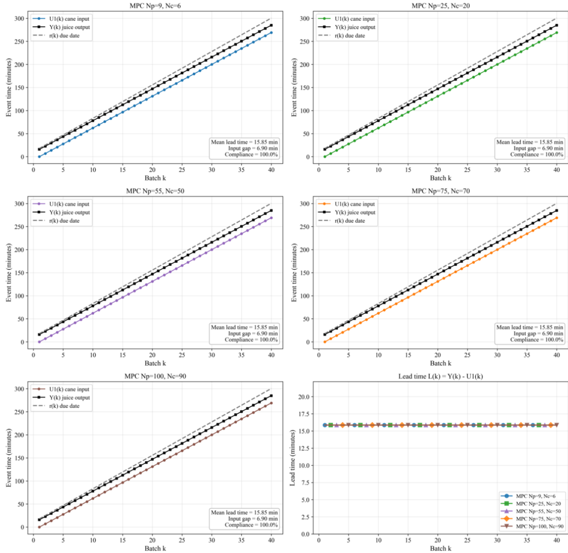
Figure 2. Sugarcane entry time U_1(k) , juice completion time Y(k) , and output due date r(k) across five MPC horizon pairs; the bottom-right panel displays the lead time for each configuration (Model M1, nominal parameters)
