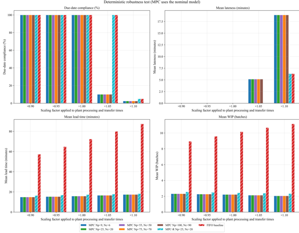
Figure 11. Due-date compliance, average tardiness, average lead time, and average WIP under deterministic robustness testing
