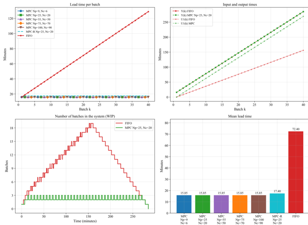
Figure 6. Comparison of MPC and FIFO: per-batch lead time, entry and completion times, number of batches in the system (WIP), and average lead time
