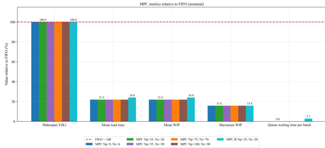
Figure 7. MPC and MPC-R performance metrics relative to FIFO (FIFO = 100) under nominal conditions
