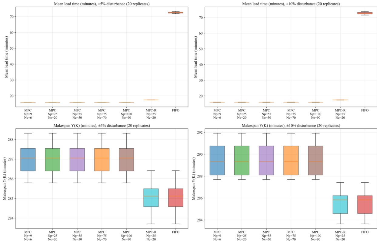
Figure 13. Distribution of average lead time (top) and makespan (bottom) under stochastic perturbations of \pm 5\% (left) and \pm 10\% (right)
