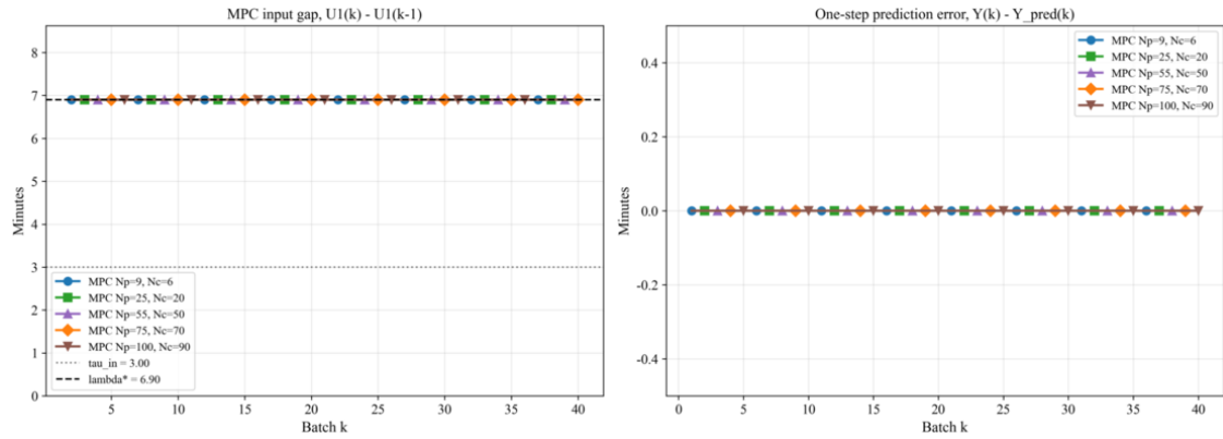
Figure 3. MPC input spacing U_1(k) - U_1(k - 1) and one-step prediction error under nominal conditions
