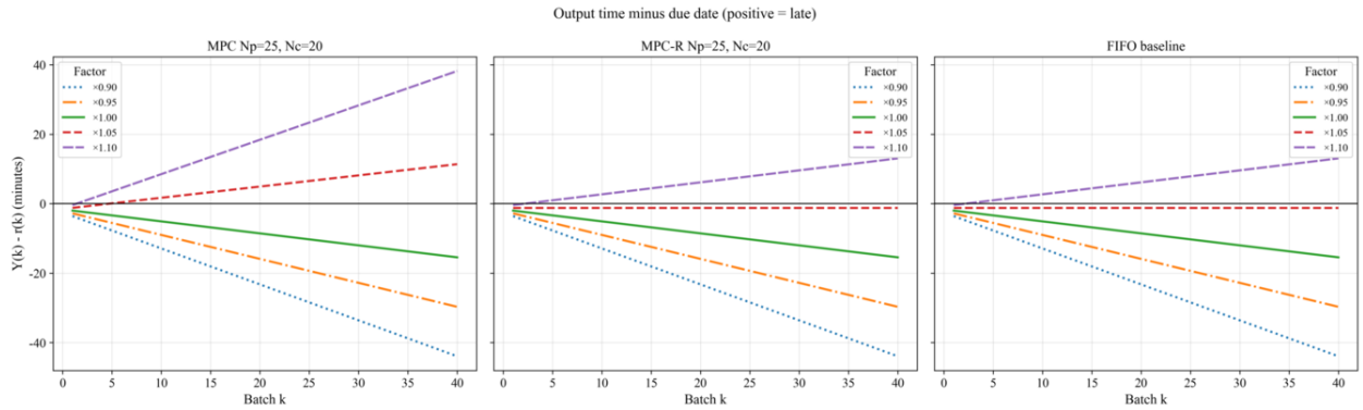
Figure 12. Difference between exit time and due date, Y(k) - r(k) , for nominal MPC, MPC-R, and FIFO across five perturbation factors (positive values indicate tardiness)
