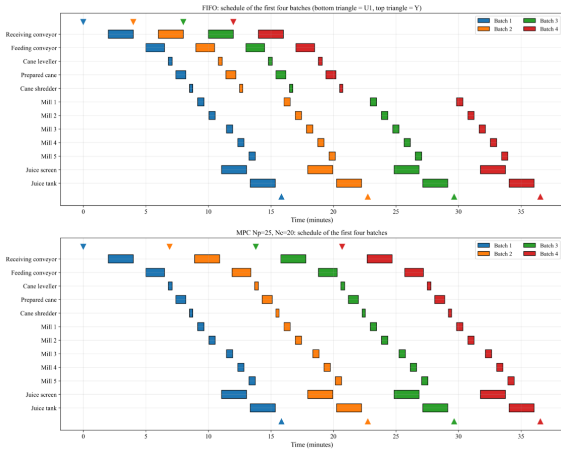
Figure 8. Gantt chart of the first four batches under FIFO (top) and MPC with N_p = 2 (bottom)
