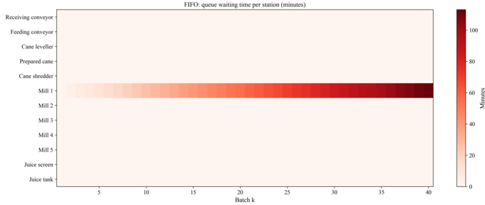
Figure 5. Distribution of FIFO queue waiting times by station and by batch
