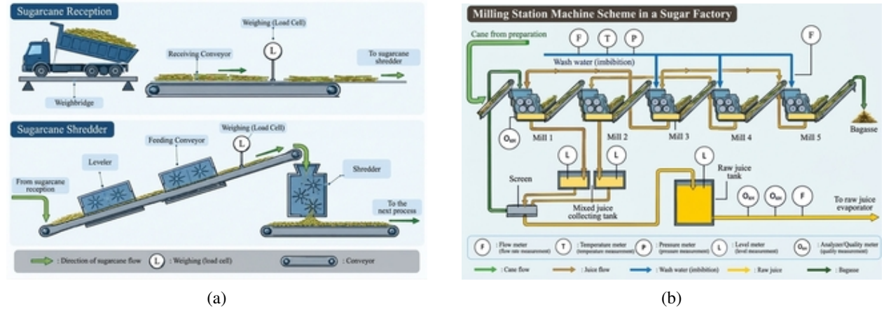
Figure 1. (a) Preparation station and (b) Milling station [12]
