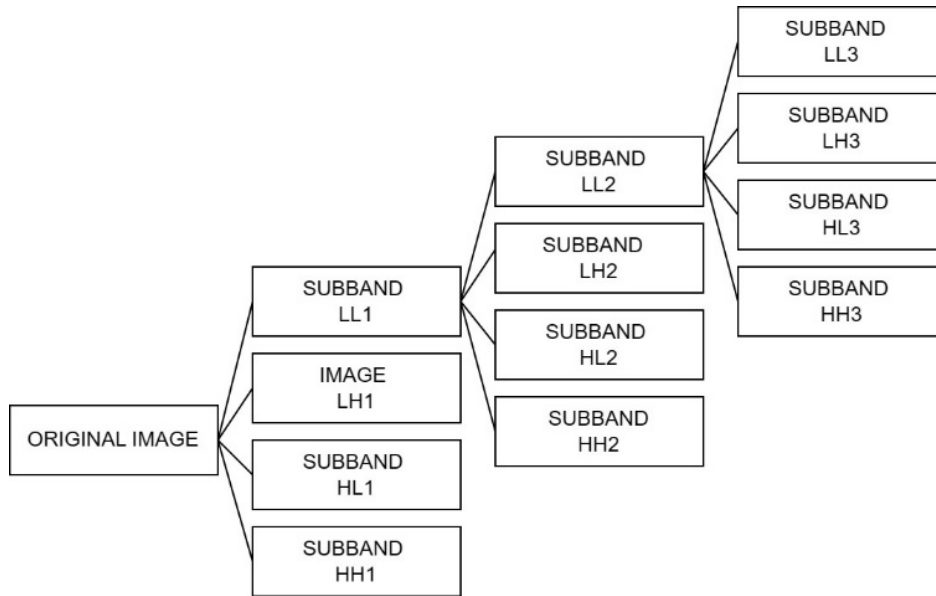
Figure 3. Illustration of the 3-level Discrete Wavelet Transform.
