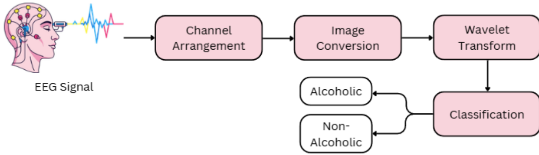
Figure 1. The proposed methods for EEG classification into Alcoholic and Non-Alcoholic. The pipeline consists of four stages: (1) Channel Arrangement, in which the raw multichannel EEG signal is organized into a channel-by-sample matrix; (2) Image Conversion, in which the matrix is rescaled to an 8-bit grayscale image via Min-Max scaling (Equation (1)); (3) Wavelet Transform, in which the resulting image is decomposed via 2D-DWT and statistical features are extracted from the sub-bands; and (4) Classification, in which the extracted features are fed into ML/DL classifiers to produce the Alcoholic / Non-Alcoholic decision.
