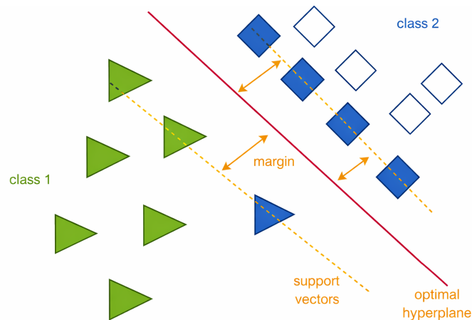
Figure 5. Optimal hyperplane in support vector machine (SVM).
