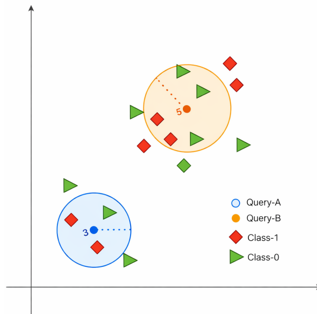
Figure 4. Illustration of k-nearest neighbors (KNN).
