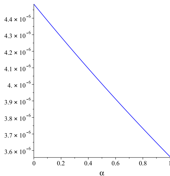
Figure 10. Graph the upper absolute error for example 3.
