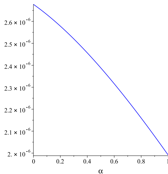
Figure 6. Graph the upper absolute error for example 2.
