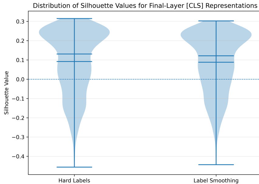
Figure 2. Silhouette coefficient distribution for the [CLS] representations produced by BERT on FinancialPhraseBank using hard label and label smoothing training. The violin plot shows the distribution between paired experiments, with the mean and median shown within each distribution.
