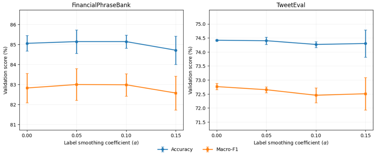
Figure 1. Performance of the validation procedure as a function of label smoothing coefficient in BERT with FinancialPhraseBank and TweetEval. The markers indicate the mean performance of the validation procedure through repeated validation procedures, with the error bars indicating the standard deviation.
