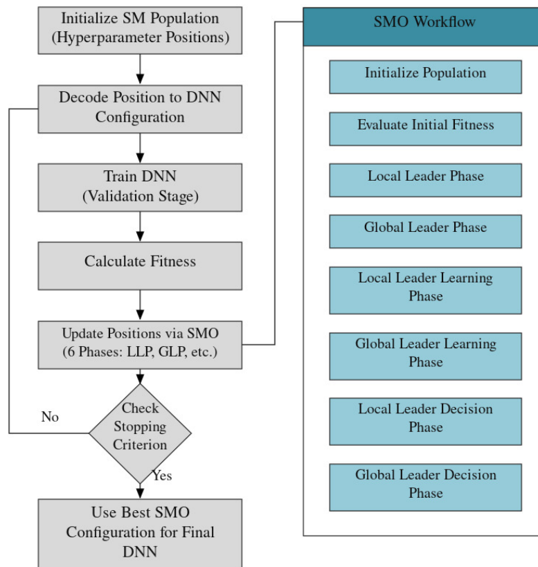
Figure 2. Integration of SMO and DNN
