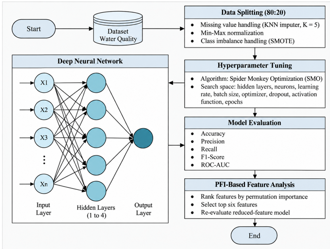
Figure 1. Workflow of the proposed SMO-PFI-DNN framework
