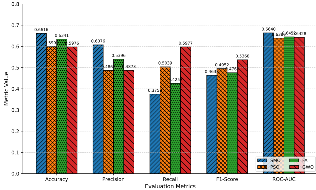
Figure 4. Performance Comparison Across Five Evaluation Metrics
