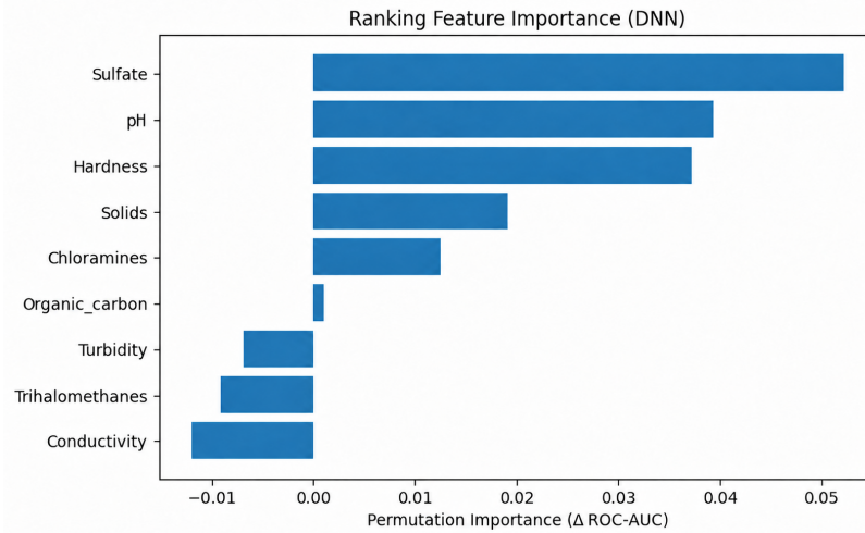
Figure 6. Feature Importance Ranking
