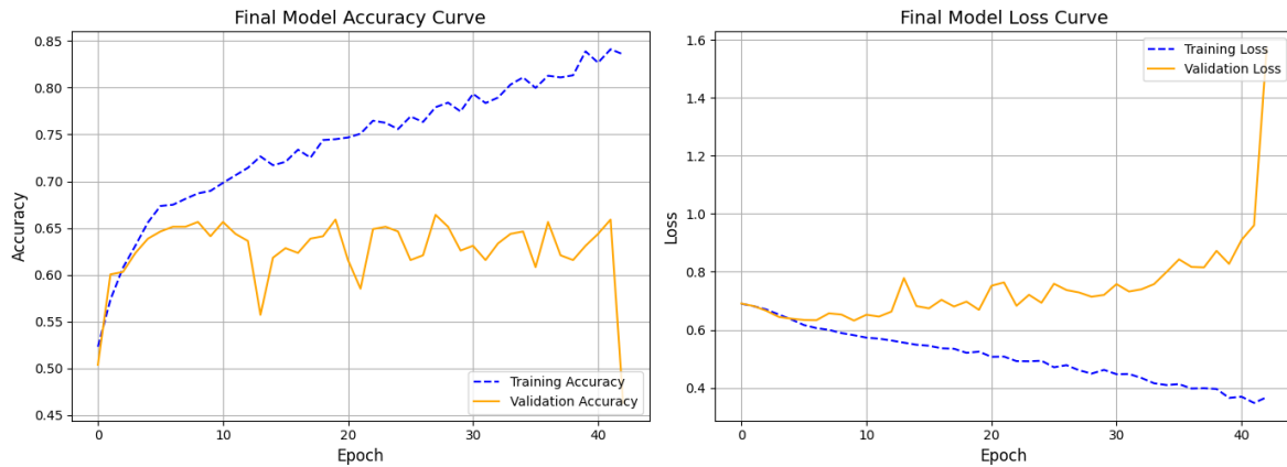
Figure 3. Training and validation accuracy and loss curves of the final SMO-optimized DNN.
