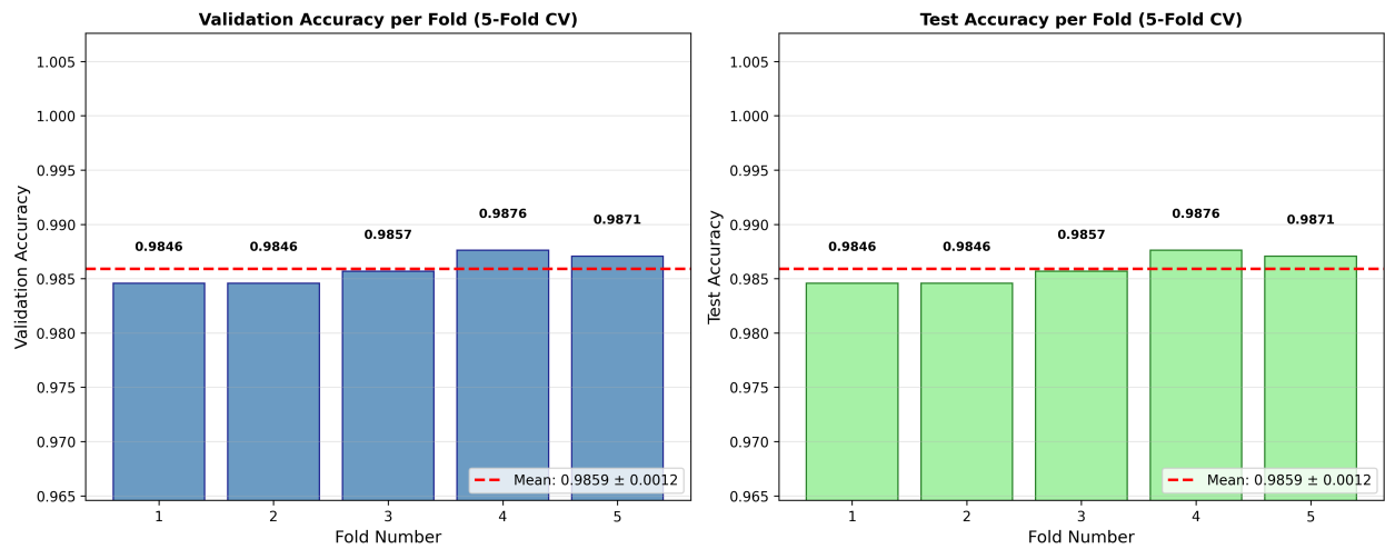
Figure 12. Validation and Test Accuracy per Fold (5-Fold Cross-Validation, Experiment 4).
