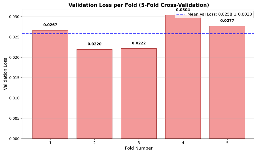
Figure 13. Validation Loss per Fold (5-Fold Cross-Validation, Experiment 4).
