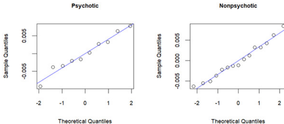
Figure 3. STS Q-Q plots for psychotic and nonpsychotic groups when (r, d) = (2, 0) .
