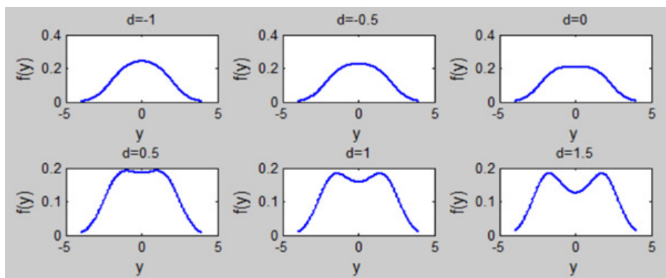
Figure 2. The pdf plots of the STS distribution for certain values of d when r = 4 .
