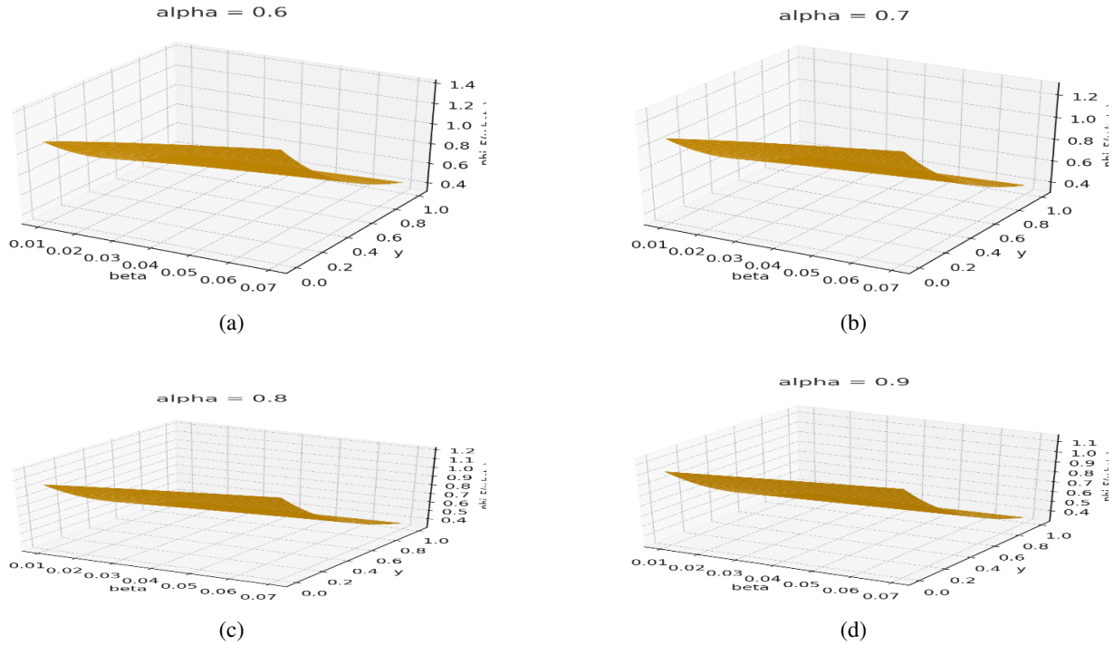
Figure 1. The graph of the solution \phi_5(y, \beta) , and several values \alpha in Example 1 at m = -1.2 in all graphs (a) \alpha = 0.6 , (b) \alpha = 0.7 , (c) \alpha = 0.8 , (d) \alpha = 0.9 .
