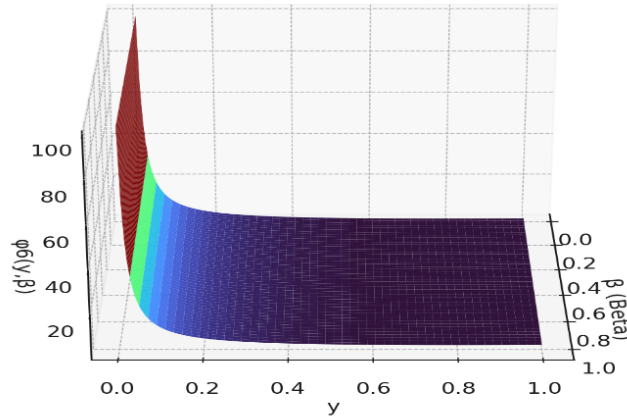
Figure 2. The graph of the solution \phi(y, \beta) of the Example 2.
