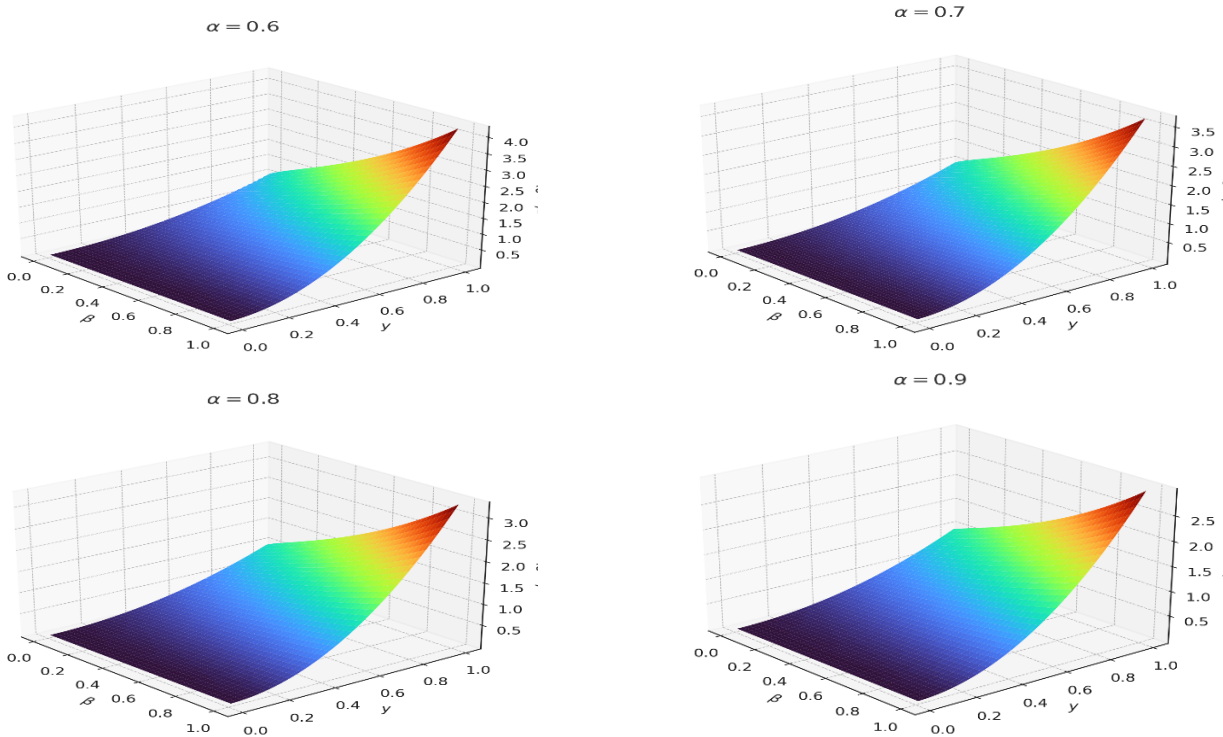
Figure 5. The graph of the solution \phi(y, \beta) of the Example 3.
