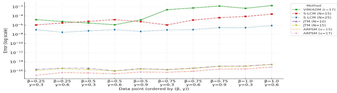
Figure 4. comparison of the different numerical methods
