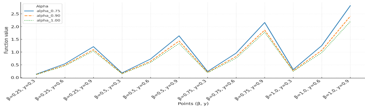
Figure 3. Comparative Analysis of Fractional approximate Solutions at Varying Points
