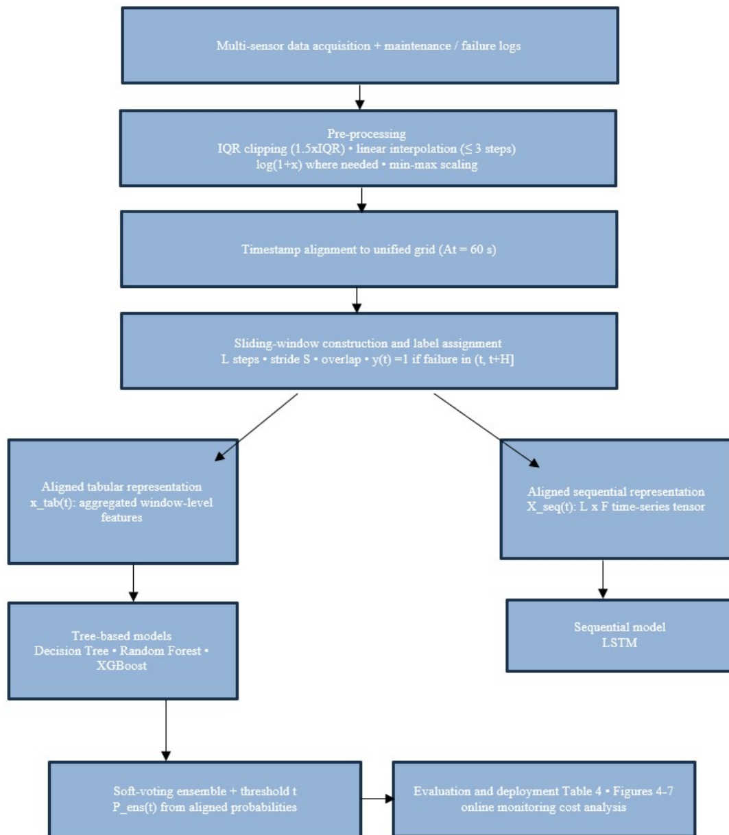
Figure 1. Methodological flowchart of the proposed predictive-maintenance pipeline.
