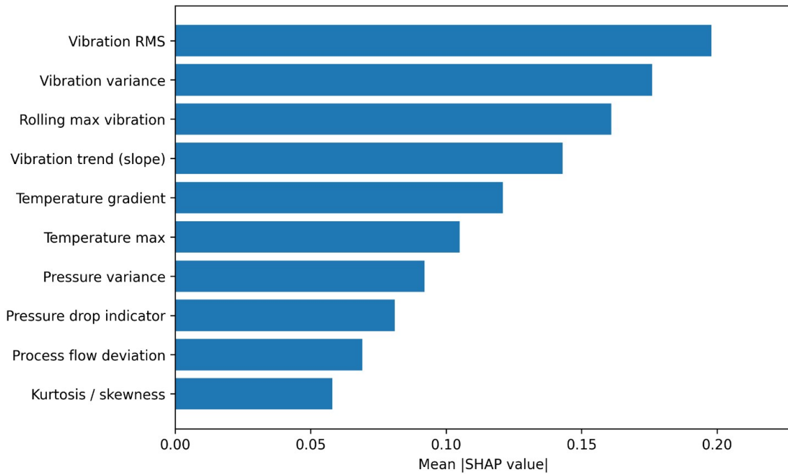
Figure 7. Feature importance ranking for the strongest tabular model (XGBoost).
