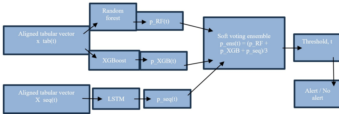
Figure 3. Synchronised ensemble fusion and threshold-based alert generation.
