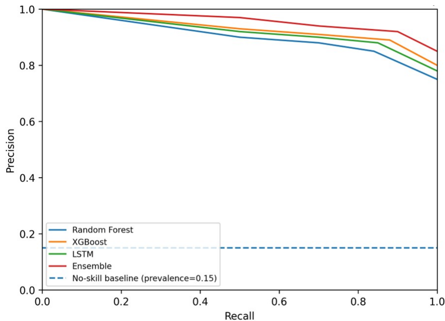
Figure 5. Precision–Recall curves on the held-out time-based test interval for key models and the ensemble.
