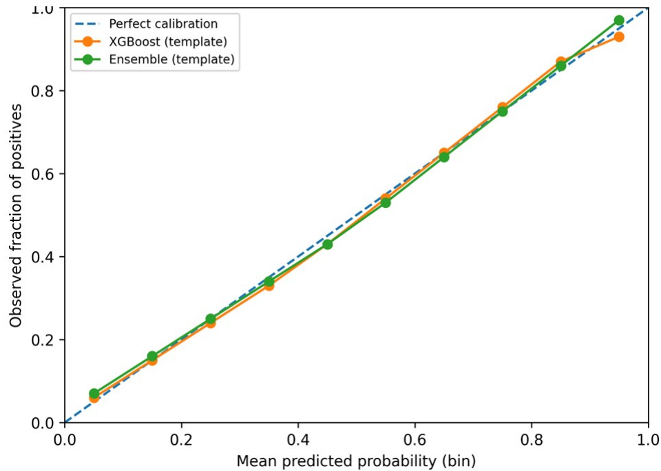
Figure 6. Calibration curves (reliability diagrams) on the held-out time-based test interval for the ensemble and the strongest tabular model.
