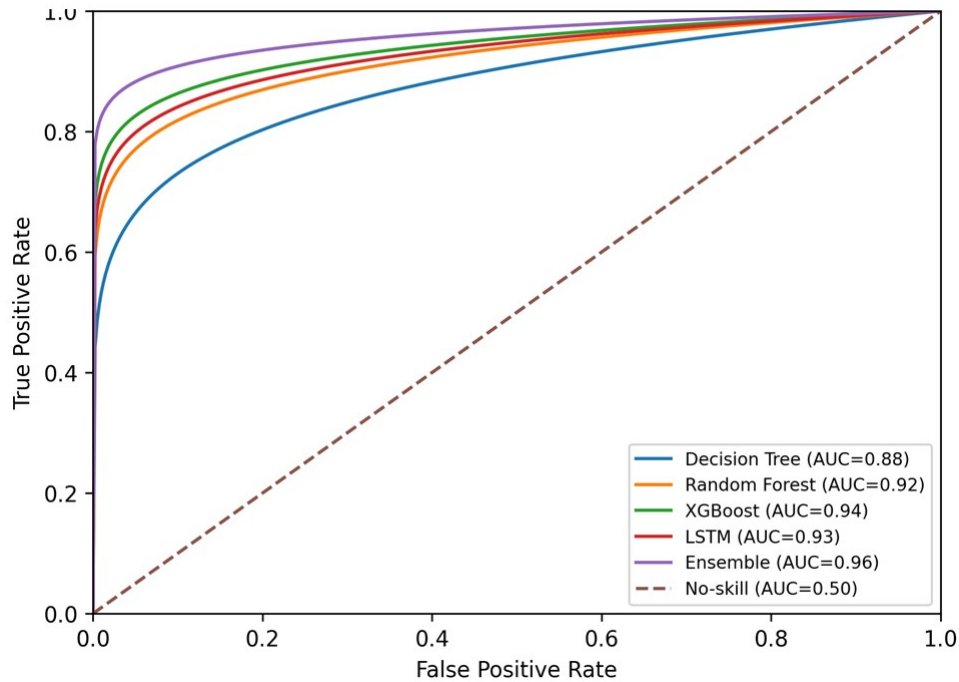
Figure 4. ROC curves on the held-out time-based test interval for the strongest standalone models and the ensemble.
