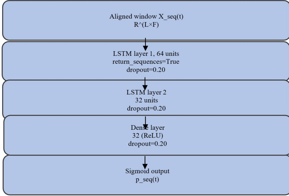
Figure 2. Sequential modelling branch used for time-series failure prediction.
