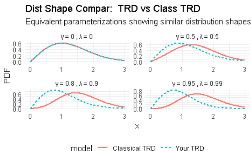
Figure 7. Comparison of Probability Density Functions: Proposed TRD vs. Classical TRD Parameterization.
