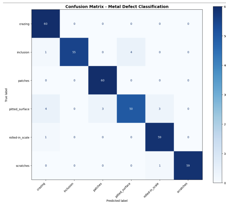
Figure 8. Resnet50 confusion matrix Result after testing on 360 images
