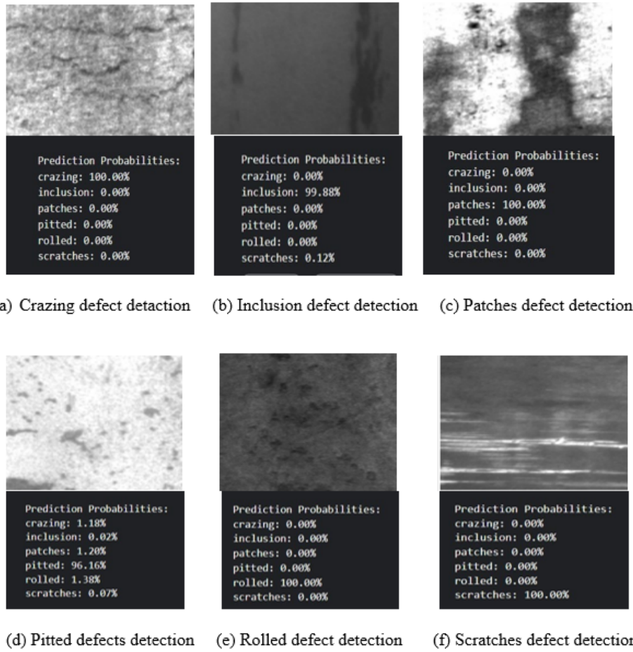
Figure 5. Six tested samples for the six different defects from the NEU-DET dataset and their corresponding detection results by ResNet50V2 model
