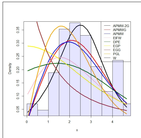
Figure 7. estimated densities with histogram for data set 1.
