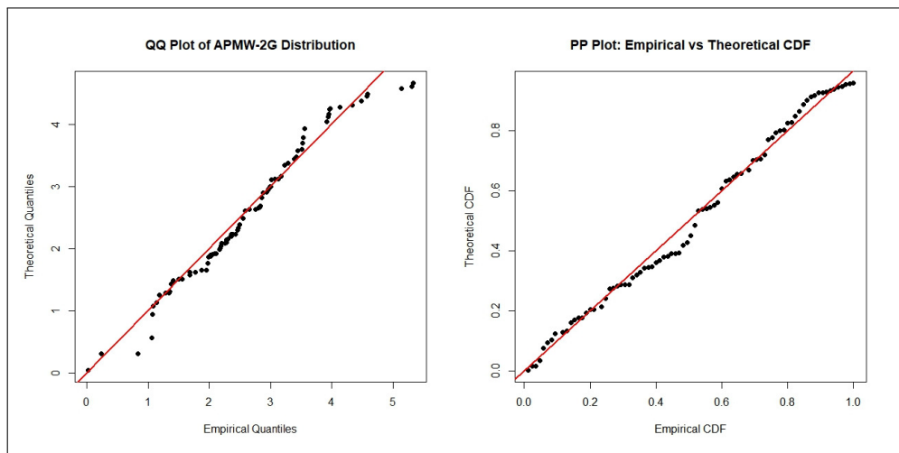
Figure 8. (a)QQ-plot; (b) PP-plot of APMW-2G distribution for data set 1.
