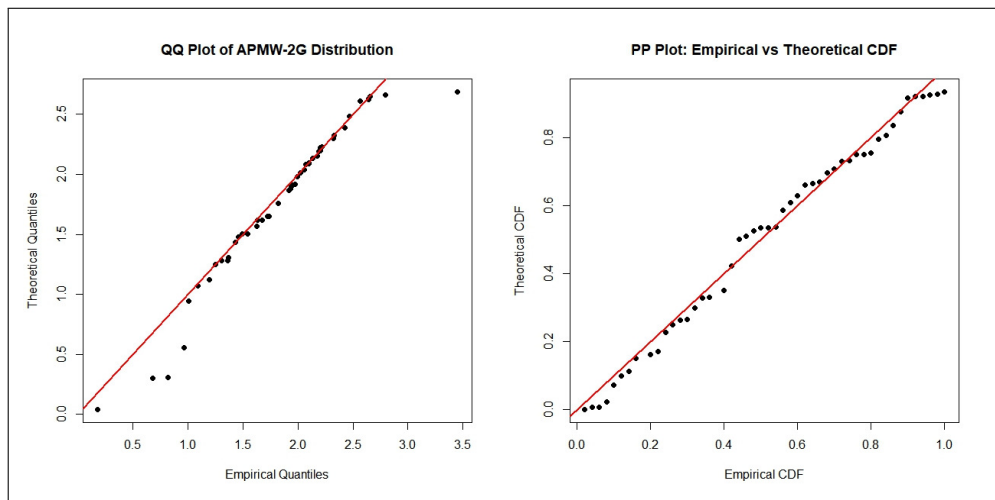
Figure 11. (a)QQ-plot; (b) PP-plot of APMW-2G distribution for the progressive type II censored sample to data set 1.
