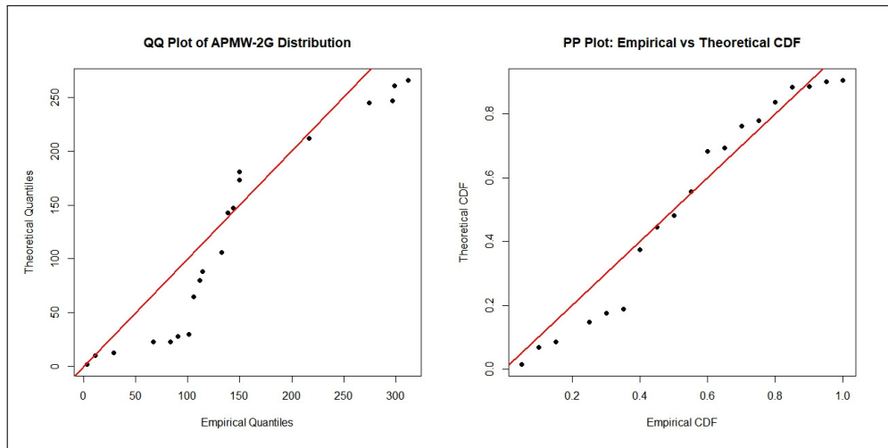
Figure 17. (a)QQ-plot; (b) PP-plot of APMW-2G distribution for the progressive type II censored sample to data set 2.
