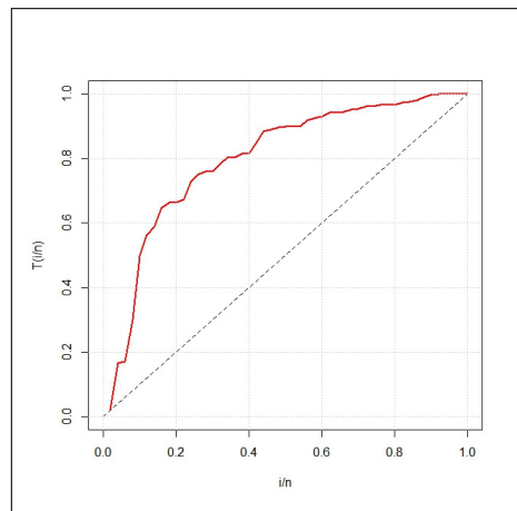
Figure 9. TTT plot for the progressive type II censored sample to data set 1
