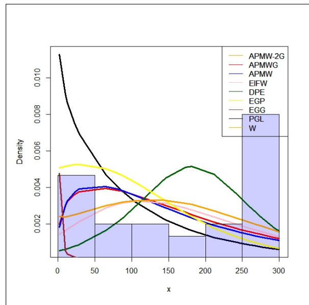
Figure 13. estimated densities with histogram for data set 2.
