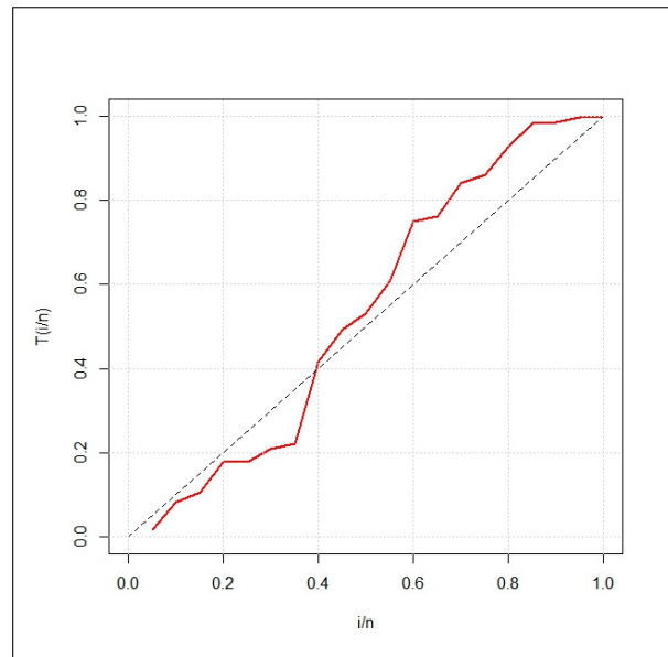
Figure 15. TTT plot for the progressive type II censored sample to data set 2
