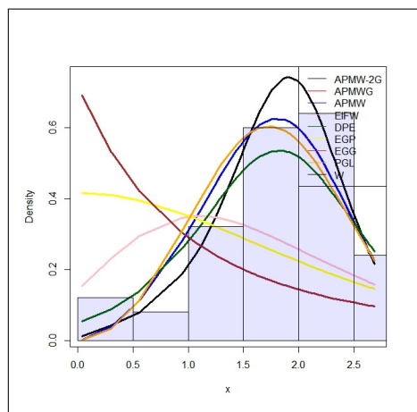
Figure 10. estimated densities with histogram for the progressive type II censored sample to data set 1.
