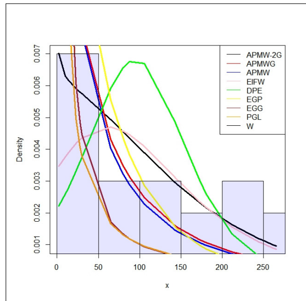
Figure 16. estimated densities with histogram for the progressive type II censored sample to data set 1.
