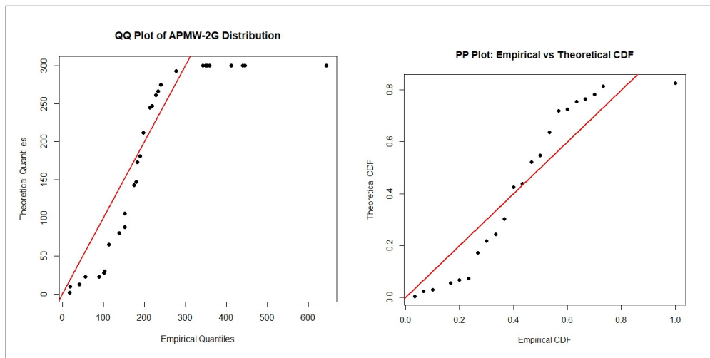
Figure 14. (a)QQ-plot; (b) PP-plot of APMW-2G ditribution for data set 2.
