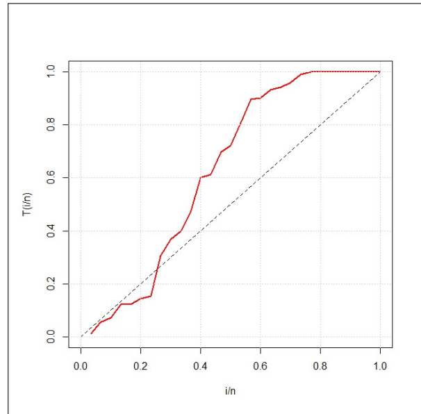
Figure 12. TTT plot for data set 2
