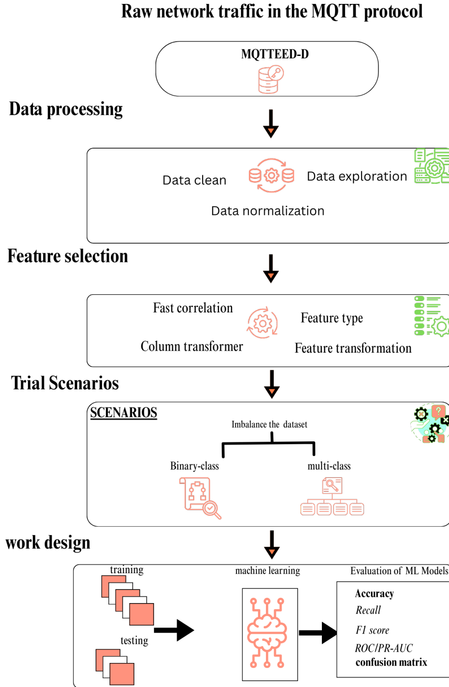
Figure 1. Experimental workflow for IoT threat detection, illustrating data acquisition, preprocessing, feature engineering, model training, and performance evaluation stages.
