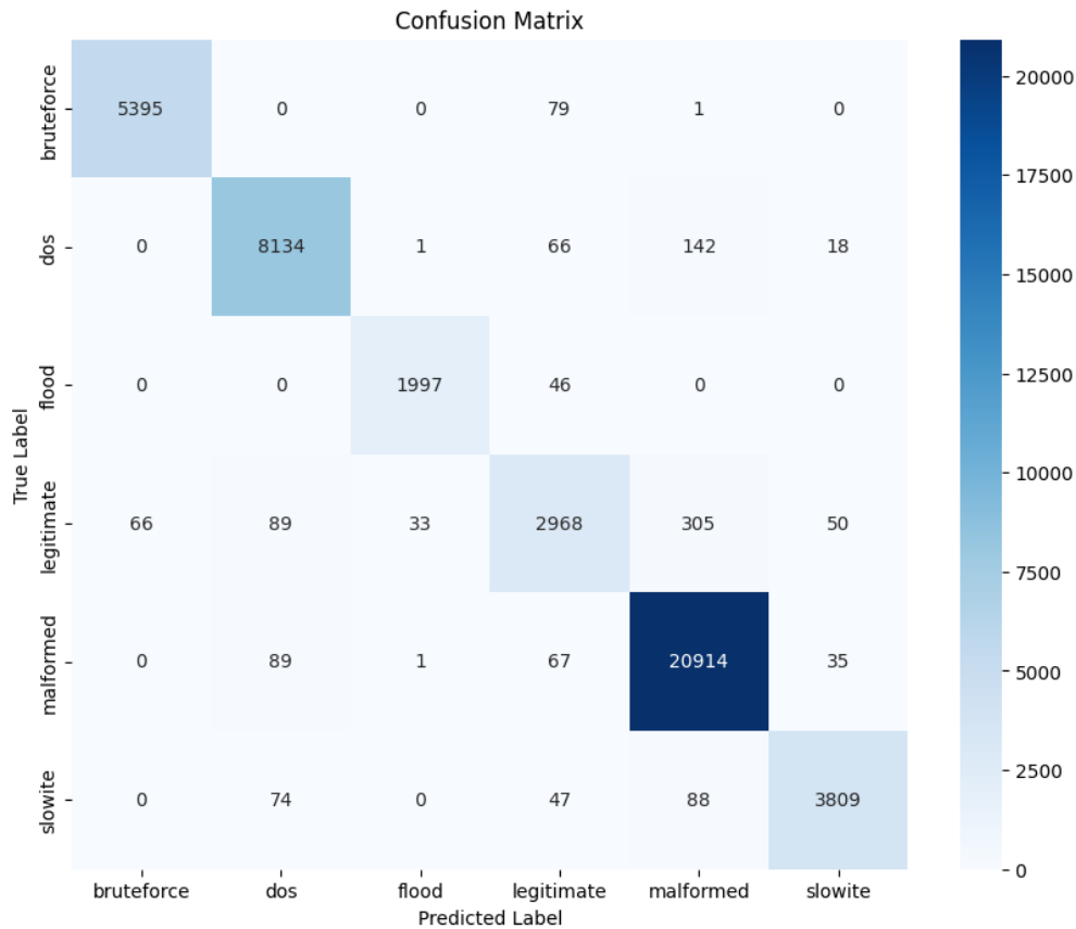
Figure 2. Confusion matrix for the RF classifier. Diagonal cells indicate high true positive rates for attack classes, while off-diagonal values highlight the misclassification of legitimate traffic as the primary source of error.
