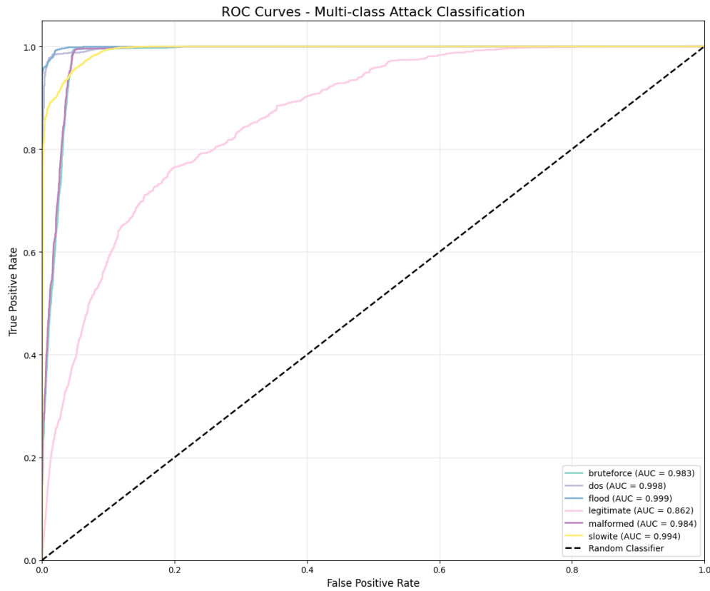
Figure 3. ROC curves for the MLP classifier, illustrating high discriminative power for all attack classes ( AUC > 0.98 ) and a comparatively weaker performance on the legitimate class ( AUC = 0.862 ).
