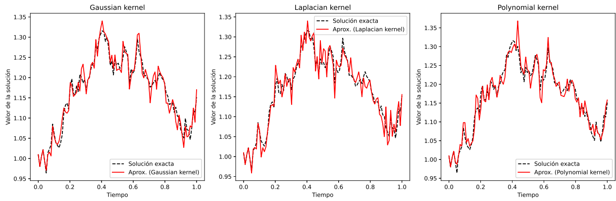
Figure 1. Comparison between the exact trajectory (dashed black line) and RKHS fits using Gaussian, Laplacian, and Polynomial kernels.
