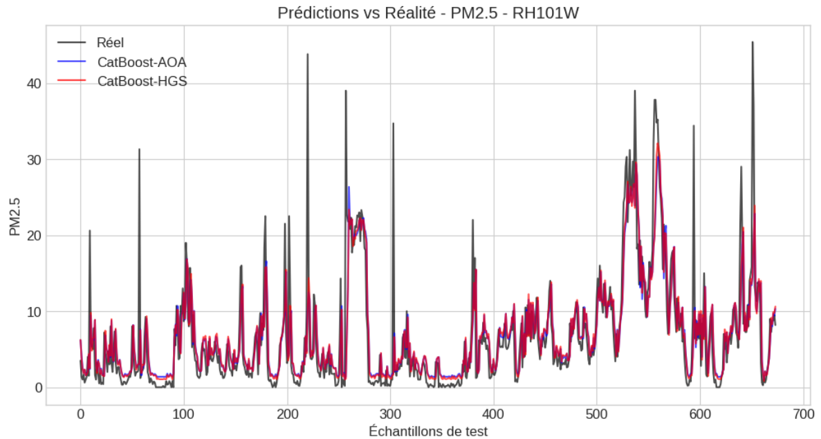
Figure 7. Observed vs. predicted PM2.5 concentrations - RH101W station
