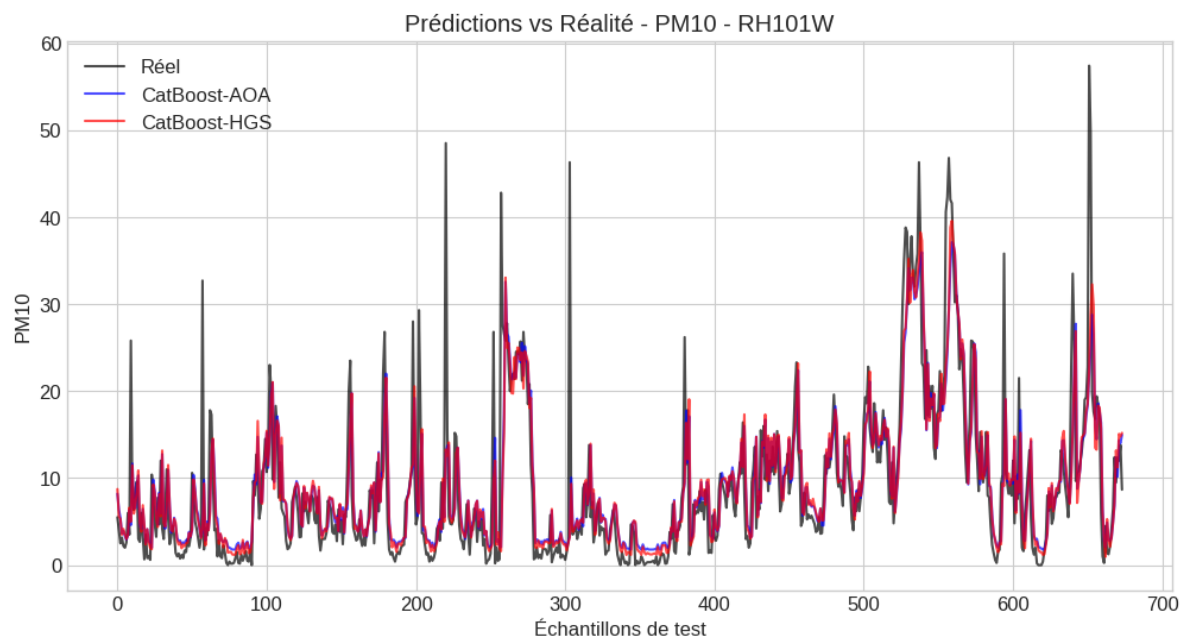
Figure 9. Observed vs. predicted PM10 concentrations - RH101W station
