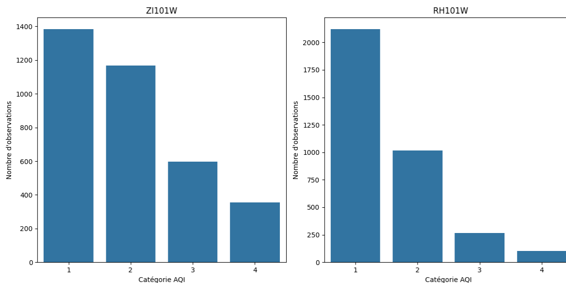
Figure 3. Distribution of air pollutants by station
