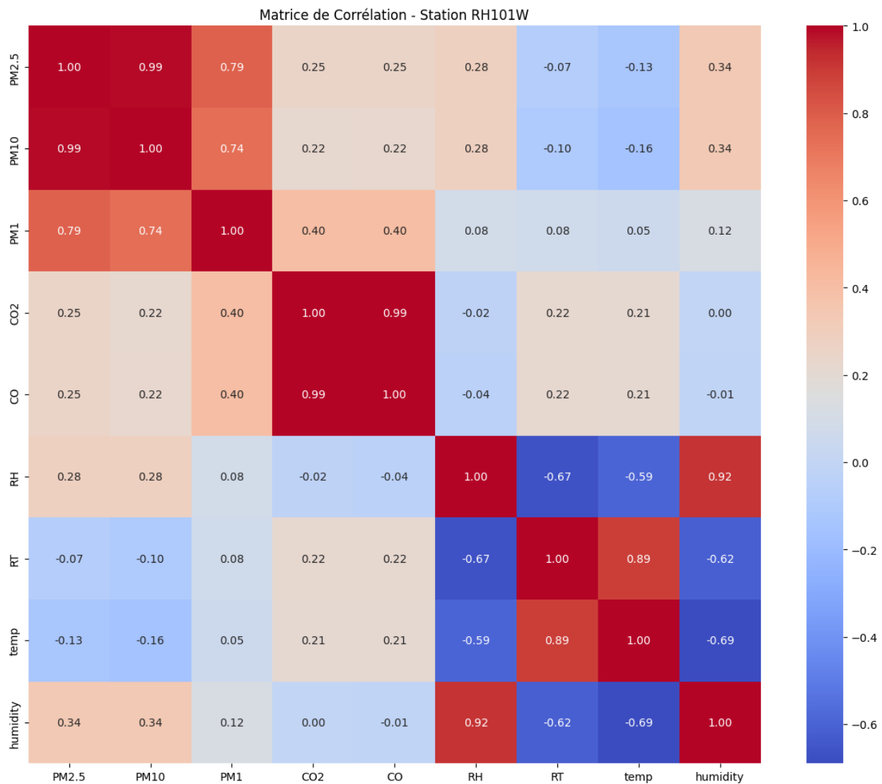
Figure 5. Correlation matrix of air pollutants - station RH101W
