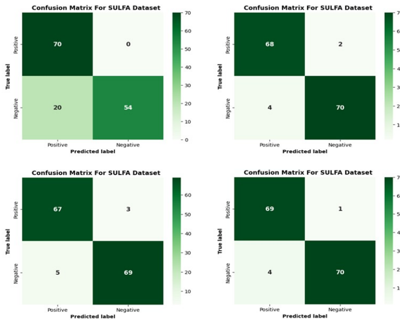
Figure 10. Confusion Matrix for SULFA dataset in Different Configuration Patterns with varying kernel size, learning rate, and conv layers
