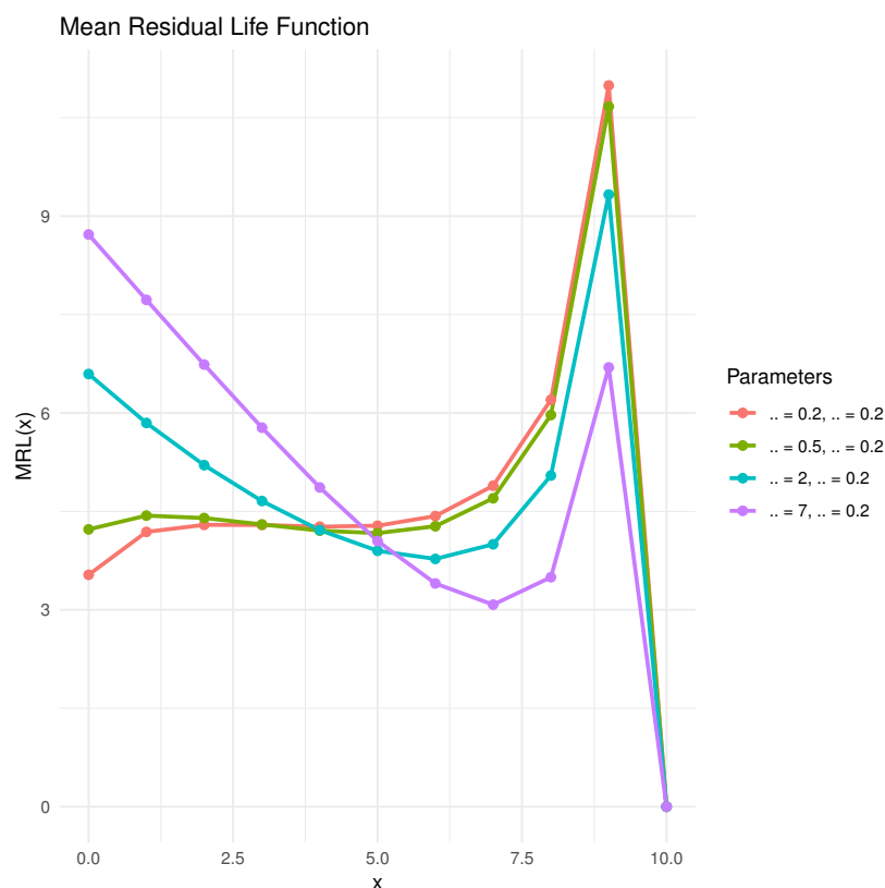
Figure 9. Mean Residual Life ( MRL ) for the LB2 distribution with (\alpha, \beta) are varying parameters.
