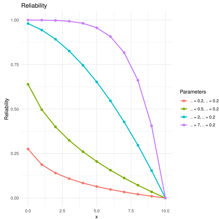
Figure 6. The survival analysis (Reliability Function) of the LB2 various values of the parameters \beta and \alpha .
