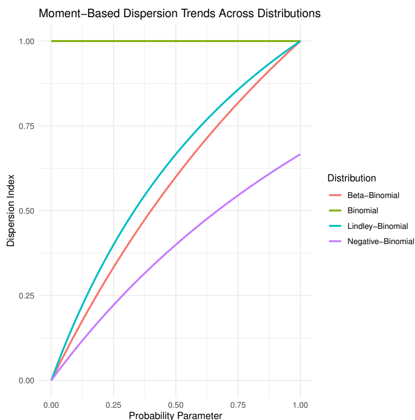
Figure 11. Index of Dispersion for various distributions Across Probability Values.
