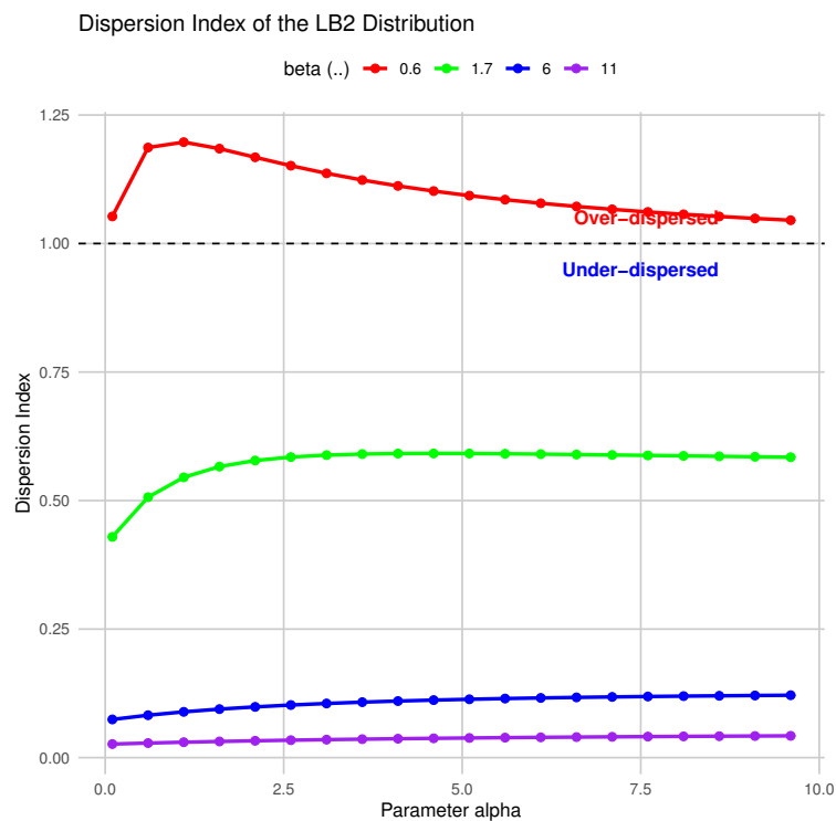
Figure 4. The dispersion of two-parameter Lindley Distribution for various \alpha and constant \beta .
