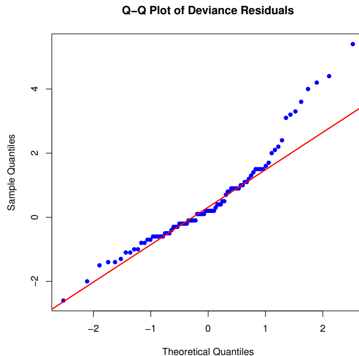
Figure 10. displays the Q-Q plot of residuals.
