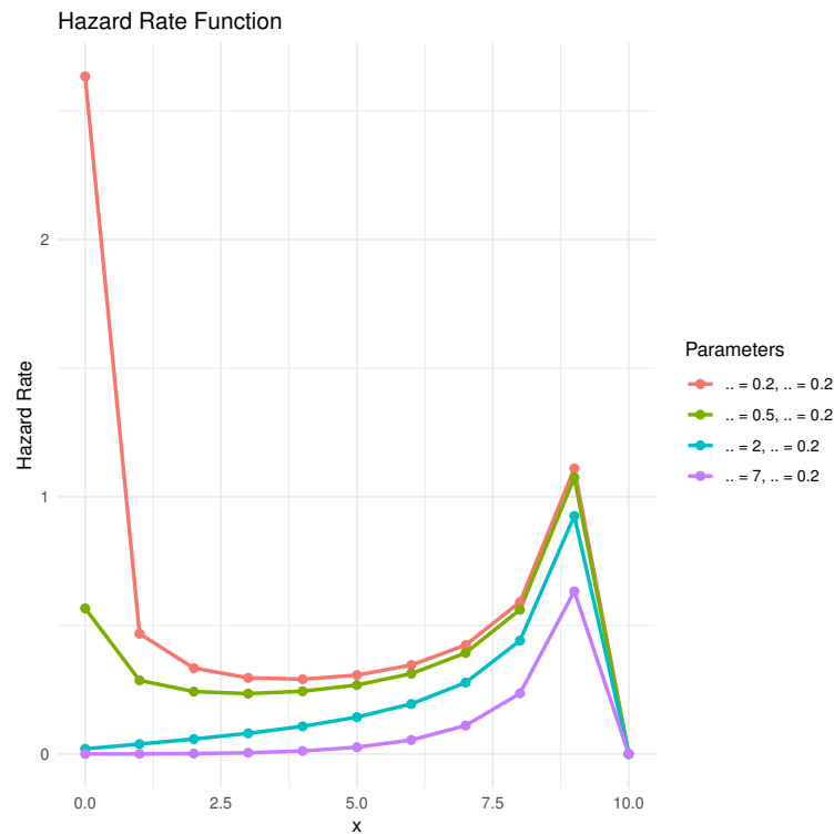
Figure 7. The Hazard Rate Function of the LB2 Distribution.
