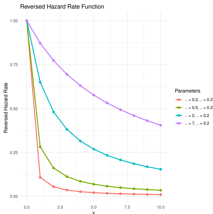
Figure 8. The Reversed Hazard Rate Function for the LB2 Distribution varies with the parameters (\alpha, \beta) .
