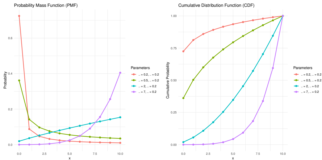
Figure 3. The (PMF) in the left and (cdf) in the right of two-parameter Lindley-Binomial distribution for various \beta and constant \alpha .
