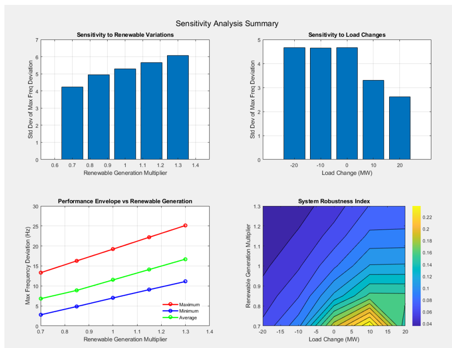
Figure 20. sensitivity analysis
