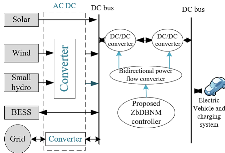
Figure 1. Proposed architecture
