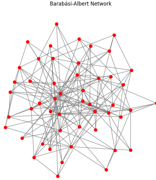
Figure 2. The BA network with N=50 , k=8
