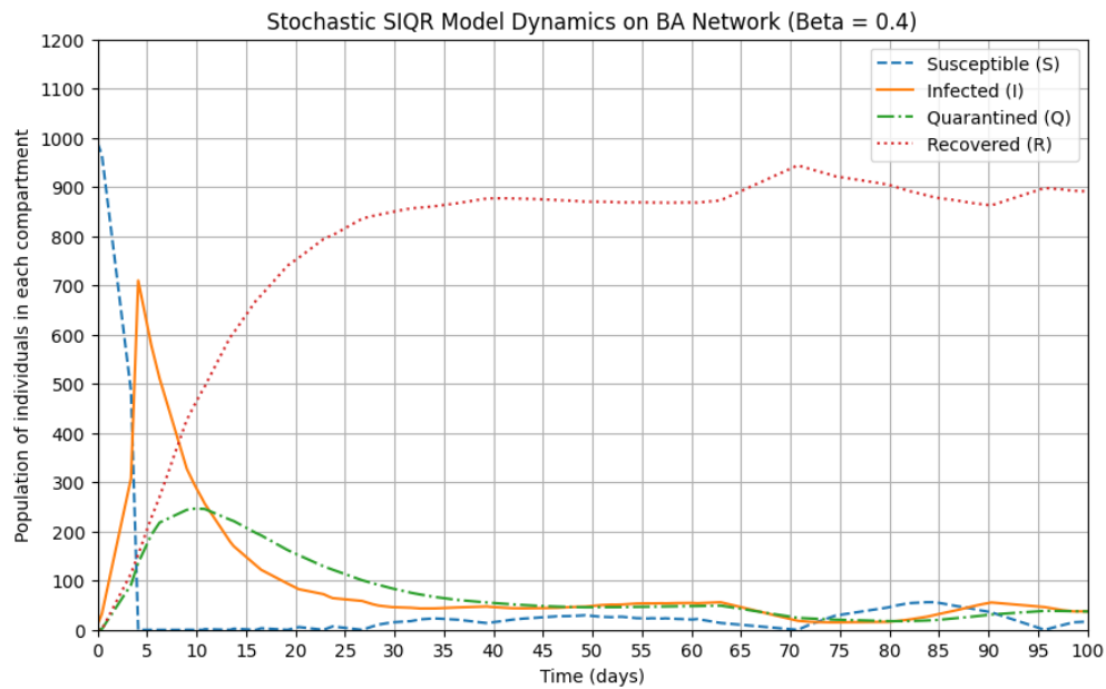
Figure 6. Time evolution of the number of susceptible (S), infected (I), quarantined (Q), and recovered (R) individuals in a Barabási-Albert (BA) network
