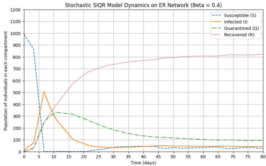
Figure 5. Time evolution of the number of susceptible (S), infected (I), quarantined (Q), and recovered (R) individuals in a Erdős Rénýi (ER) network
