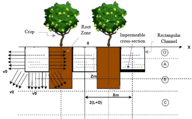
Figure 1. Geometry of Rectangular Channel at Furrow Irrigation Channels with Crops
