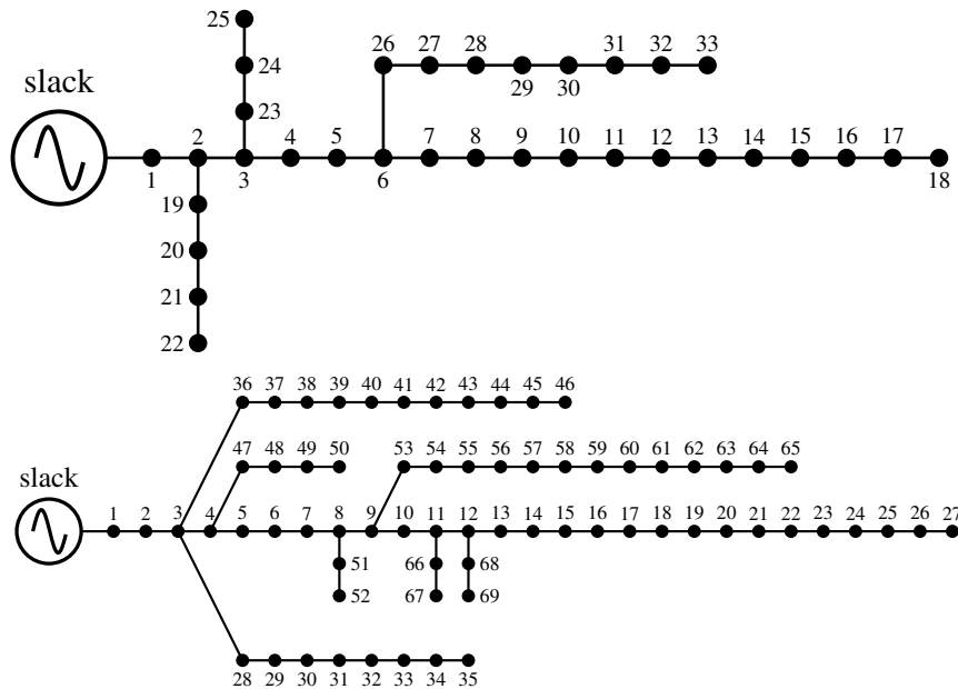
Figure 3. Single-line diagrams of the 33- and 69-bus distribution systems
