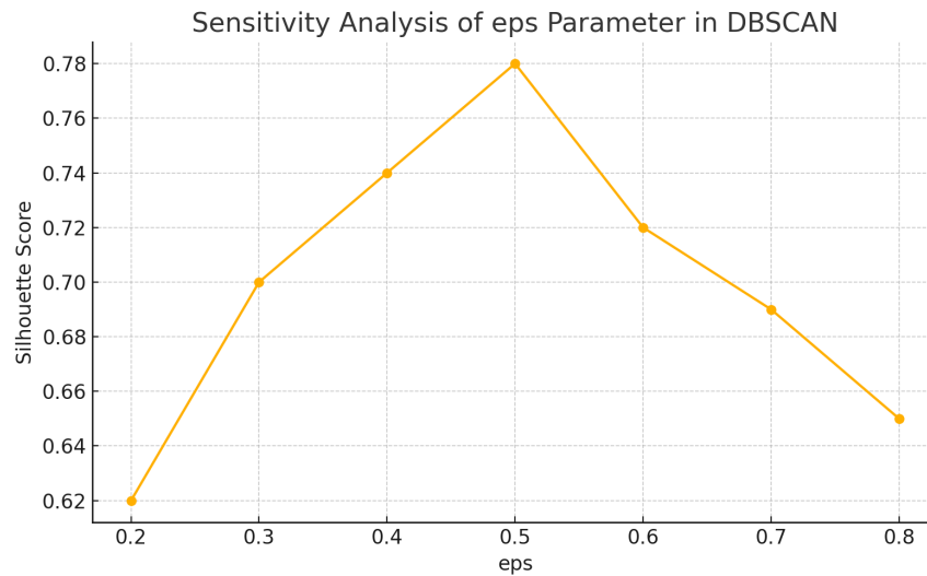
Figure 14. Silhouette Score obtained for different values of \text{eps} , with fixed \text{min\_samples} . The optimal value was \text{eps} = 0.5 .
