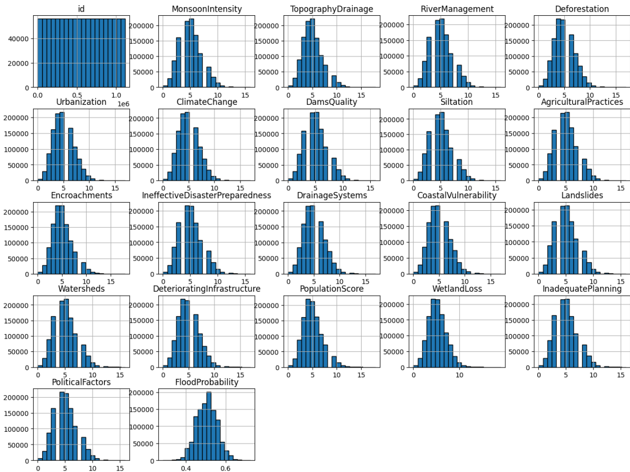
Figure 2. Feature distribution of the Flood Prediction Dataset, showing variability and statistical patterns across 22 predictors
