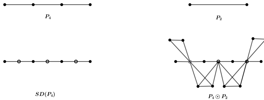
Figure 7. Subdivision - vertex neighbourhood corona
