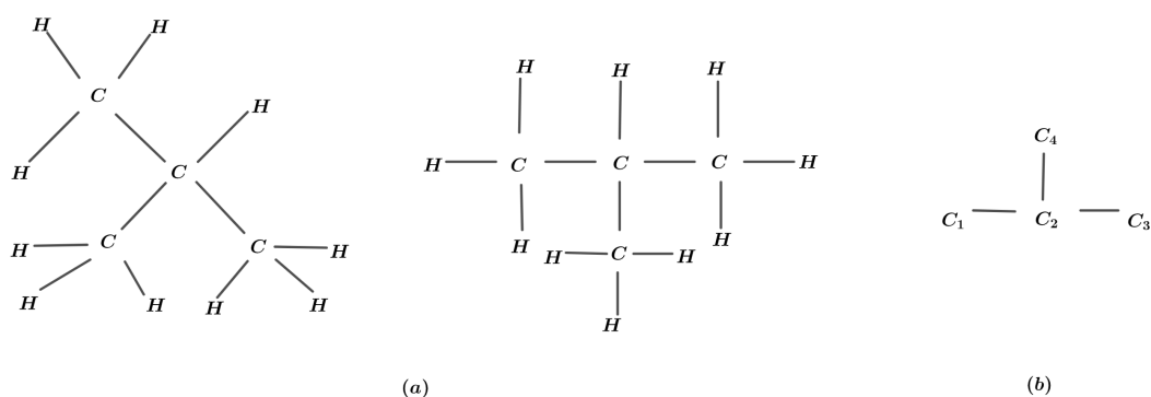
Figure 10. (a) - Isopentane [C_6H_{10}] and (b) Carbon Skeleton of C_6H_{10} as Graph H_3
