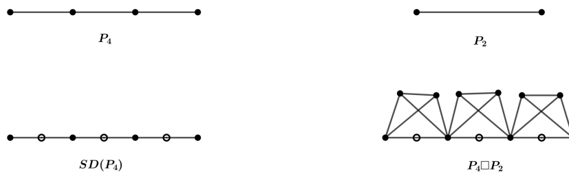
Figure 8. Subdivision - edge neighbourhood corona
