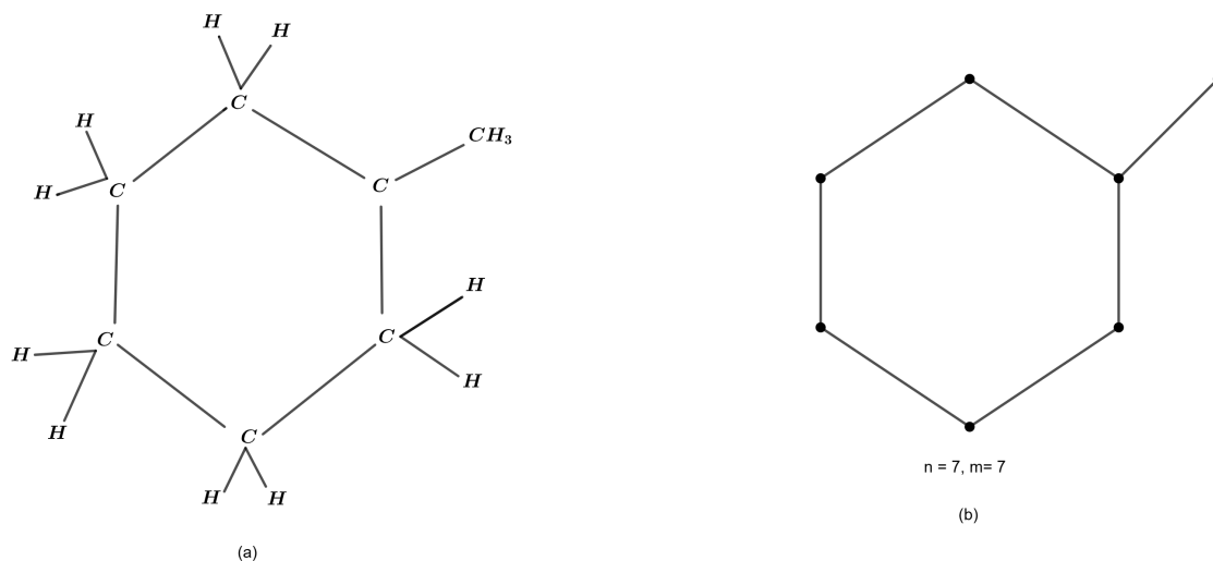
Figure 3. (a)- Ethylcyclohexane C_7H_{14} and (b)- Carbon skeleton C_7H_{14} as Graph H_2
