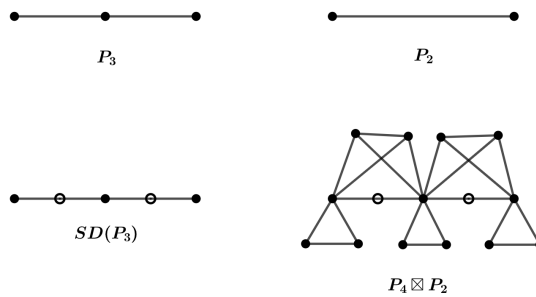
Figure 9. The Vertex-edge corona graph
